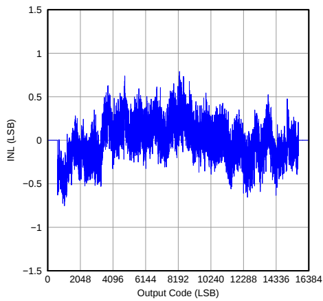
Figure 81. Integral Nonlinearity
