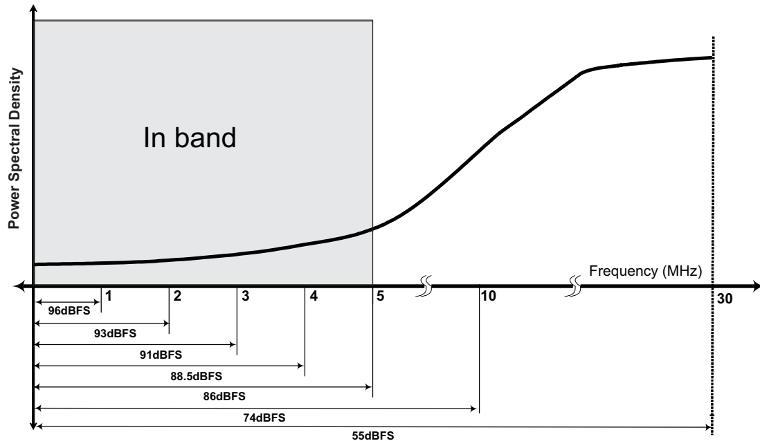
Figure 38. Typical Filter Bypass Mode Noise Spectral Density
