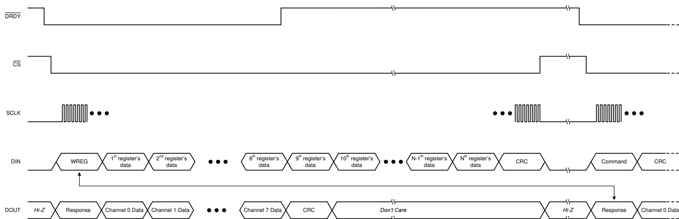
图 8-25. Writing Registers
