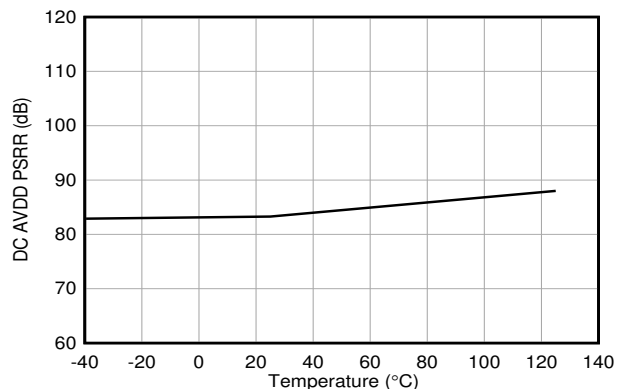
图 6-13. DC AVDD PSRR vs Temperature
