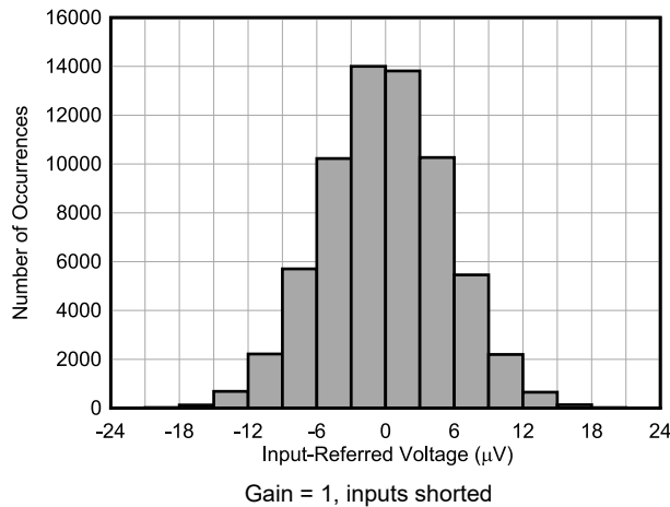
图 6-16. Single Device Noise Histogram at 4 kSPS
