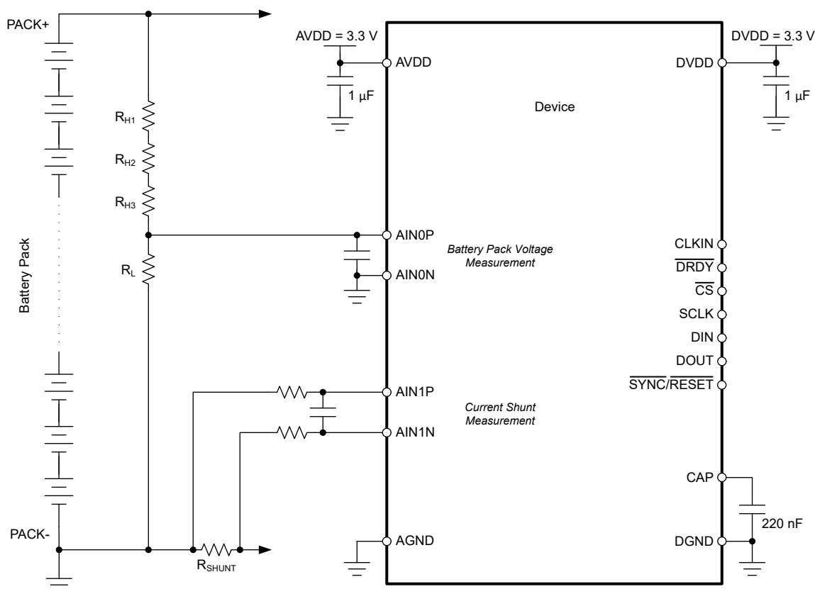
图 9-4. ADS131M06-Q1 in a Typical Battery Management System Application
