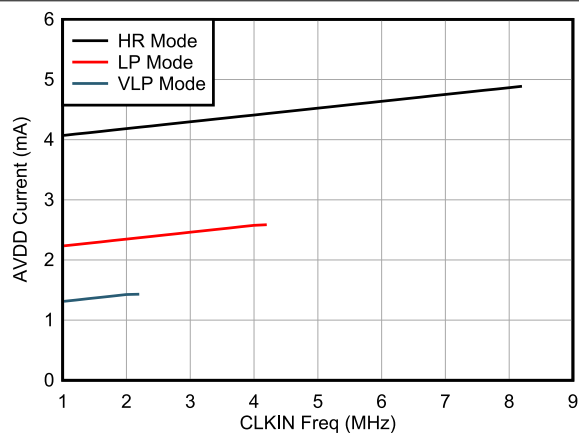
图 6-26. AVDD Current vs CLKIN Frequency
