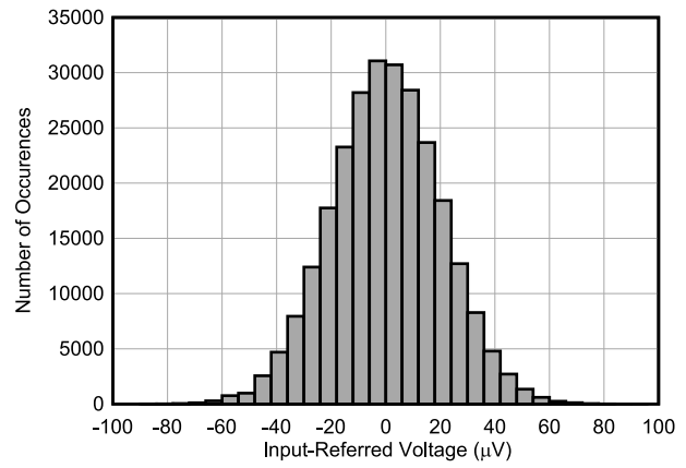
图 6-17. Single Device Noise Histogram at 32 kSPS
