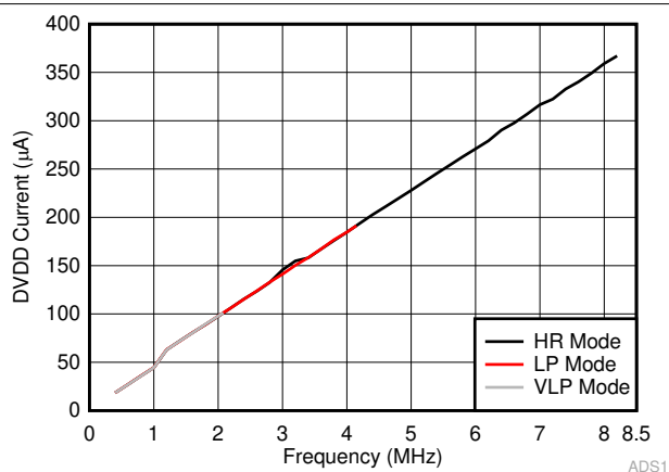
图 6-29. DVDD Current vs CLKIN Frequency
