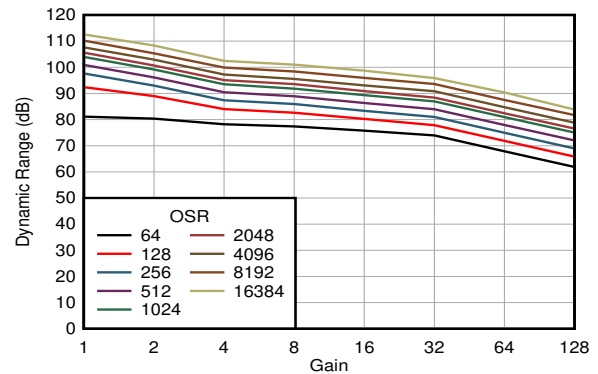
图 6-23. Dynamic Range vs Gain
