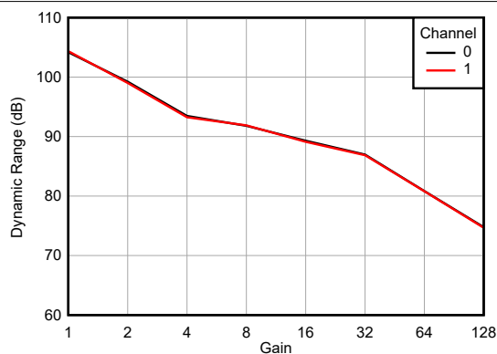
图 6-22. Dynamic Range vs Gain
