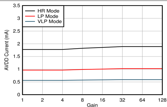
图 6-27. AVDD Current vs Gain
