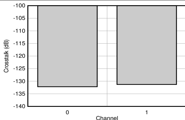
图 6-24. Crosstalk vs Channel
