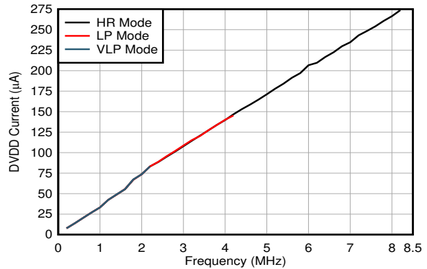
图 6-31. DVDD Current vs CLKIN Frequency
