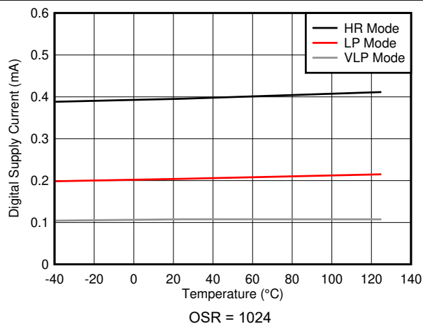
OSR = 1024 图 6-14. Digital Supply Current vs Temperature
