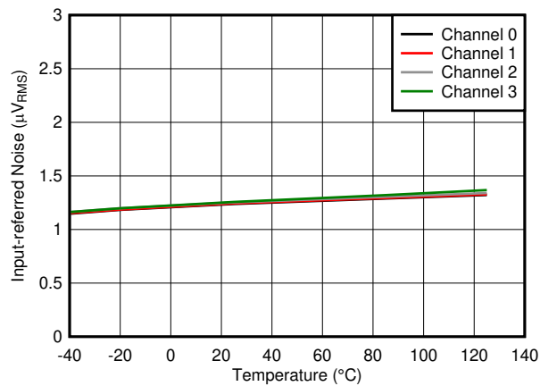
Gain = 8, global-chop mode disabled 图 6-10. Input-referred Noise vs Temperature
