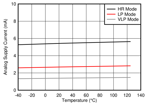
Gain = 1, OSR = 1024, all four ADC channels enabled 图 6-12. Analog Supply Current vs Temperature
