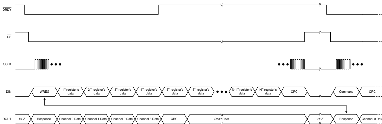
图 8-23. Writing Registers
