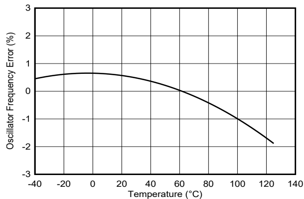
图 6-11. Oscillator Frequency Error vs Temperature
