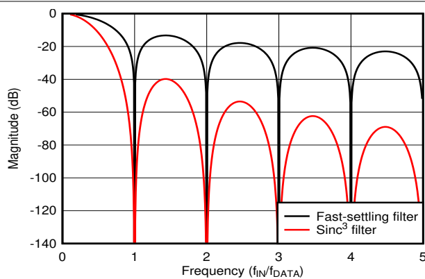
图 8-5. Fast-Settling and Sinc 3 Digital Filter Response
