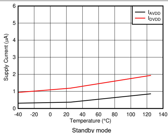
Standby mode 图 6-15. Supply Current vs Temperature
