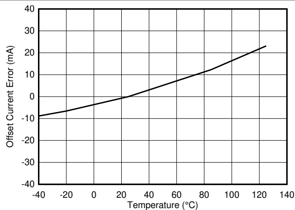
图 9-5. Offset Current Error vs Temperature
