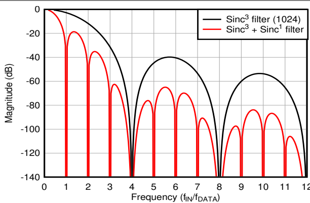
图 8-7. Digital Filter Response for OSR = 1024 and OSR = 4096
