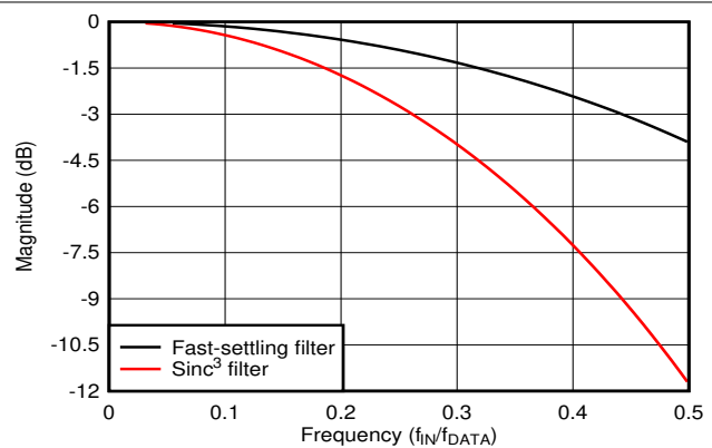
图 8-6. Fast-Settling and Sinc 3 Digital Filter Response, Pass-Band Detail
