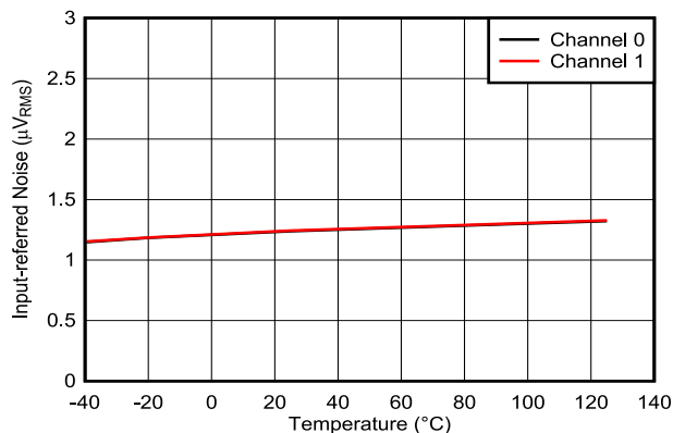
Gain = 8, global-chop mode disabled 图 6-10. Input-referred Noise vs Temperature
