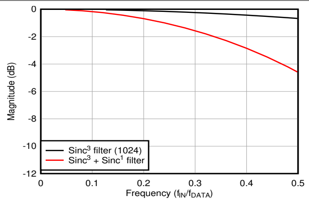
图 8-8. Digital Filter Response for OSR = 1024 and OSR = 4096, Pass-Band Detail
