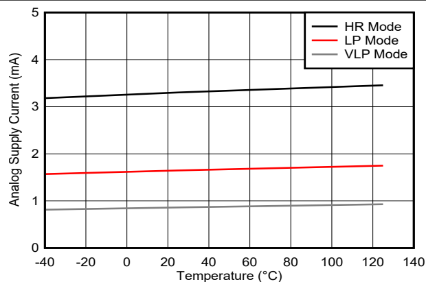
Gain = 8, OSR = 1024, all two ADC channels enabled 图 6-13. Analog Supply Current vs Temperature
