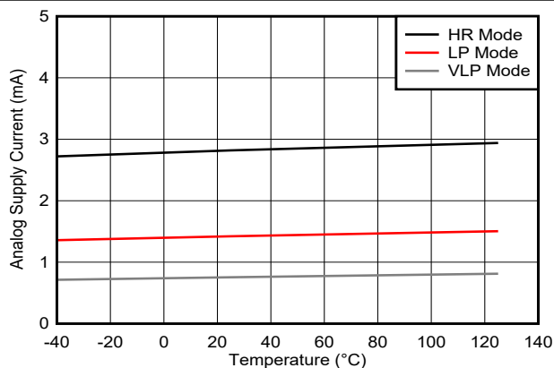
Gain = 1, OSR = 1024, all two ADC channels enabled 图 6-12. Analog Supply Current vs Temperature
