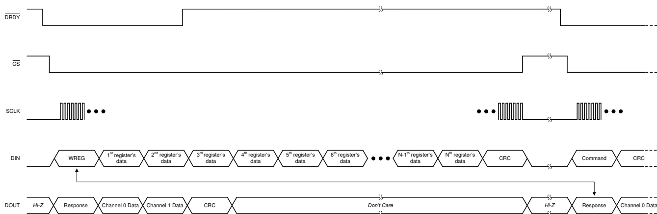
图 8-23. Writing Registers
