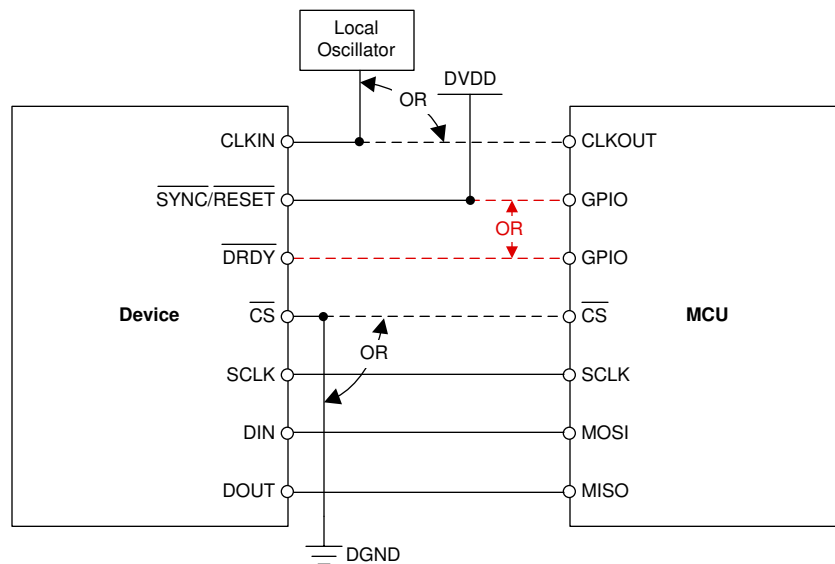
图 9-2. Minimum Connections Required to Operate the ADS130B02-Q1
