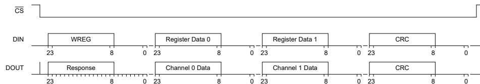
图 8-15. SPI Frame using 24-bit, zero-padded Word Size
