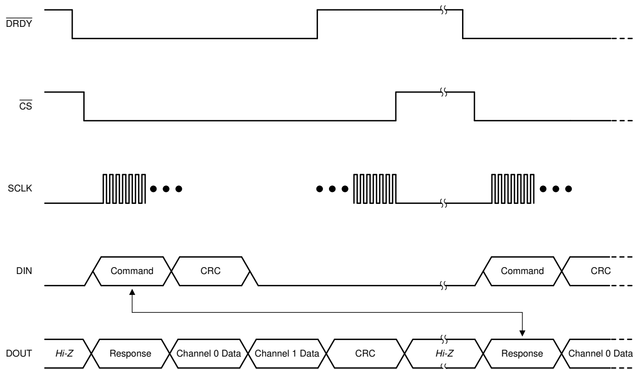
图 8-13. Typical Communication Frame
