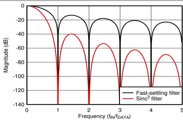
图 8-5. Fast-Settling and Sinc 3 Digital Filter Response
