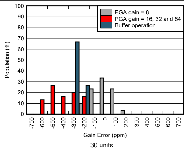
图 6-42. Gain Error Distribution
