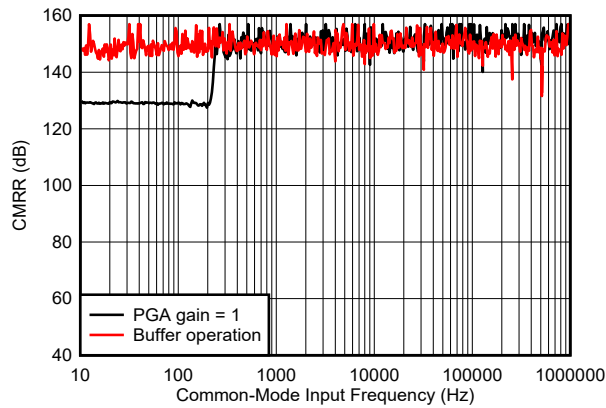
图 6-59. CMRR vs Common-Mode Input Frequency
