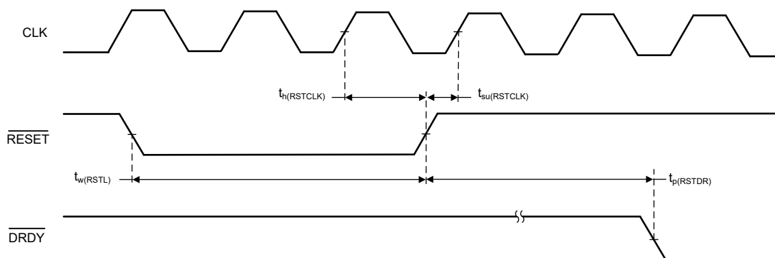
图 6-5. RESET Timing Requirements and Switching Characteristics
