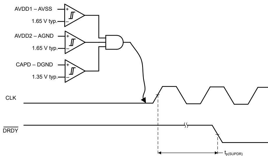
图 6-8. Power-Up Switching Characteristics
