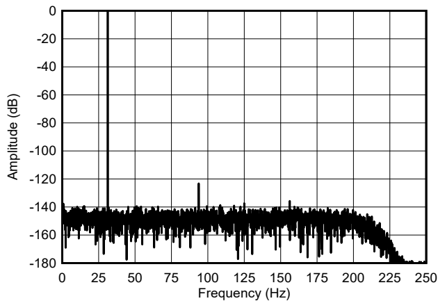
图 6-31. Low-Power Mode FFT Spectrum
