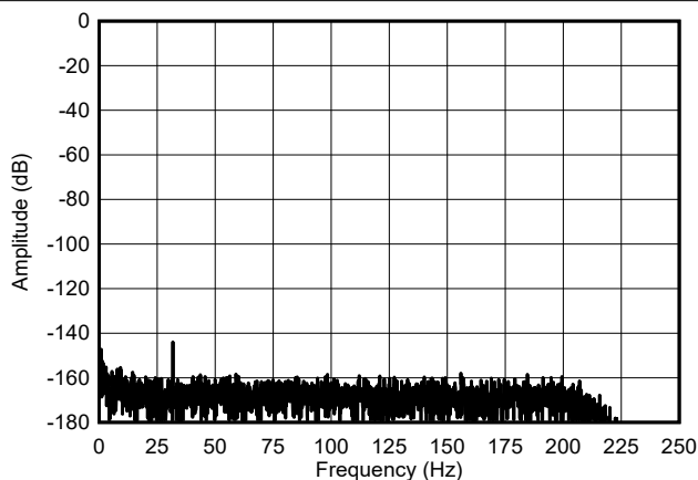
图 6-33. Low-Power Mode FFT Spectrum
