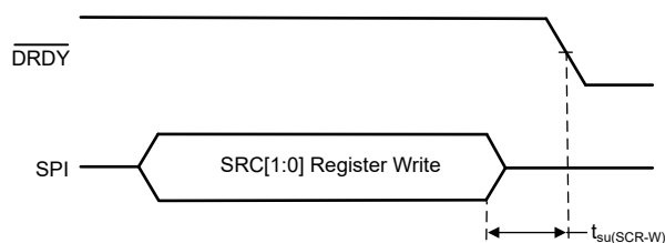
图 6-7. Sample Rate Converter Register-Write Timing Requirements
