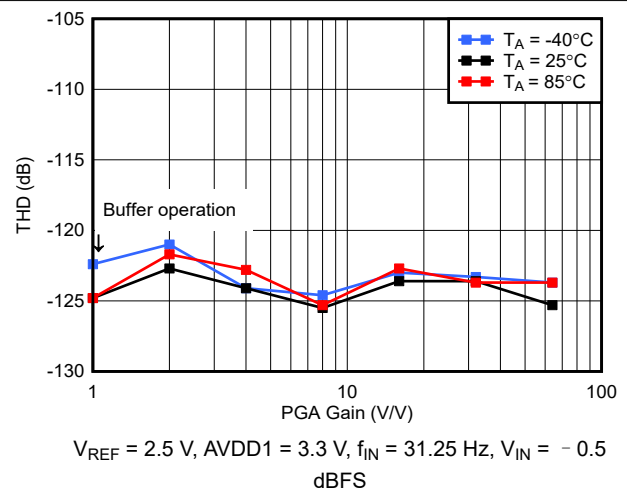
图 6-48. Low-Power Mode THD vs PGA Gain
