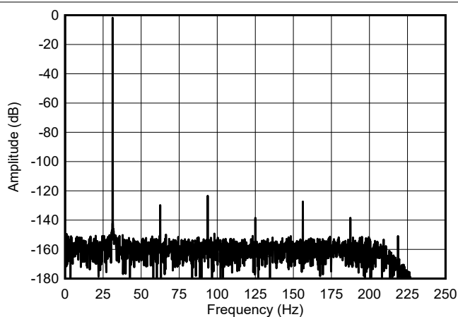
图 6-11. High-Power Mode FFT Spectrum
