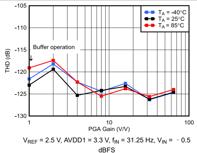
图 6-46. High-Power Mode THD vs PGA Gain
