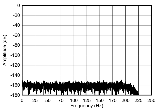
图 6-10. High-Power Mode FFT Spectrum
