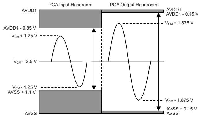
图 8-5. PGA Headroom (AVDD1 = 5 V, PGA Gain = 1)
