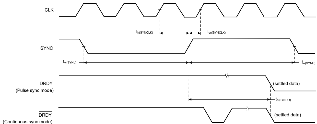
图 6-4. SYNC Timing Requirements and Switching Characteristics
