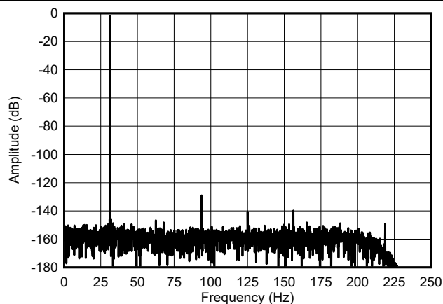
图 6-28. Low-Power Mode FFT Spectrum
