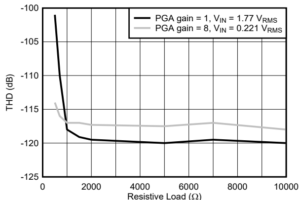
图 8-3. THD Performance vs R_{LOAD}
