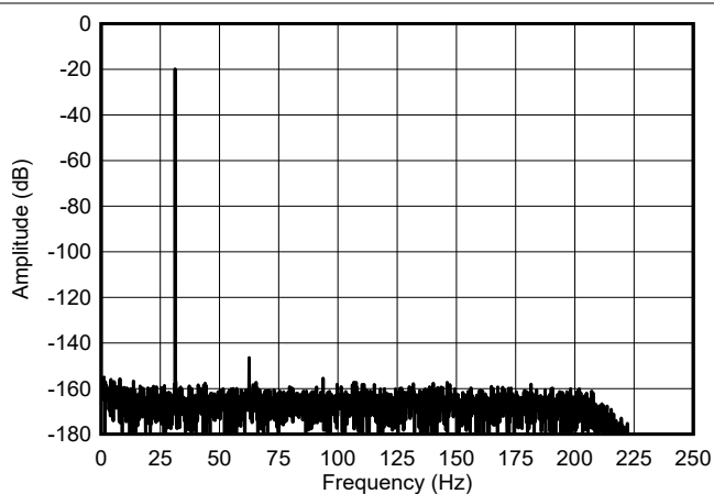
图 6-12. High-Power Mode FFT Spectrum
