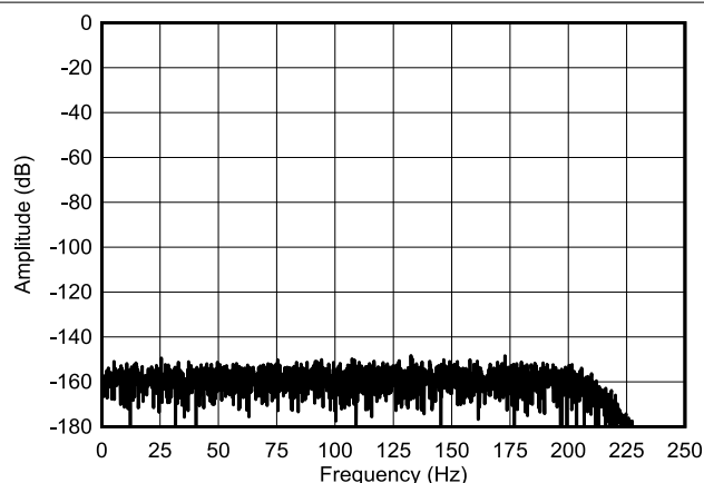
图 6-26. Mid-Power Mode FFT Spectrum
