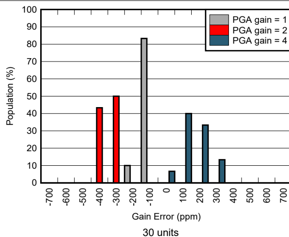
图 6-41. Gain Error Distribution
