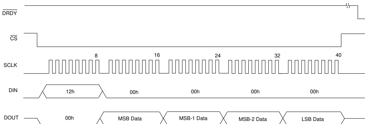
图 8-25. Read Conversion Data by Command
