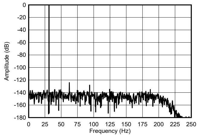
图 6-16. High-Power Mode FFT Spectrum
