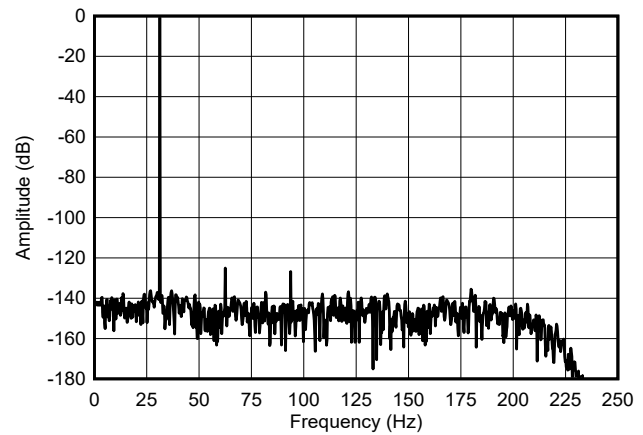
图 6-32. Low-Power Mode FFT Spectrum
