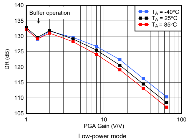
图 6-38. Dynamic Range vs PGA Gain
