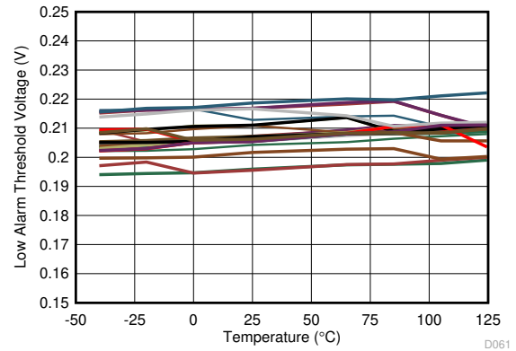
图 7-47. ADC1 Absolute Low Alarm Threshold vs Temperature
