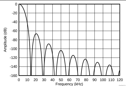
图 62. Frequency Response (14400 SPS)
