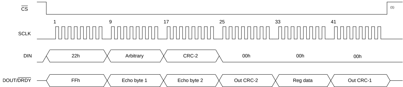
图 78. Register Read Operation (address = 02h, CRC Mode Enabled)
