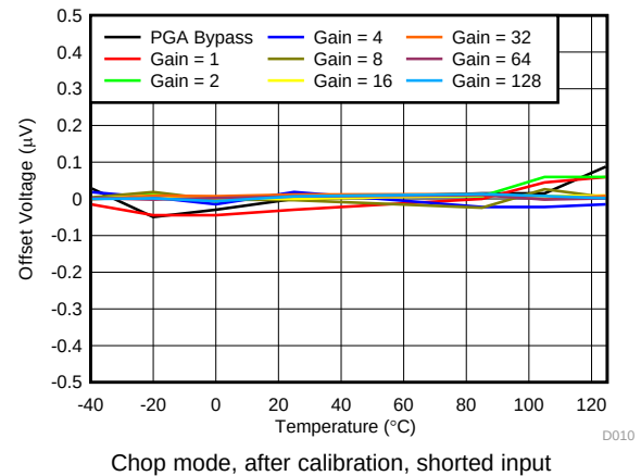
图 10. Offset Voltage vs Temperature
