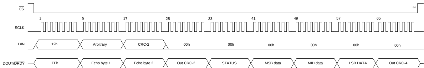
图 77. Conversion Data Read Operation (STATUS Byte and CRC Mode Enabled)
