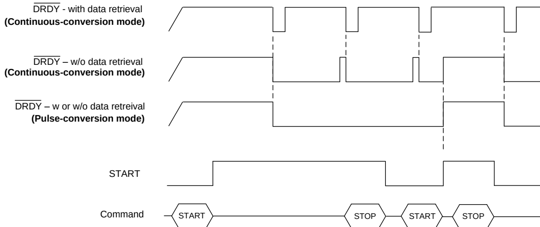
图 75. \overline{\text{DRDY}} Operation
