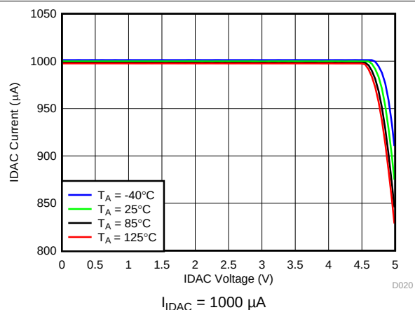
图 44. IDAC Current vs IDAC Voltage
