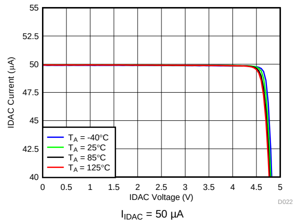
图 42. IDAC Current vs IDAC Voltage
