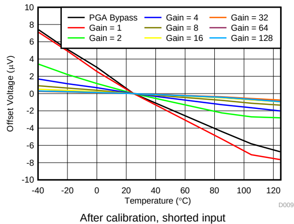
图 9. Offset Voltage vs Temperature
