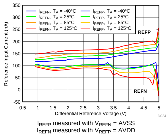
图 32. Reference Input Current vs Reference Voltage
