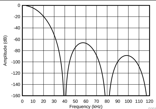
图 61. Frequency Response (40000 SPS)
