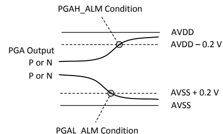
图 52. PGA Monitor Thresholds
