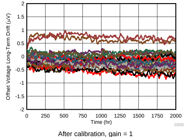
图 14. Offset Voltage Long-Term Drift
