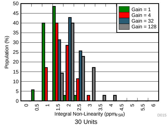
图 28. Integral Nonlinearity Distribution
