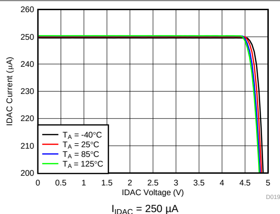
图 43. IDAC Current vs IDAC Voltage
