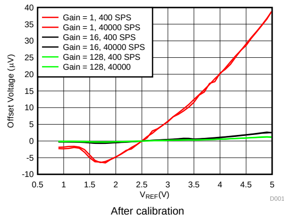
图 13. Offset Voltage vs Reference Voltage
