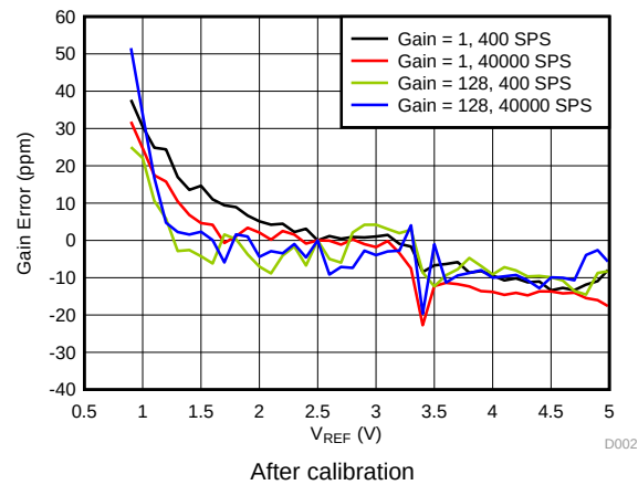
图 17. Gain Error vs Reference Voltage
