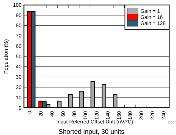
图 11. Offset Voltage Drift Distribution
