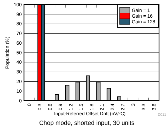
图 12. Offset Voltage Drift Distribution
