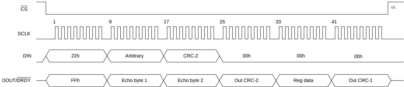
图 39. Register Read Operation (address = 02h, CRC Mode Enabled)
