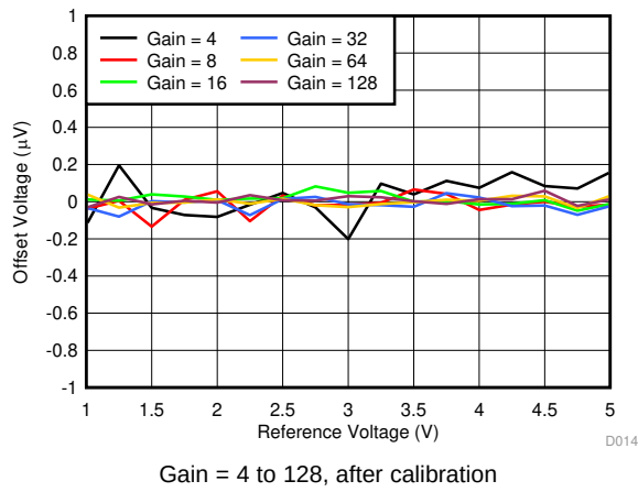
图 30. Offset Voltage vs Reference Voltage
