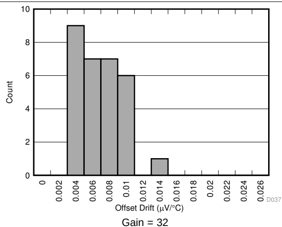
图 25. Offset Voltage Drift Distribution
