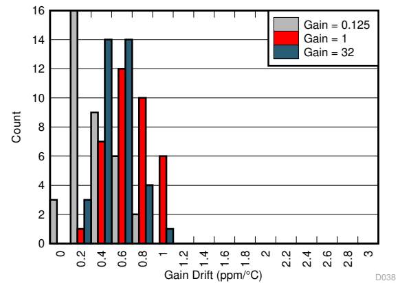
图 7-19. Gain Drift Distribution
