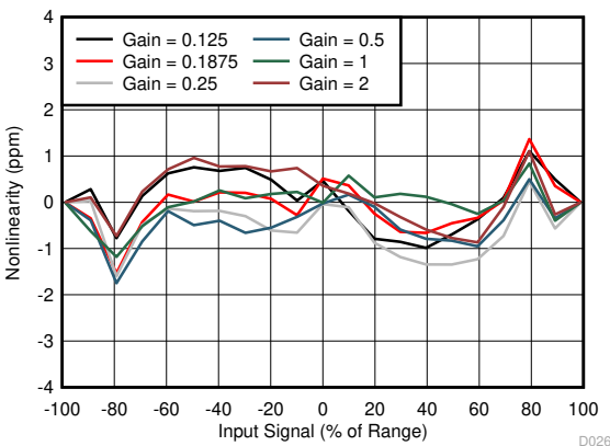
图 7-10. Nonlinearity vs Input Signal
