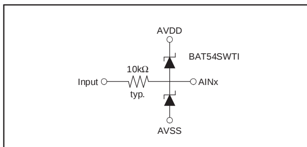
Figure 62. Input Overload Protection
