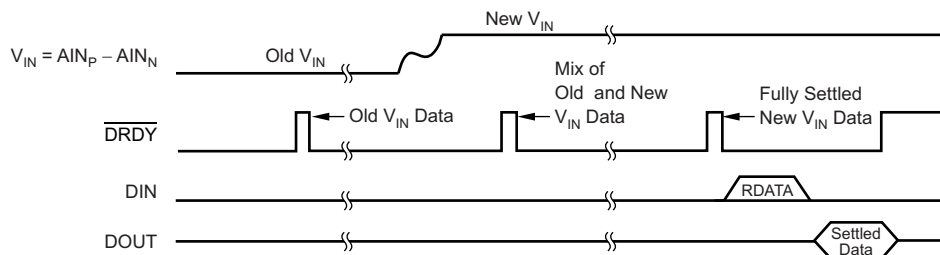
Figure 38. Step Change on V_{\text{IN}} While Continuously Converting for Data Rates \leq 3750 SPS
