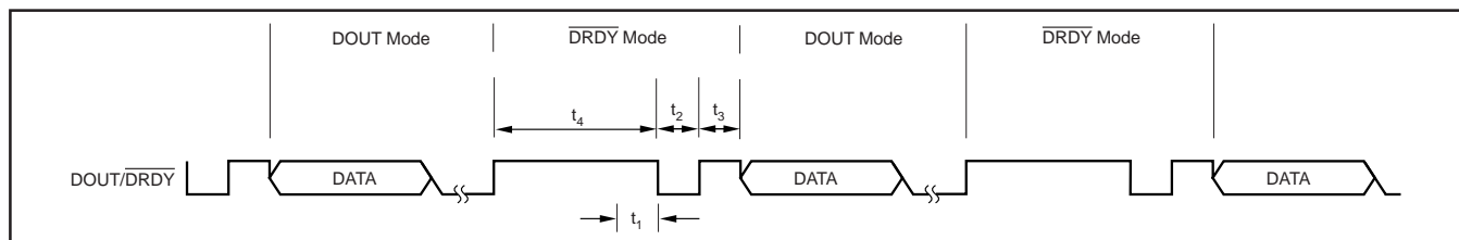
FIGURE 12. DOUT/DRDY Partitioning.
