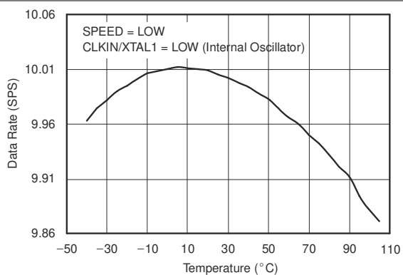
图 5-25. Data Rate vs Temperature
