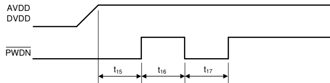
图 7-15. Power-Up Timing Sequence
