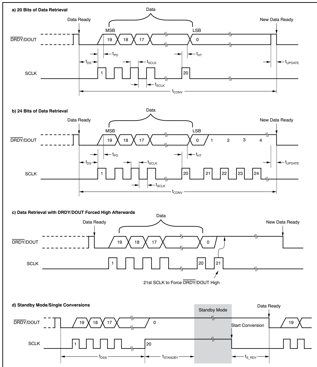
Figure 34. Summary of Data Retrieval Waveforms
