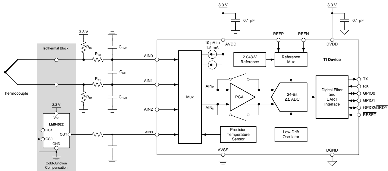
图 76. Thermocouple Measurement
