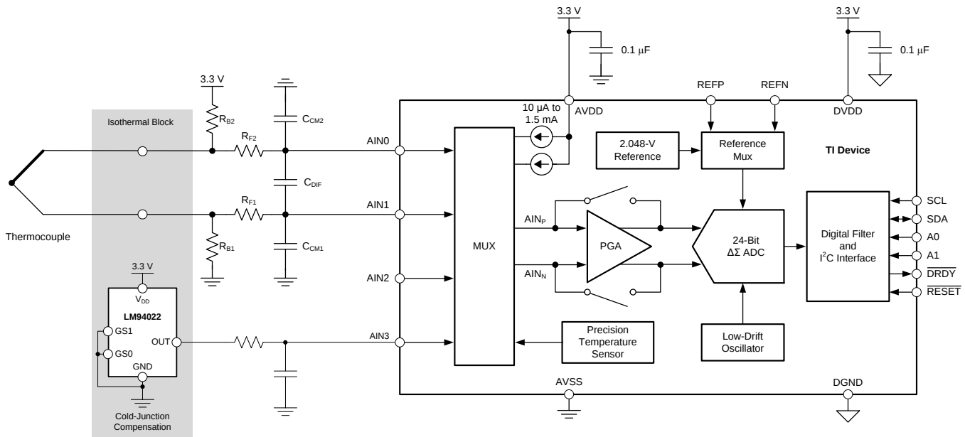
图 71. Thermocouple Measurement
