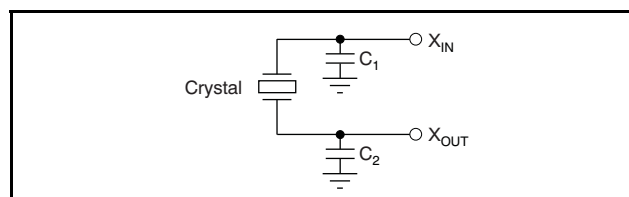
Figure 26. Crystal Connection
