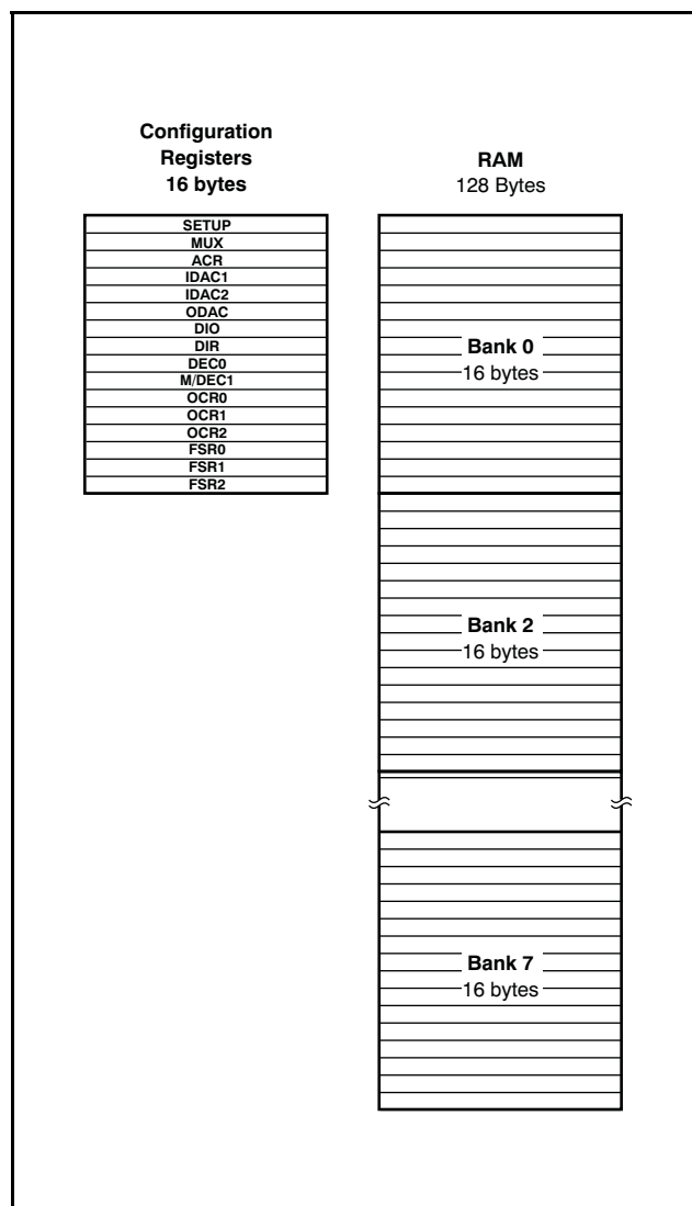
Figure 29. Memory Organization
