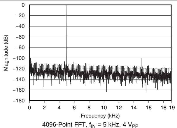
Figure 19. Frequency Spectrum
