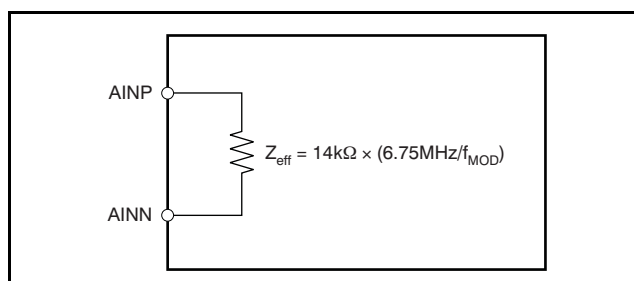
Figure 9. Effective Input Impedances
