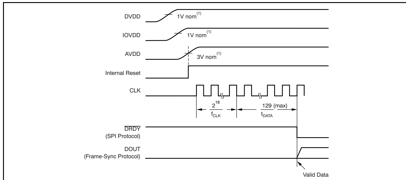
Figure 24. Start-Up Sequence
