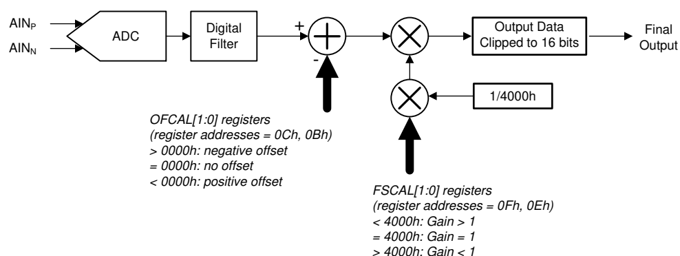
图 66. ADC Calibration Block Diagram
