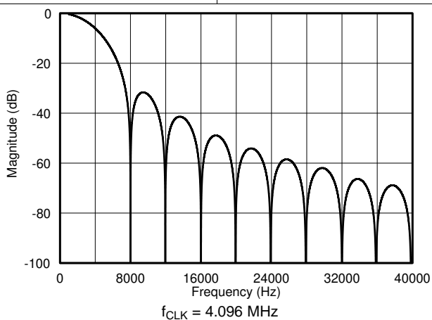
图 61. Digital Filter Frequency Response, Data Rate = 4 kSPS
