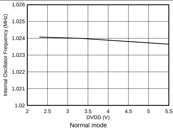
图 30. Internal Oscillator Frequency vs DVDD
