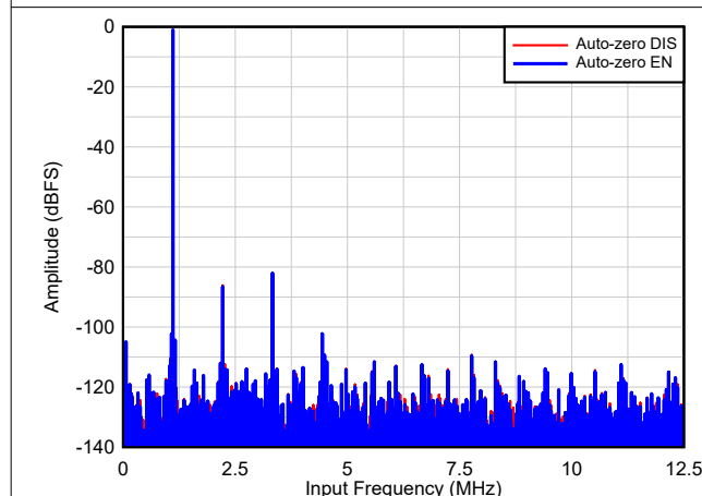
图 7-10. F_S = 25\text{MSPS} , F_{IN} = 1.1\text{MHz}
