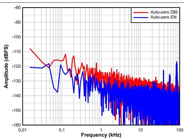
图 7-13. F_S = 65\text{MSPS} , F_{IN} = 5\text{MHz}
