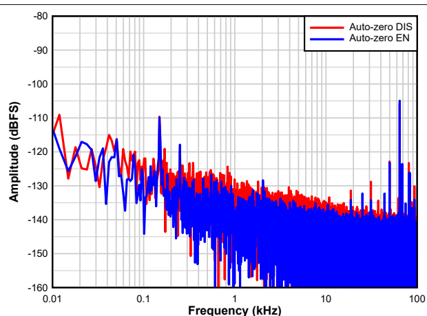
图 7-11. F_S = 25\text{MSPS} , F_{IN} = 1.1\text{MHz}
