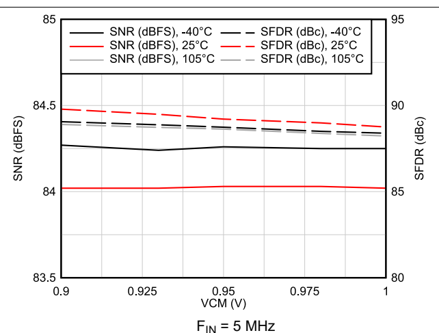
图 6-57. AC Performance vs VCM vs Temperature
