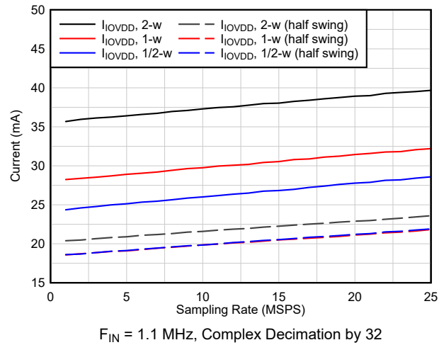
图 6-39. I_{IOVDD} Current vs Interface
