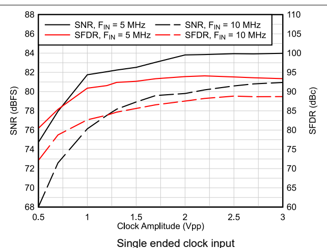
图 6-55. AC Performance vs Clock Amplitude
