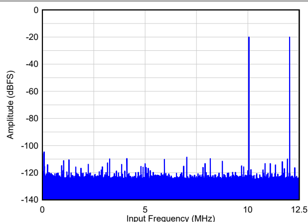
A_{IN} = -20\text{ dBFS/line} , \text{IMD3} = 88\text{ dBc} 图 6-26. Two Tone FFT at F_{IN} = 10/12\text{ MHz}
