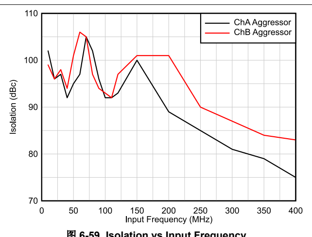
图 6-59. Isolation vs Input Frequency
