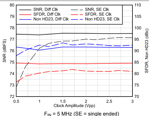
图 6-18. AC Performance vs Clock Amplitude
