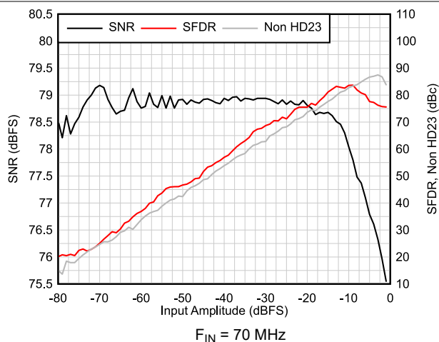
图 6-16. AC Performance vs Input Amplitude
