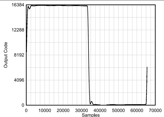
Pulse Input = 1 MHz 图 6-26. Pulse Response
