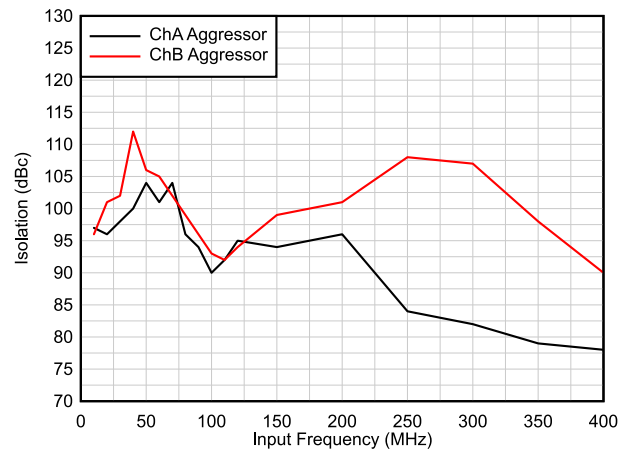
图 6-22. Isolation vs Input Frequency
