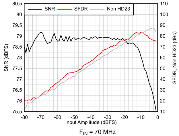
图 6-16. AC Performance vs Input Amplitude
