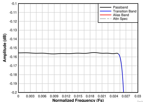
图 8-28. Decimation by 16 complex passband ripple response
