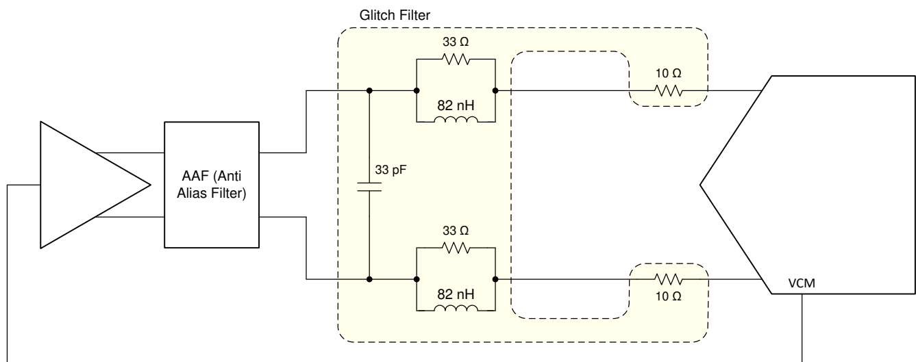
图 8-7. DC-Coupling: DC bias provided by FDA (glitch filter example for DC - 60 MHz)
