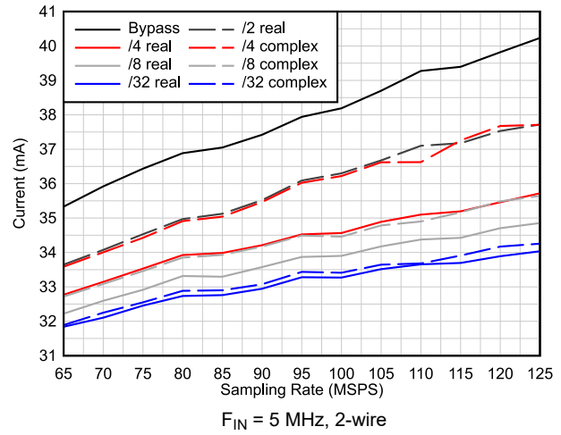
图 6-28. Power Consumption vs Decimation
