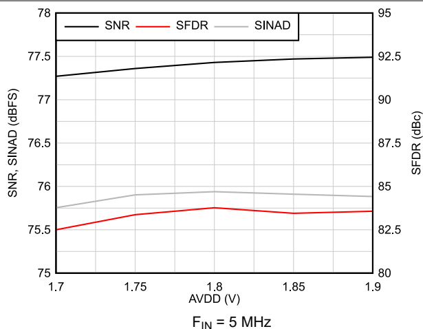
图 6-20. AC Performance vs AVDD
