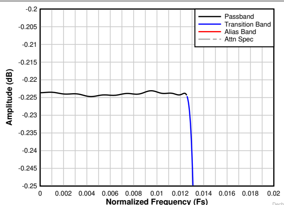
图 8-30. Decimation by 32 complex passband ripple response
