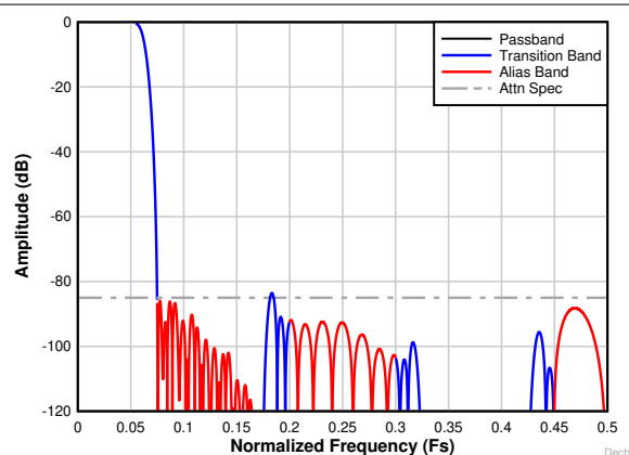
图 8-25. Decimation by 8 complex frequency response
