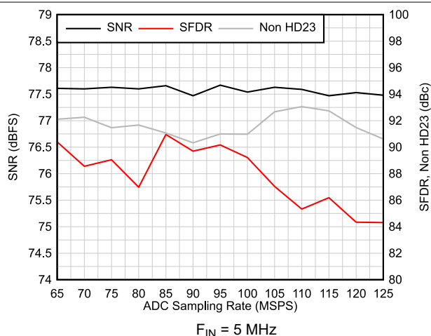
图 6-17. AC Performance vs Sampling Rate
