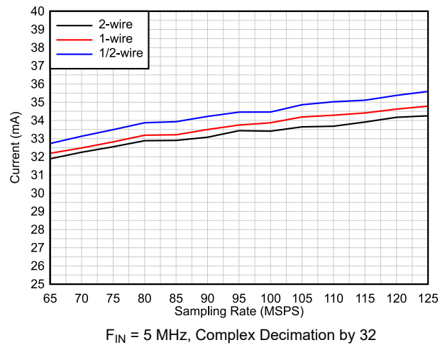
图 6-29. Power Consumption vs Output Interface
