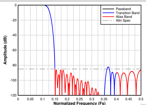
图 8-23. Decimation by 4 complex frequency response
