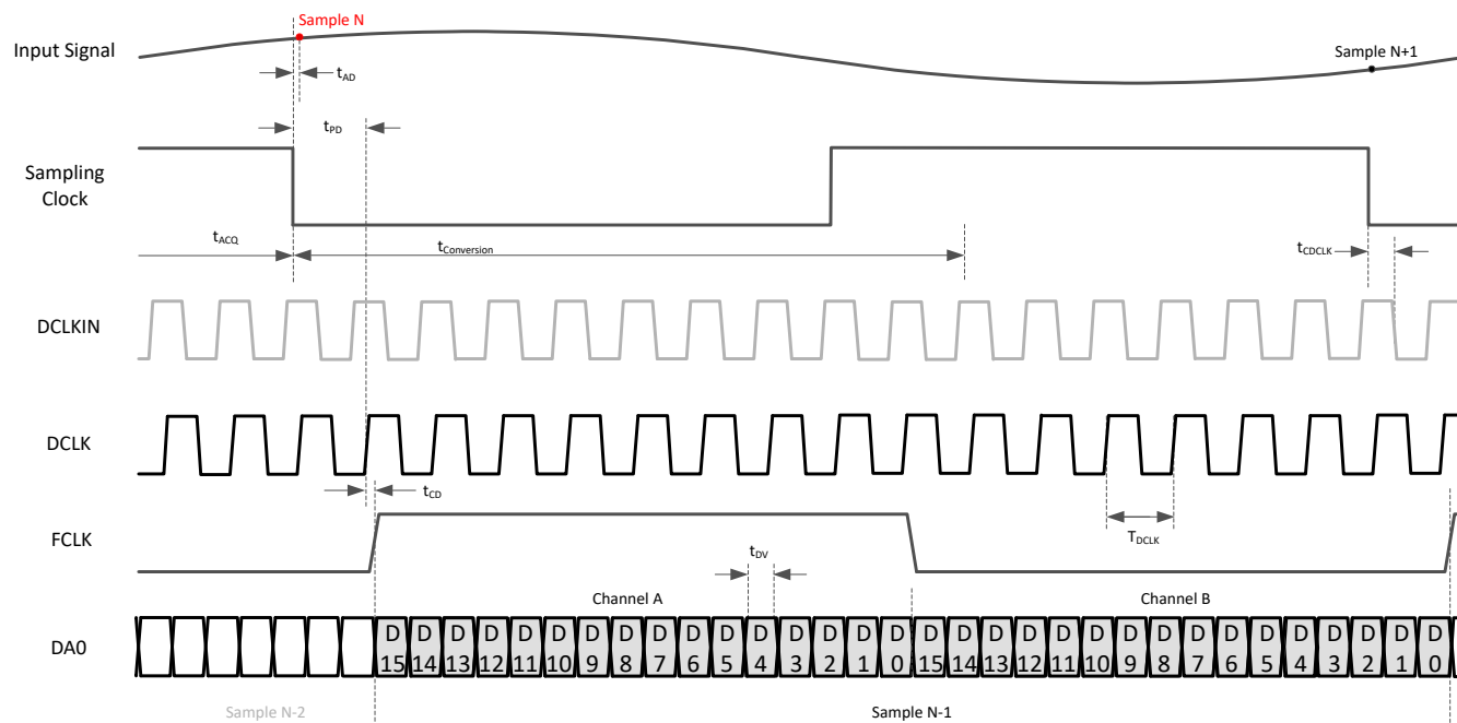
图 7-3. Timing diagram:1/2-wire SLVDS (default output bit mapper)
