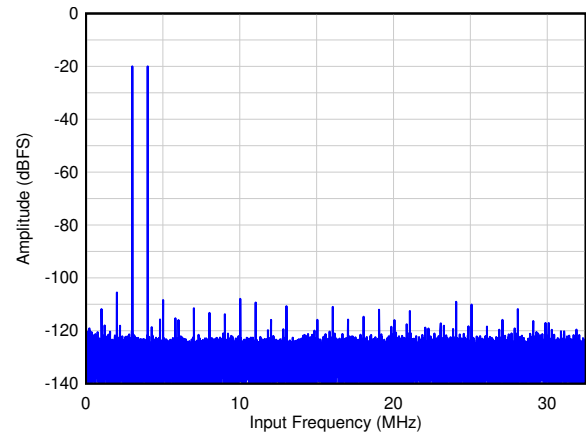
图 6-6. Two Tone FFT at F_{IN} = 3,4 MHz
