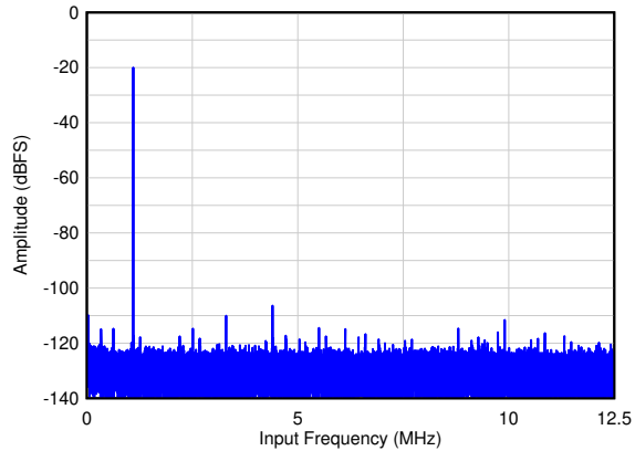
图 6-23. Single Tone FFT at F_{IN} = 1.1 MHz
