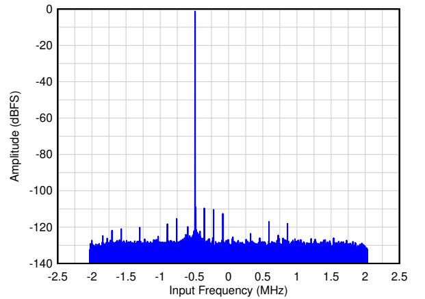
图 9-3. Single Tone FFT at F_{IN} = 5 MHz
