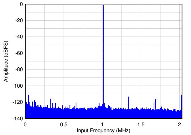
图 9-2. Single Tone FFT at F_{IN} = 1 MHz
