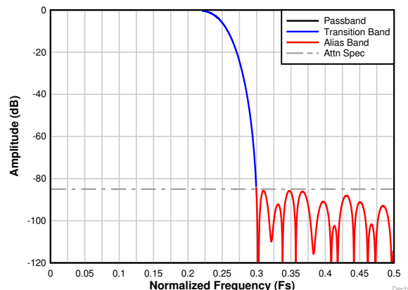
图 8-26. Decimation by 2 complex frequency response
