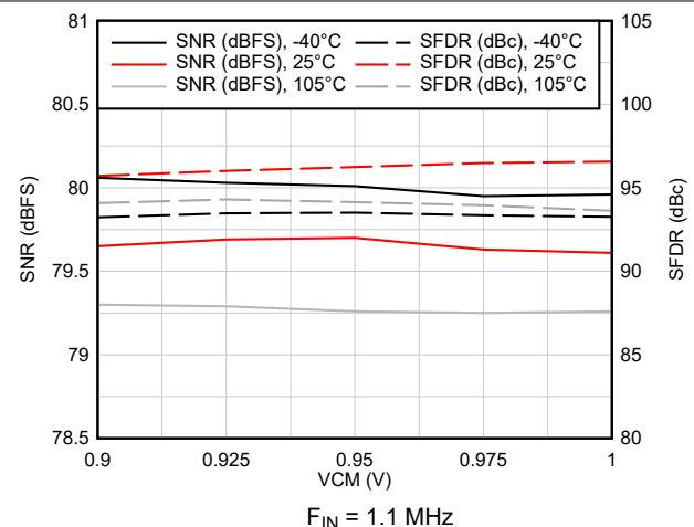
图 6-29. AC Performance vs VCM vs Temperature
