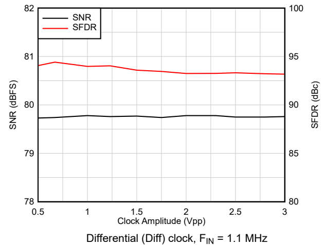
图 6-27. AC Performance vs Clock Amplitude
