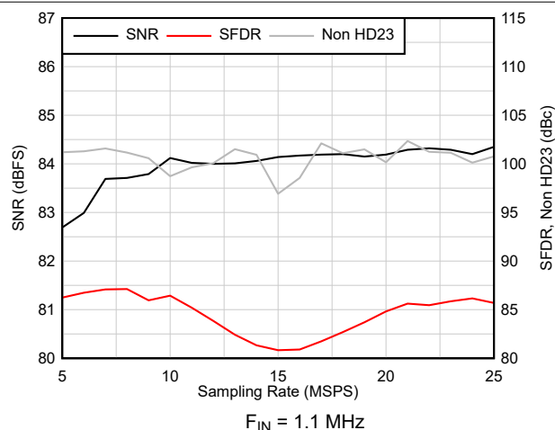
F_{IN} = 1.1\text{ MHz} 图 6-30. AC Performance vs Sampling Rate
