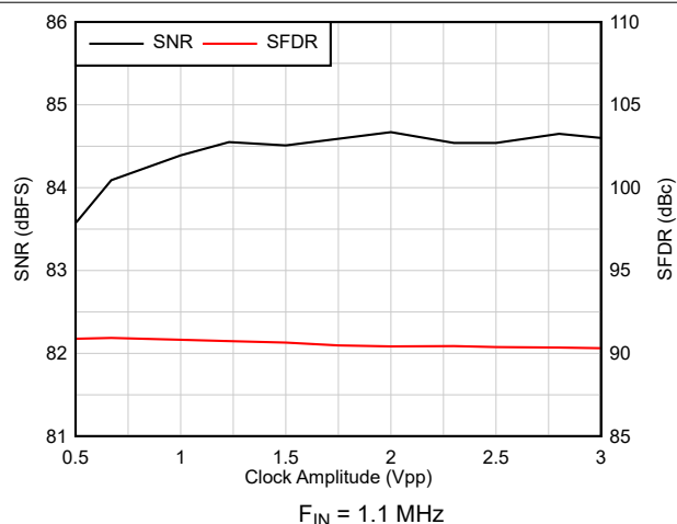
F_{IN} = 1.1\text{ MHz} 图 6-31. AC Performance vs Clock Amplitude
