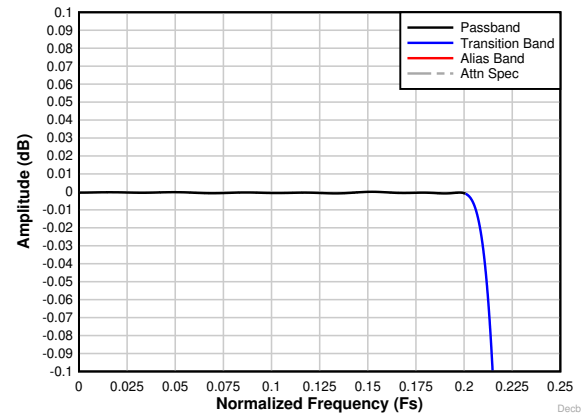
图 8-29. Decimation by 2 complex passband ripple response
