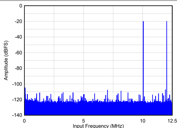
A_{IN} = -20 dBFS/tone, IMD3 = 88 dBc 图 6-26. Two Tone FFT at F_{IN} = 10/12\text{ MHz}
