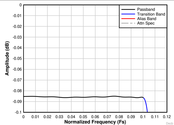
图 8-31. Decimation by 4 complex passband ripple response
