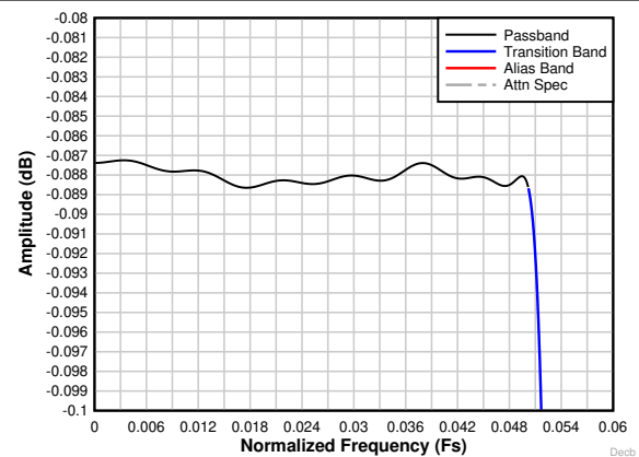
图 8-33. Decimation by 8 complex passband ripple response
