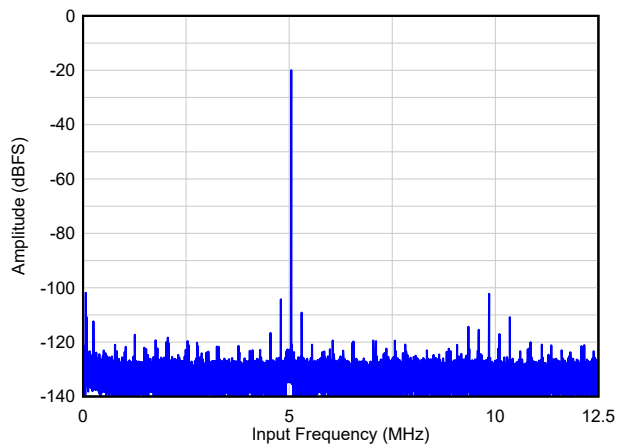
图 6-20. Single Tone FFT at F_{IN} = 5 MHz, A_{IN} = -20 dBFS
