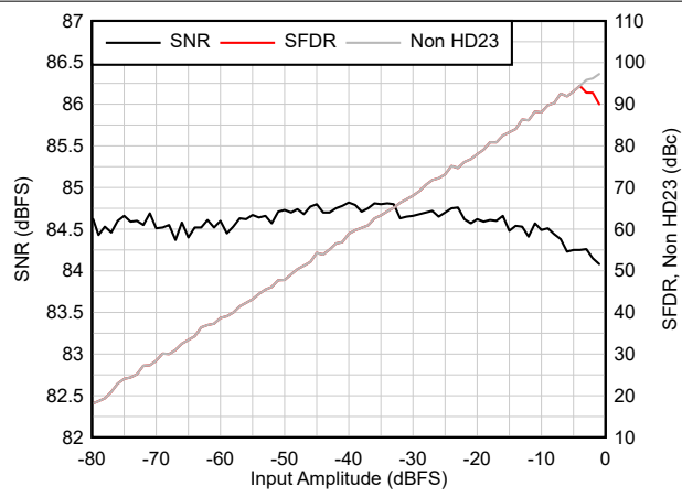
F_{IN} = 1.1\text{ MHz} 图 6-29. AC Performance vs Input Amplitude
