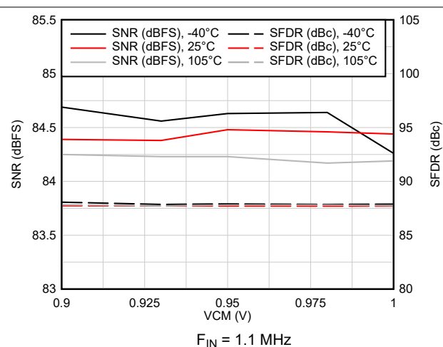
图 6-33. AC Performance vs VCM vs Temperature
