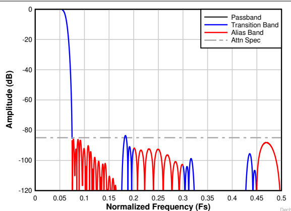
图 8-32. Decimation by 8 complex frequency response
