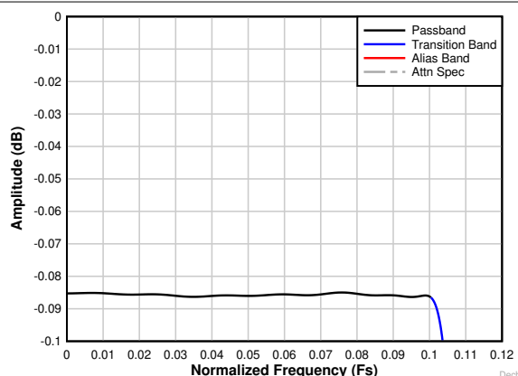
图 8-31. Decimation by 4 complex passband ripple response
