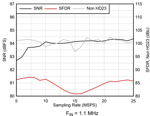
图 6-30. AC Performance vs Sampling Rate
