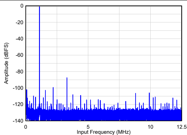
图 6-18. Single Tone FFT at F_{IN} = 1 MHz
