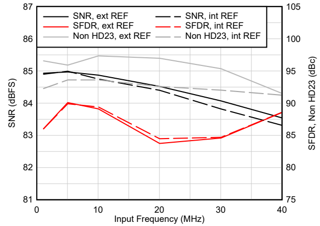
图 6-27. AC Performance vs Input Frequency
