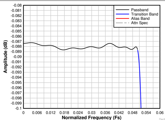
图 8-33. Decimation by 8 complex passband ripple response
