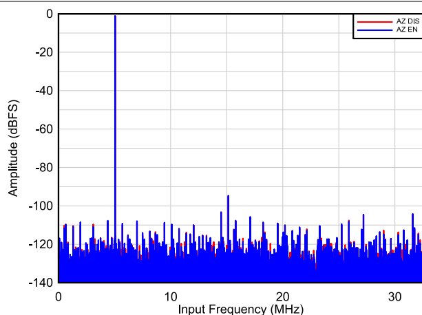
图 8-12. F_S = 65 MSPS, F_{IN} = 5 MHz
