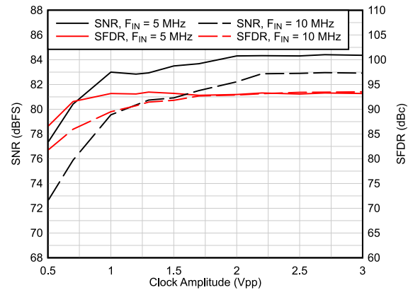
图 8-15. AC Performance vs Clock Amplitude (Single Ended Clock Input)
