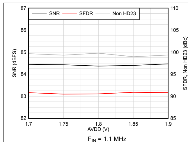
图 6-32. AC Performance vs AVDD
