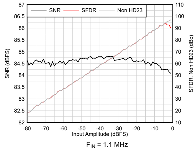
图 6-29. AC Performance vs Input Amplitude
