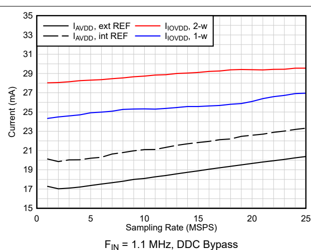
图 6-37. Current vs Sampling Rate
