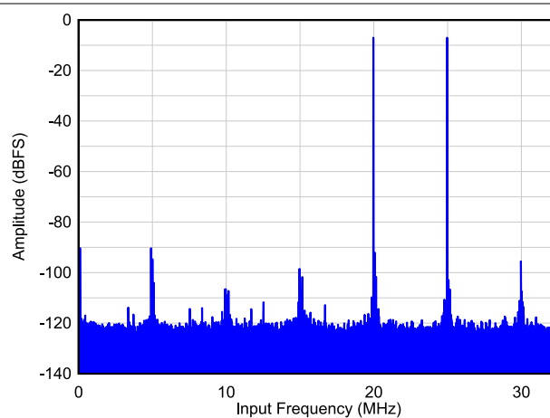
图 6-49. Two Tone FFT at F_{IN} = 40/45 MHz
