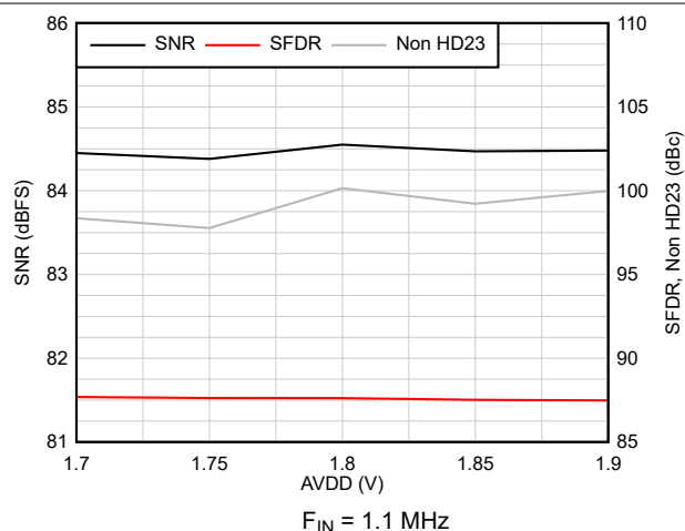
图 6-10. AC Performance vs AVDD
