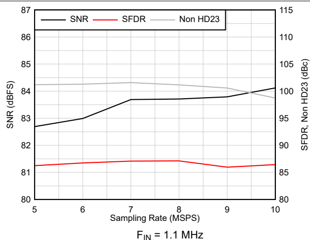
图 6-8. AC Performance vs Sampling Rate
