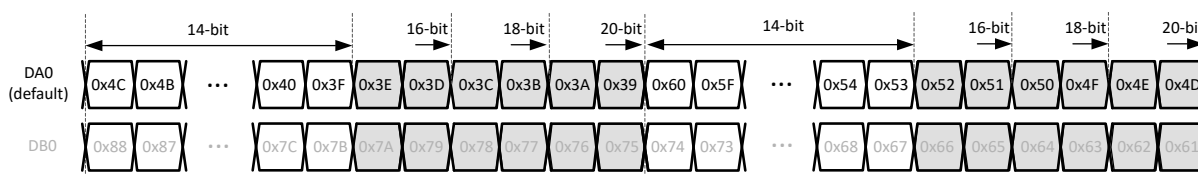
图 8-48. 1/2-wire output bit mapping
