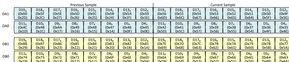
图 8-46. Example: 2-wire output bit mapping
