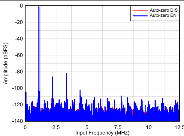
图 8-10. F_S = 25 MSPS, F_{IN} = 1.1 MHz
