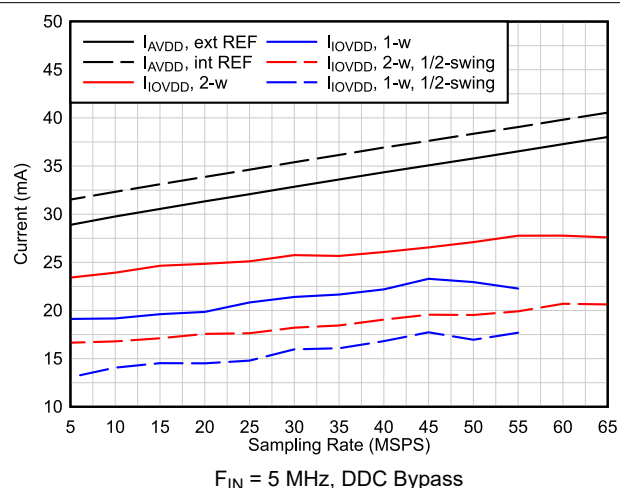
图 6-63. Current vs Sampling Rate
