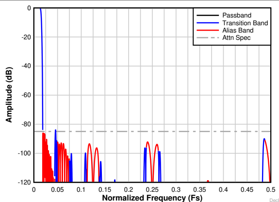
图 8-36. Decimation by 32 complex frequency response
