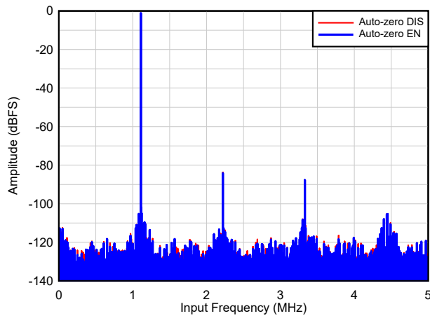
图 8-8. F_S = 10 MSPS, F_{IN} = 1.1 MHz
