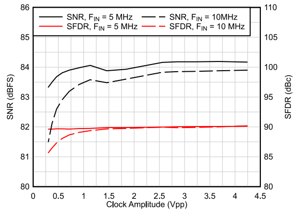
图 8-14. AC Performance vs Clock Amplitude (Differential Clock Input)
