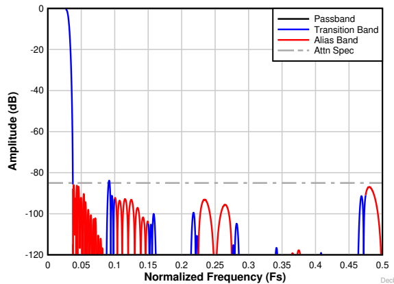
图 8-34. Decimation by 16 complex frequency response
