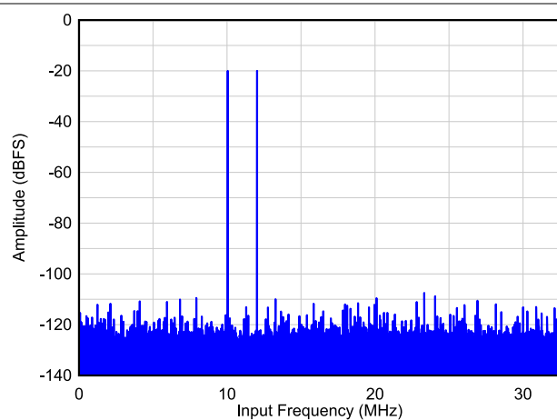
图 6-48. Two Tone FFT at F_{IN} = 10/12 MHz
