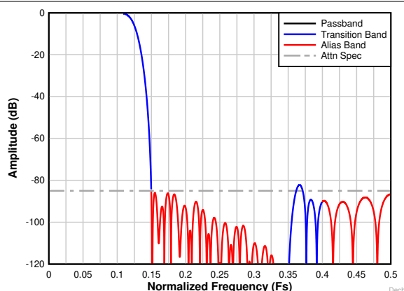
图 8-30. Decimation by 4 complex frequency response
