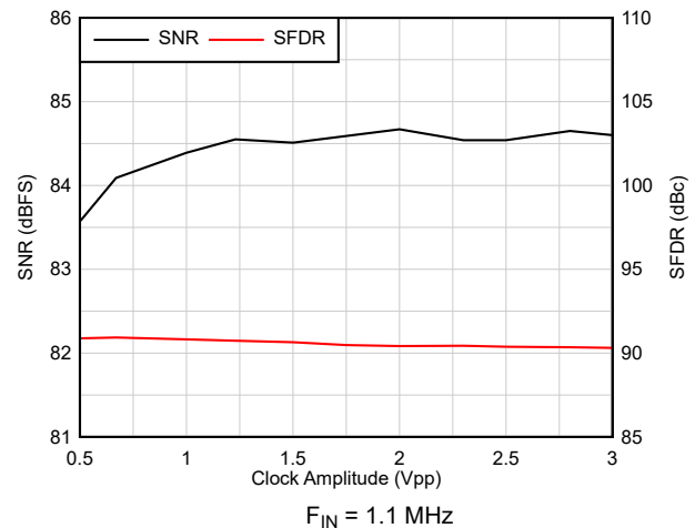
图 6-31. AC Performance vs Clock Amplitude
