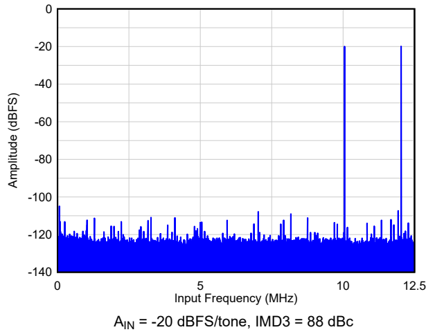
图 6-26. Two Tone FFT at F_{IN} = 10/12 MHz
