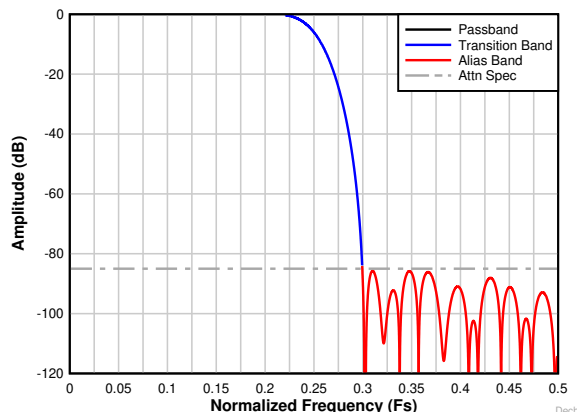
图 8-28. Decimation by 2 complex frequency response
