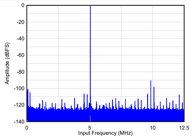
图 6-19. Single Tone FFT at F_{IN} = 5 MHz
