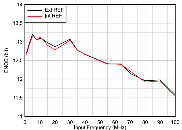
图 6-51. ENOB vs Input Frequency
