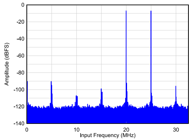
图 6-49. Two Tone FFT at F_{IN} = 40/45\text{ MHz}
