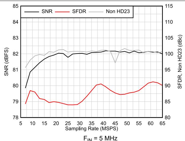
图 6-53. AC Performance vs Sampling Rate
