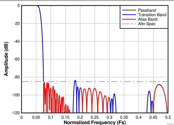
图 8-32. Decimation by 8 complex frequency response
