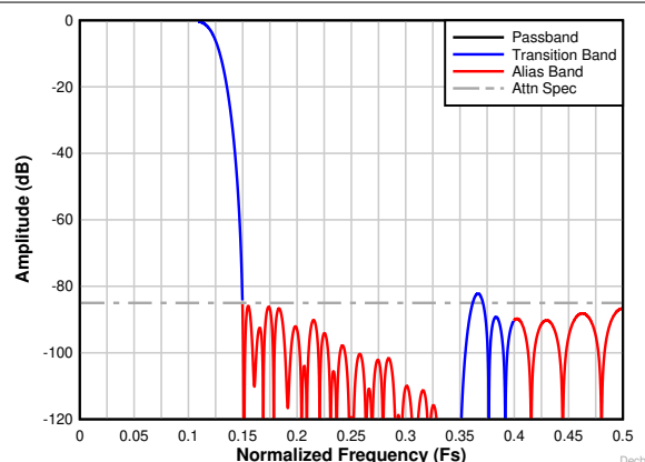
图 8-30. Decimation by 4 complex frequency response
