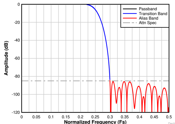
图 8-28. Decimation by 2 complex frequency response
