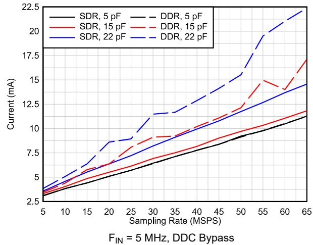
图 6-63. I_{OVDD} Current vs Output Load
