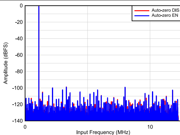
图 8-11. F_S = 25 \text{ MSPS} , F_{IN} = 1.1 \text{ MHz}
