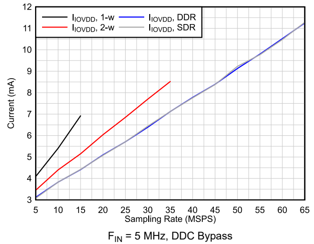
图 6-62. I_{OVDD} Current vs Output Interface
