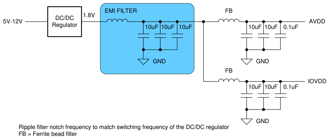
图 10-3. Example Switcher-Only Approach
