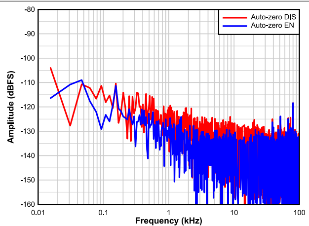
图 8-14. F_S = 65 \text{ MSPS} , F_{IN} = 5 \text{ MHz}
