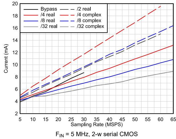
图 6-61. I_{OVDD} Current vs Decimation
