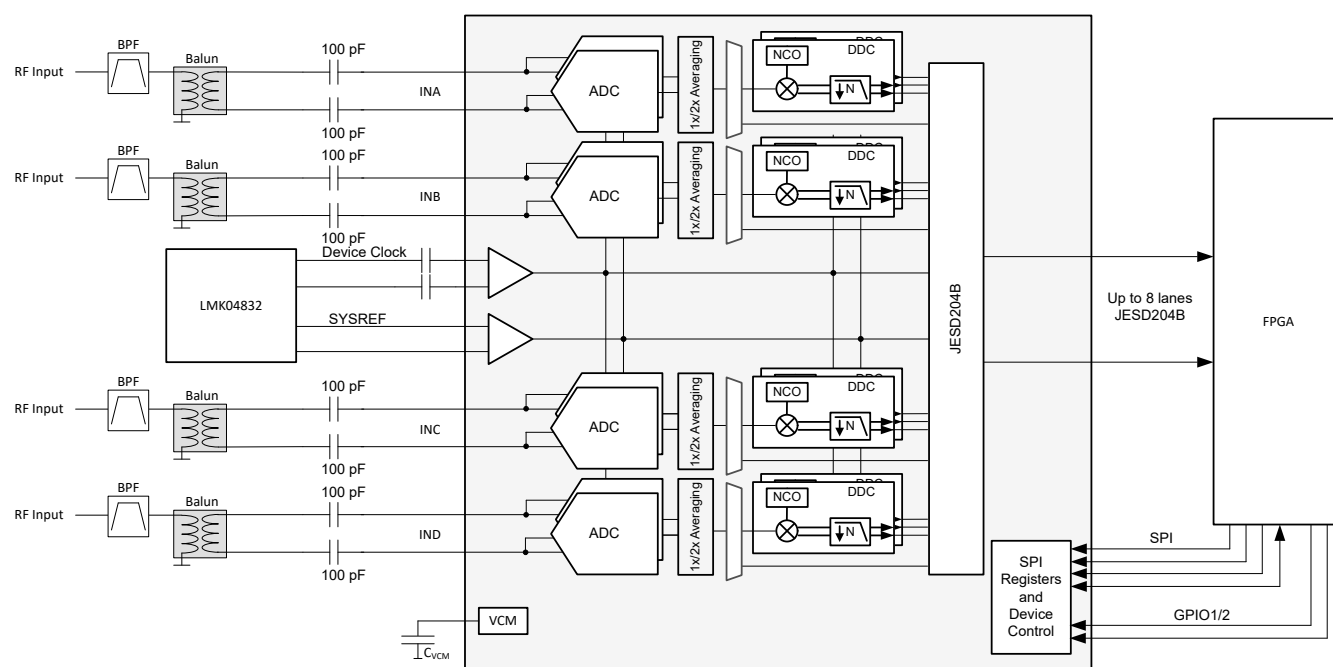
图 7-1. Typical Configuration for Wideband RF Sampling
