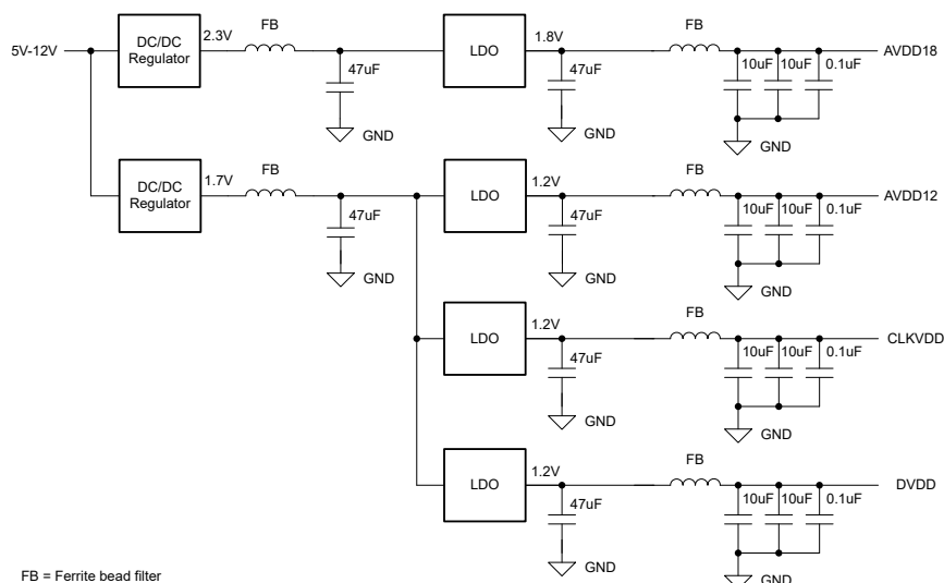
图 7-6. Power supply design example
