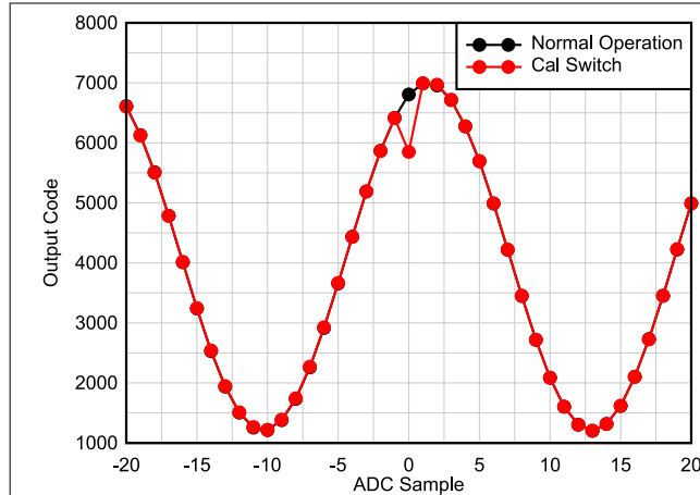
图 6-18. Output Code vs ADC Sample
