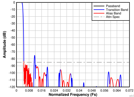
图 6-36. Complex Decimation by 128 Filter Response
