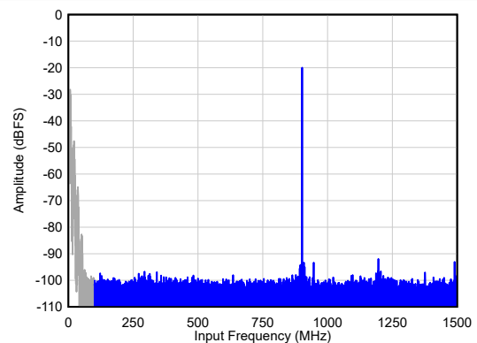
图 5-14. Single Tone FFT at F_{IN} = 900 MHz
