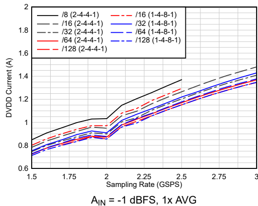
图 5-44. Current vs Sampling Rate vs Real Decimation
