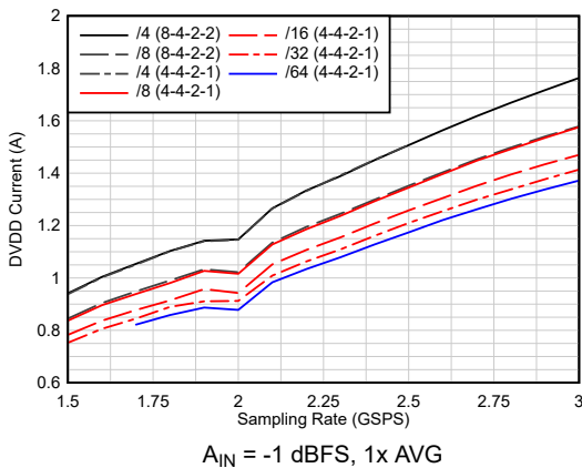
图 5-43. Current vs Sampling Rate vs Real Decimation
