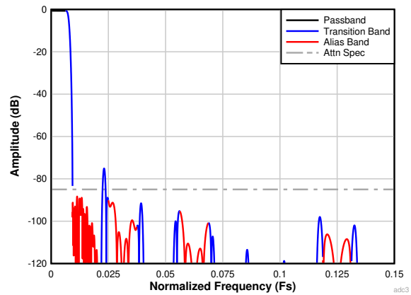
图 6-33. Complex Decimation by 64 Filter Response
