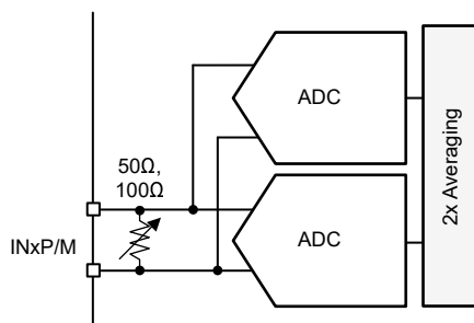
图 6-45. Internal Digital Averaging
