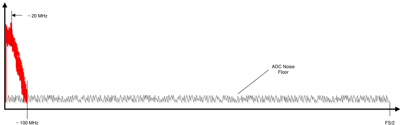
图 6-7. Analog out-of-band dither
