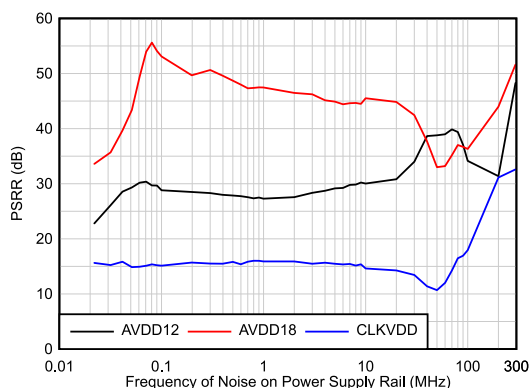
图 7-5. Power supply rejection ratio (PSRR) vs frequency
