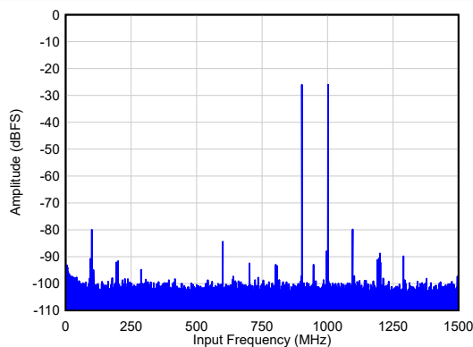
图 5-19. Two Tone FFT at F_{IN} = 900/1000 MHz
