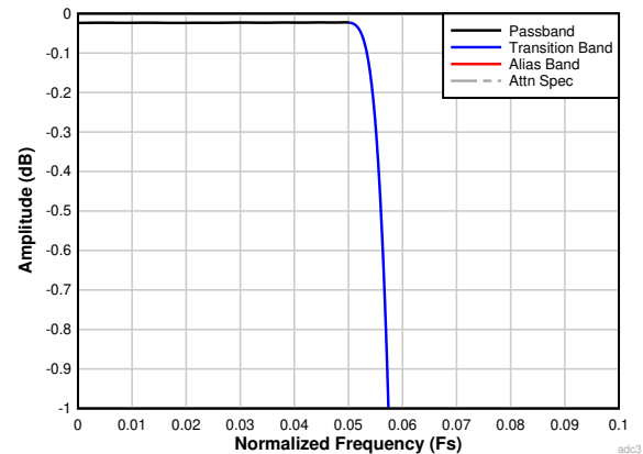
图 6-27. Decimation by 8 Passband Ripple Response
