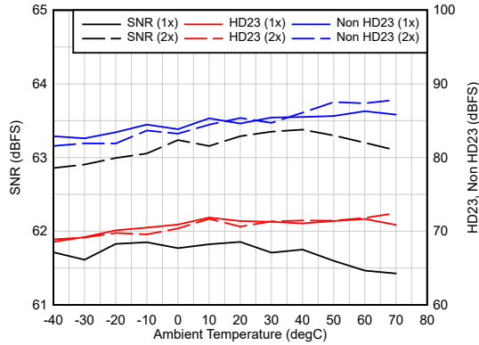
图 5-35. AC Performance vs Temperature
