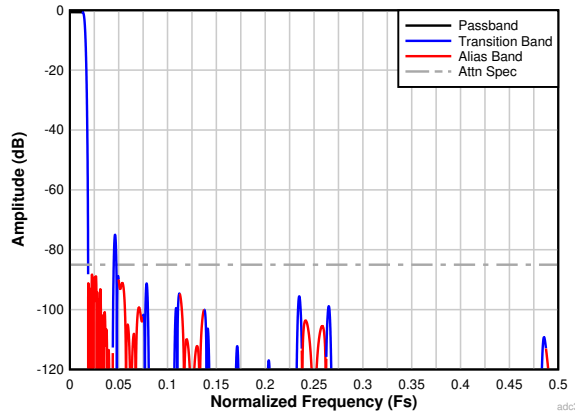
图 6-30. Complex Decimation by 32 Filter Response
