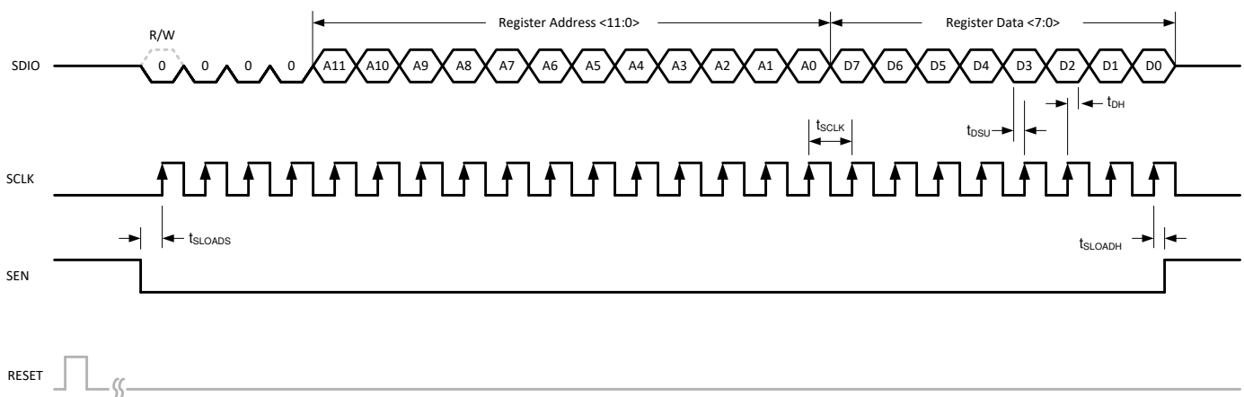
图 6-46. Serial Register Write Timing Diagram
