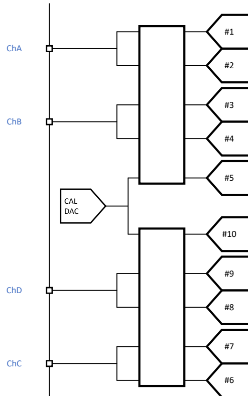
图 6-15. Internal ADC setup for 2x averaging mode
