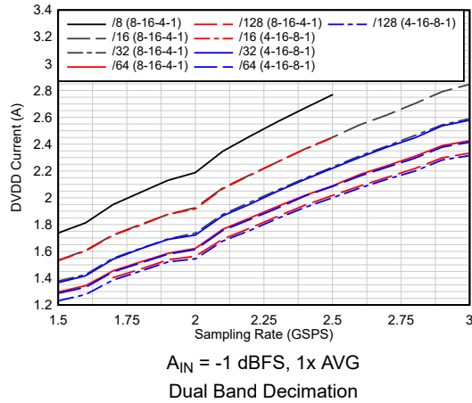
图 5-47. Current vs Sampling Rate vs Complex Decimation
