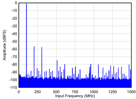
图 5-1. Single Tone FFT at F_{IN} = 100 MHz
