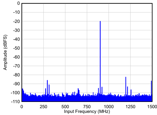
图 5-17. Single Tone FFT at F_{IN} = 900 MHz
