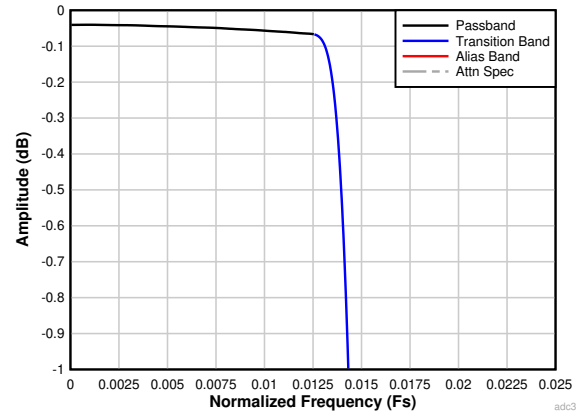
图 6-31. Decimation by 32 Passband Ripple Response
