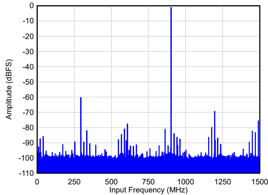
图 5-5. Single Tone FFT at F_{IN} = 900 MHz
