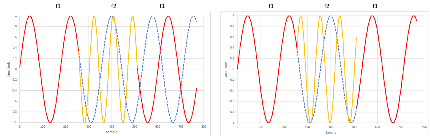
图 6-39. Phase Continuous (left) and Infinite Phase Coherent (right) NCO Frequency Switching
