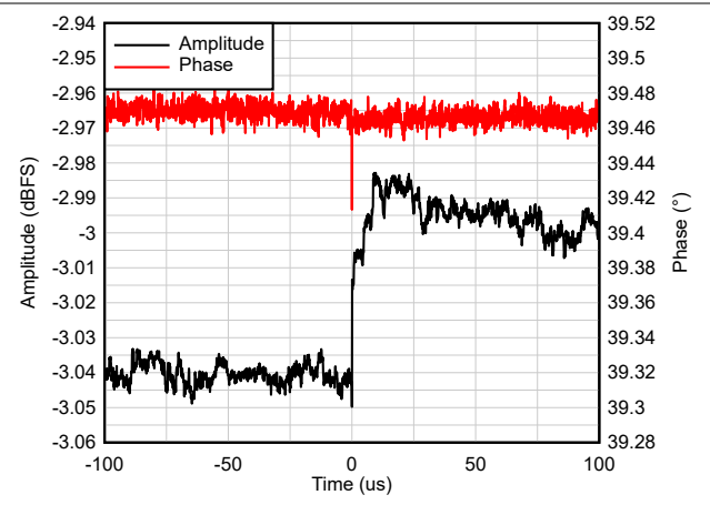
图 6-19. Amplitude and Phase vs Time
