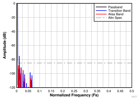
图 6-35. Complex Decimation by 128 Filter Response
