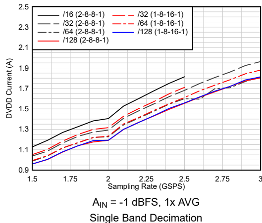
图 5-46. Current vs Sampling Rate vs Complex Decimation
