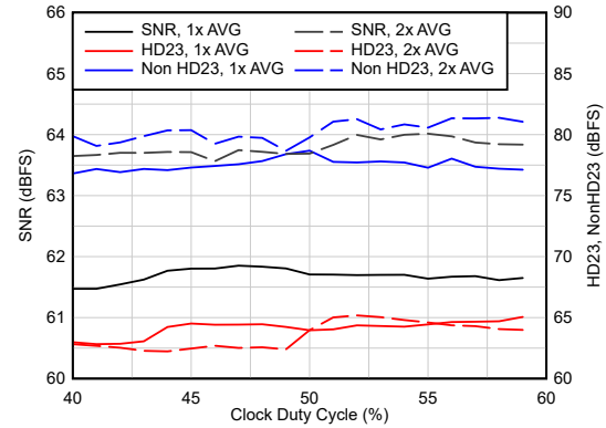
图 5-36. AC Performance vs Clock Duty Cycle
