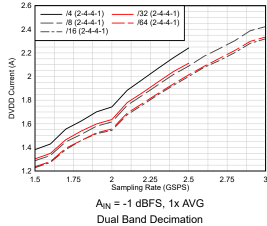
图 5-48. Current vs Sampling Rate vs Complex Decimation
