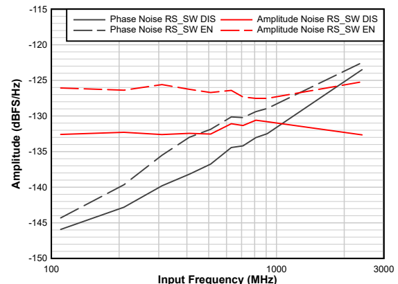
图 6-11. Amplitude and Phase noise at 10 kHz offset vs Input Frequency
