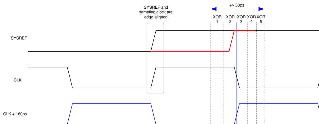
图 6-22. Detection of SYSREF Transition within Capture Window
