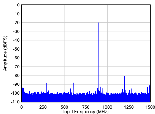
图 5-13. Single Tone FFT at F_{IN} = 900 MHz
