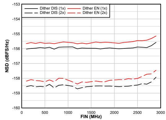
图 5-24. AC Performance vs F_{IN}
