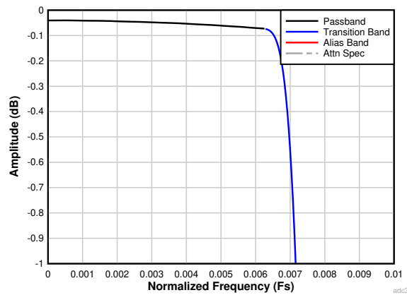
图 6-34. Decimation by 64 Passband Ripple Response
