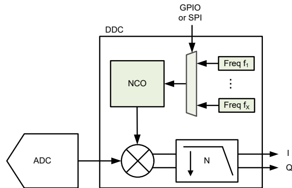
图 6-38. Phase Coherent NCO Block Diagram
