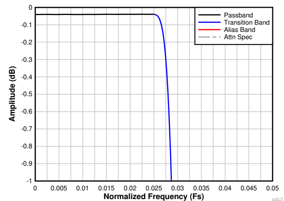
图 6-29. Decimation by 16 Passband Ripple Response
