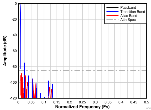
图 6-32. Complex Decimation by 64 Filter Response
