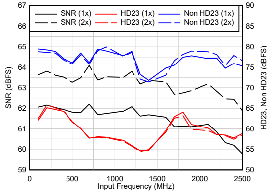
图 5-23. AC Performance vs F_{IN}
