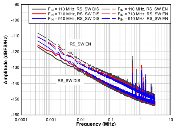
图 6-10. Amplitude Noise vs Input Frequency
