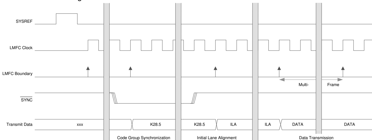
图 6-42. JESD204B Internal Timing Diagram
