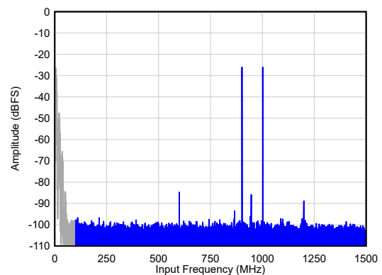
图 5-20. Two Tone FFT at F_{IN} = 900/1000 MHz
