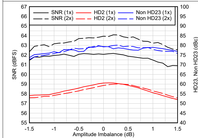
图 6-5. Amplitude Imbalance - 3.0 GSPS
