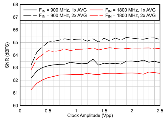
图 6-13. SNR vs Clock Amplitude (Dither ON)
