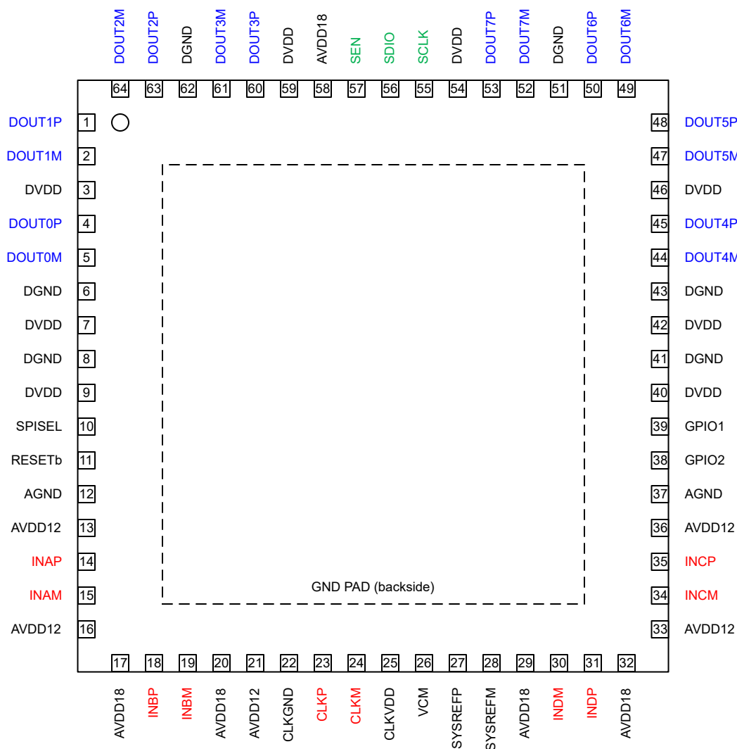
图 4-1. RTD Package, 64 Pin QFN (Top View)
