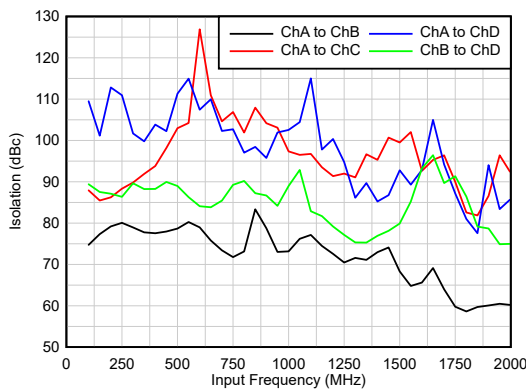
图 5-37. Isolation vs Input Frequency
