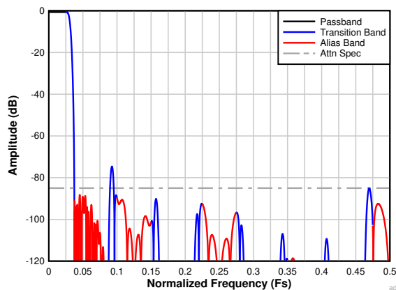
图 6-28. Complex Decimation by 16 Filter Response
