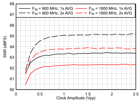
图 6-12. SNR vs Clock Amplitude (Dither OFF)
