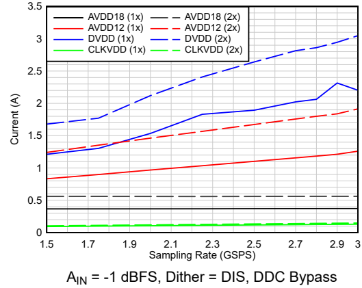
图 5-42. Current vs Sampling Rate vs Averaging
