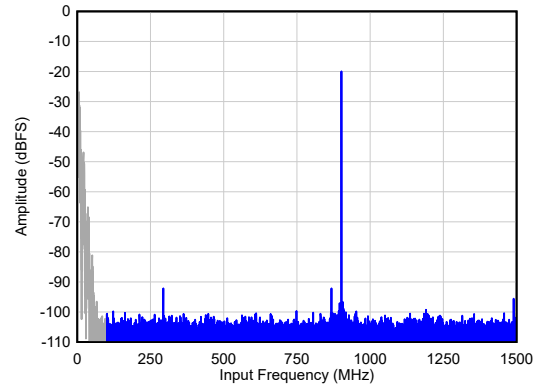
图 5-18. Single Tone FFT at F_{IN} = 900 MHz
