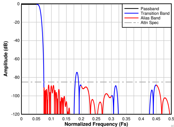
图 6-26. Complex Decimation by 8 Filter Response
