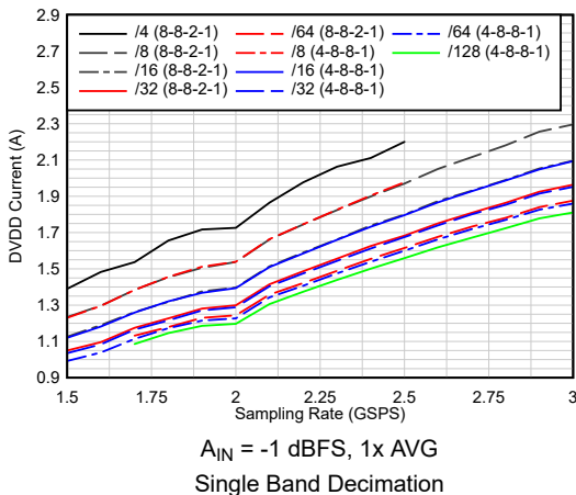
图 5-45. Current vs Sampling Rate vs Complex Decimation
