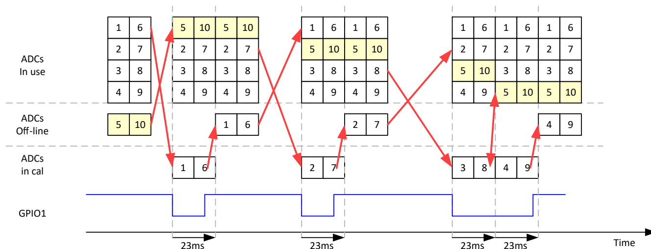
图 6-16. Timing diagram - calibration (2x AVG example)
