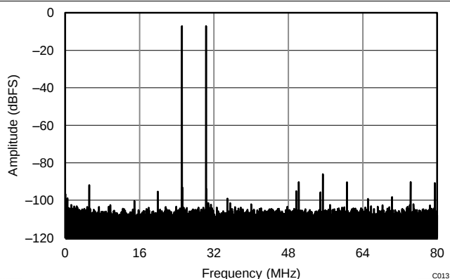
Figure 13. FFT for Two-Tone Input Signal (-7 dBFS at 185 MHz and 190 MHz)
