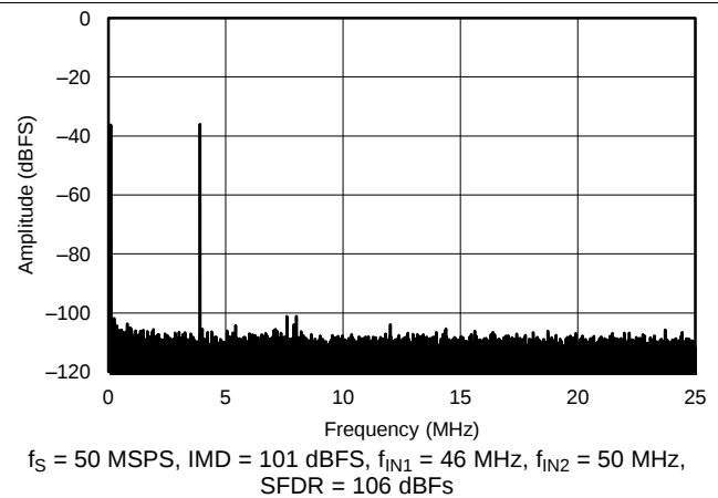
Figure 111. FFT for Two-Tone Input Signal ( -36\text{ dBFS} at 46\text{ MHz} and 50\text{ MHz} )
