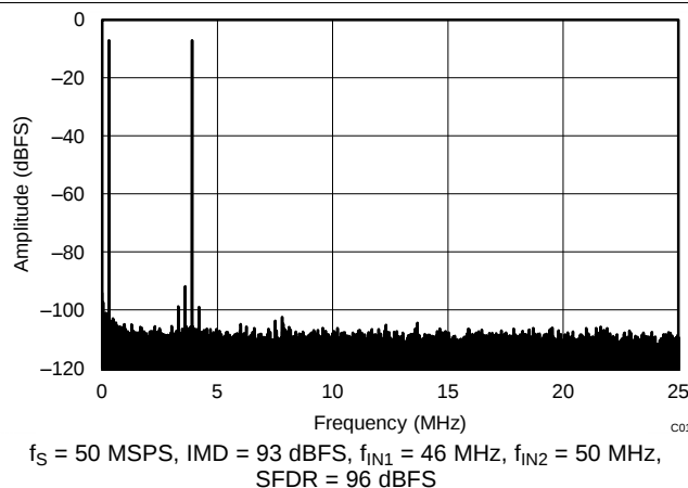
Figure 110. FFT for Two-Tone Input Signal ( -7\text{ dBFS} at 46\text{ MHz} and 50\text{ MHz} )
