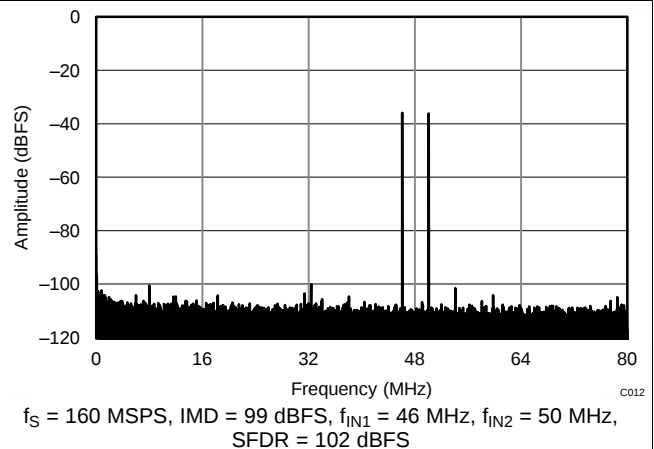
Figure 12. FFT for Two-Tone Input Signal (-36 dBFS at 46 MHz and 50 MHz)
