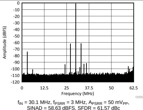
Figure 134. Power-Supply Rejection Ratio Spectrum (Chopper On)
