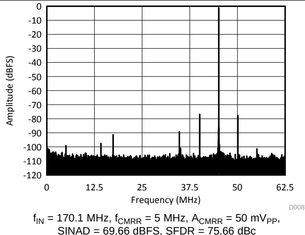
Figure 136. Common-Mode Rejection Ratio Spectrum
