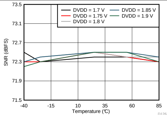
Figure 125. Signal-to-Noise Ratio vs DVDD Supply and Temperature (170 MHz)
