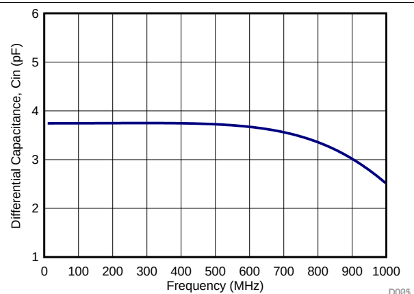
Figure 196. Differential Input Capacitance, C_{IN}
