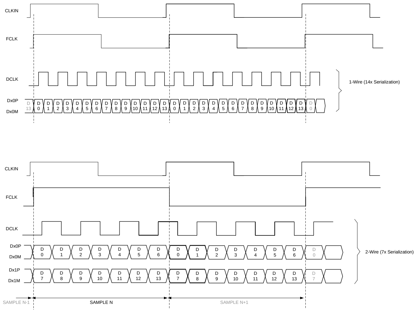
Figure 143. Output Timing Diagram
