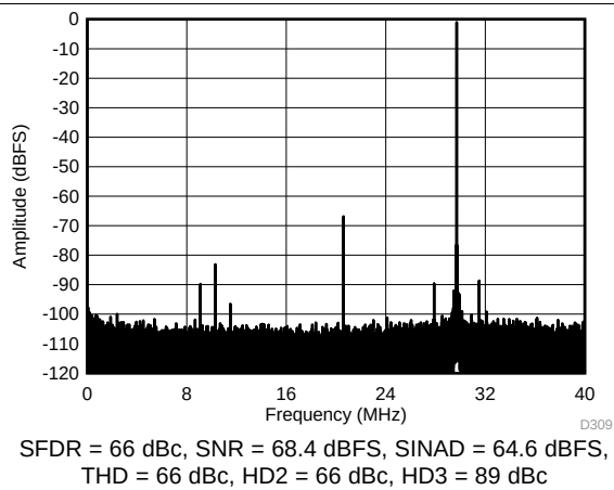
Figure 75. FFT for 450-MHz Input Signal (Dither On)
