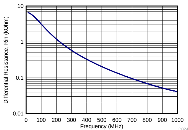
Figure 195. Differential Input Resistance, R_{IN}
