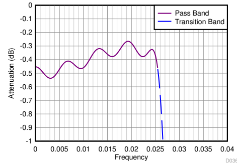
图 8-32. Divide-by-16 Filter Response (Zoomed)
