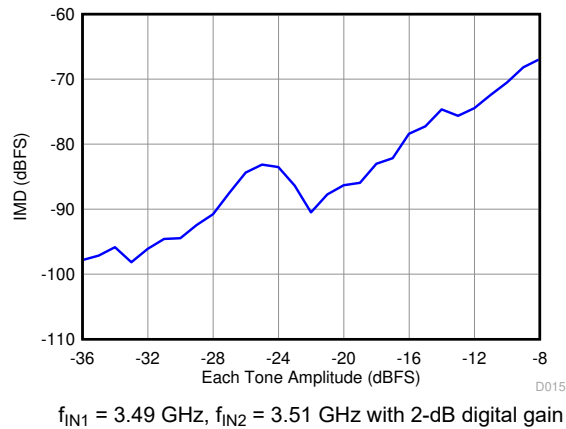
图 6-35. Intermodulation Distortion vs. Input Amplitude (3490 MHz and 3510 MHz)
