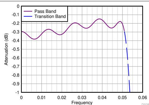
图 8-24. Divide-by-8 Filter Response (Zoomed)
