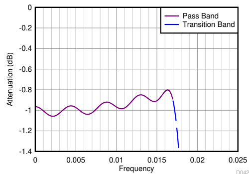
图 8-38. Divide-by-24 Filter Response (Zoomed)
