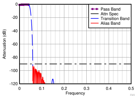
图 8-27. Divide-by-10 Filter Response
