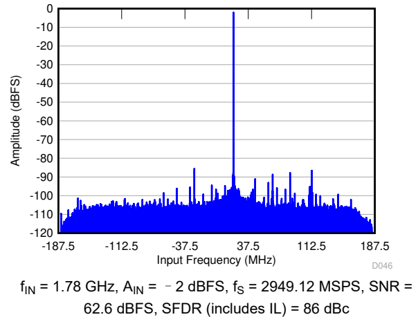
图 6-70. FFT in 8x Decimation (Complex Output)
