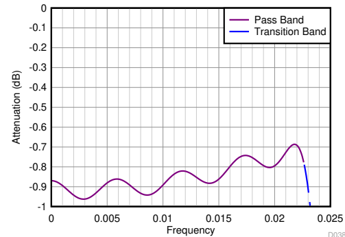
图 8-34. Divide-by-18 Filter Response (Zoomed)
