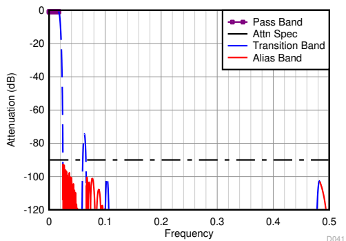
图 8-37. Divide-by-24 Filter Response
