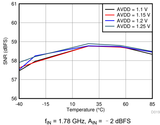
图 6-43. Signal-to-Noise Ratio vs. AVDD Supply and Temperature
