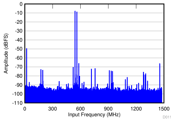
f_{IN1} = 3.49 \text{ MHz} , f_{IN2} = 3.51 \text{ GHz} , IMD = 66 dBFS, A_{IN} = -3 \text{ dBFS} with 2-dB gain
