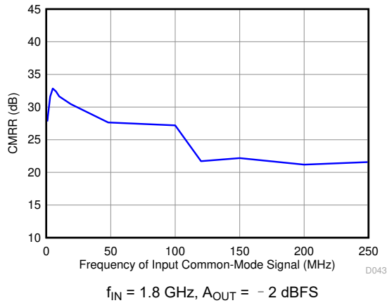
图 6-67. Common-Mode Rejection Ratio vs. Tone Frequency
