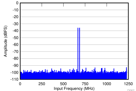
图 6-20. FFT for Two-Tone Input Signal (-36 dBFS)
