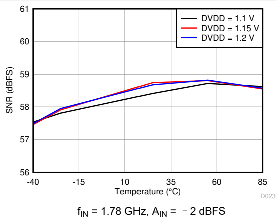
图 6-47. Signal-to-Noise Ratio vs. DVDD Supply and Temperature
