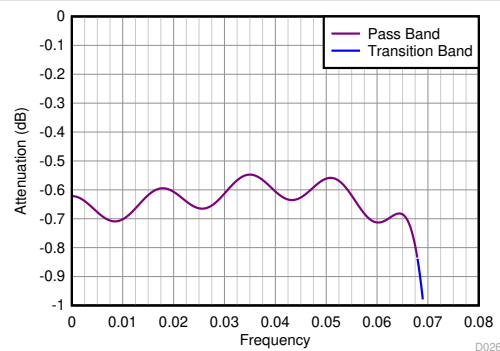
图 8-22. Divide-by-6 Filter Response (Zoomed)
