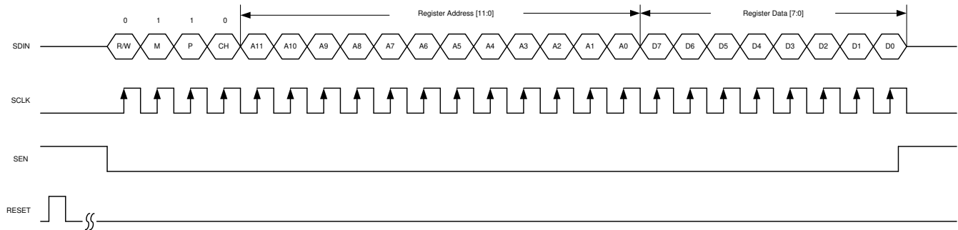
图 8-61. SPI Write Timing Diagram for Digital Bank Register Write
