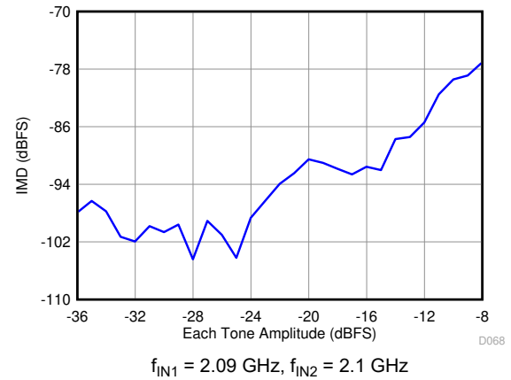
图 6-34. Intermodulation Distortion vs. Input Amplitude (1800 MHz and 2600 MHz, f_s = 2457.6 MSPS)
