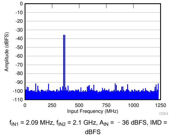
图 6-26. FFT for Two-Tone Input Signal ( - 36 dBFS, f_s = 2457.6 \text{ MSPS} )
