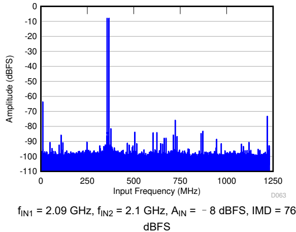
图 6-25. FFT for Two-Tone Input Signal ( - 8 dBFS, f_s = 2457.6 \text{ MSPS} )
