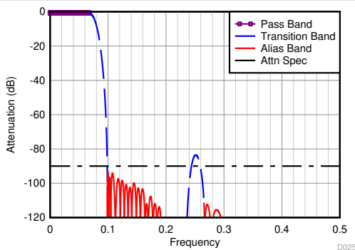
图 8-21. Divide-by-6 Filter Response
