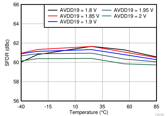
图 6-52. Spurious-Free Dynamic Range vs. AVDD19 Supply and Temperature
