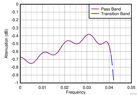
图 8-28. Divide-by-10 Filter Response (Zoomed)
