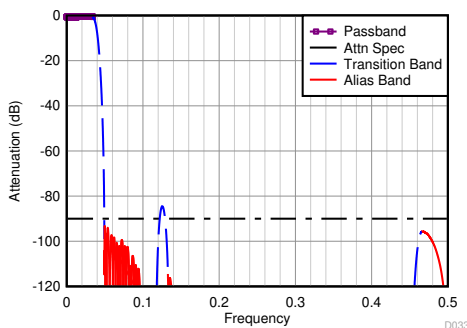
图 8-29. Divide-by-12 Filter Response
