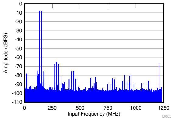
f_{IN1} = 2.59 \text{ GHz} , f_{IN2} = 2.6 \text{ GHz} , A_{IN} = -8 \text{ dBFS} , IMD = 65 dBFS
