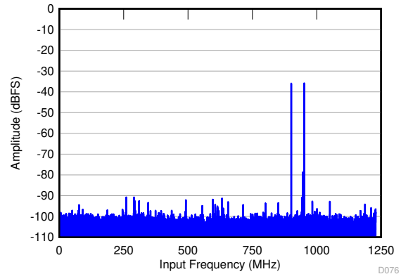
图 6-16. FFT for Two-Tone Input Signal (-36 dBFS)
