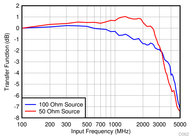
图 8-5. Input Bandwidth With a 100- \Omega Source Resistance
