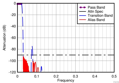
图 8-35. Divide-by-20 Filter Response
