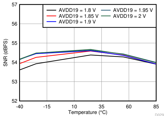
图 6-51. Signal-to-Noise Ratio vs. AVDD19 Supply and Temperature
