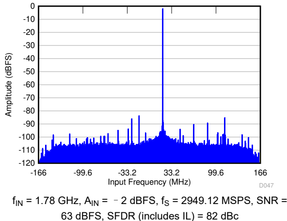
图 6-71. FFT in 9x Decimation (Complex Output)
