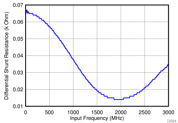
图 8-4. Differential Input Resistance vs. Input Frequency
