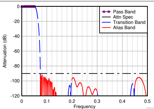
图 8-23. Divide-by-8 Filter Response
