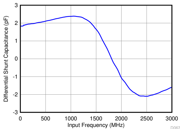
图 8-3. Differential Input Capacitance vs. Input Frequency
