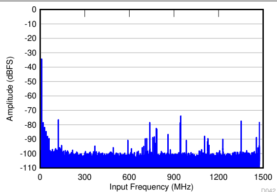
图 6-64. Power-Supply Rejection Ratio FFT for Test Signal on AVDD Supply
