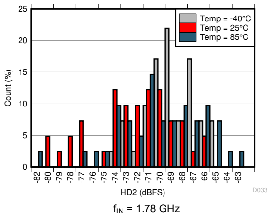
图 6-57. HD2 Histogram at AVDD19 = 2.0 V
