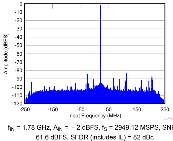
图 6-69. FFT in 6x Decimation (Complex Output)
