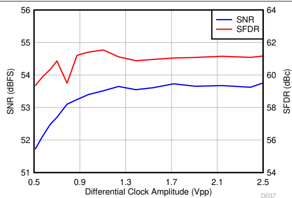
图 6-61. Performance vs. Clock Amplitude
