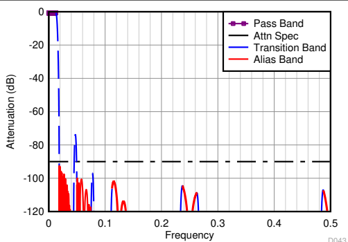
图 8-39. Divide-by-32 Filter Response
