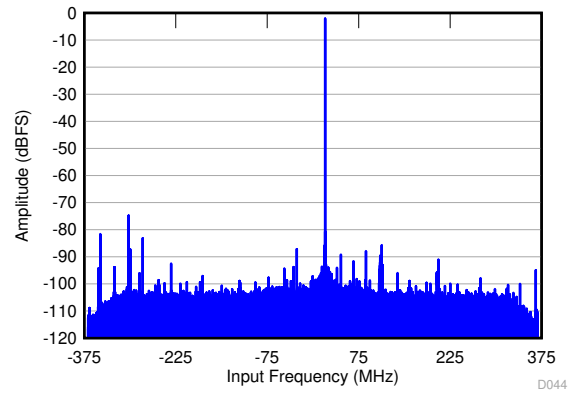
图 6-68. FFT in 4x Decimation (Complex Output)
