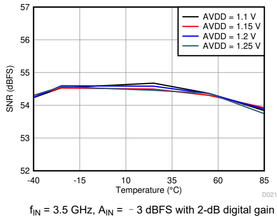
图 6-45. Signal-to-Noise Ratio vs. AVDD Supply and Temperature
