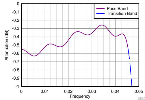
图 8-26. Divide-by-9 Filter Response (Zoomed)
