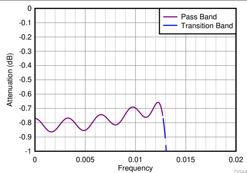
图 8-40. Divide-by-32 Filter Response (Zoomed)
