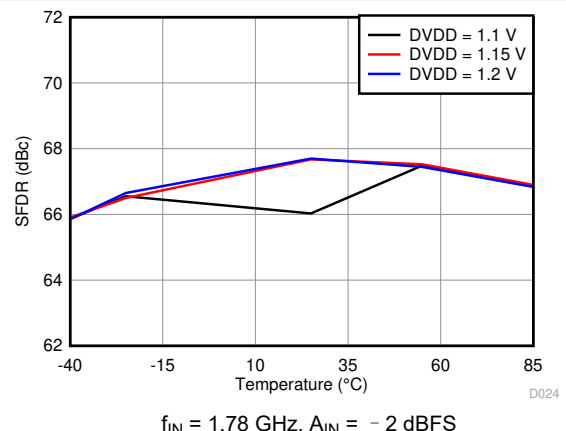
图 6-48. Spurious-Free Dynamic Range vs. DVDD Supply and Temperature
