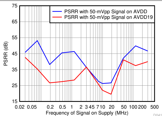
图 6-65. Power-Supply Rejection Ratio vs. Tone Frequency
