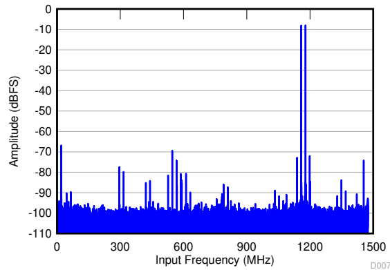
图 6-19. FFT for Two-Tone Input Signal (-8 dBFS)
