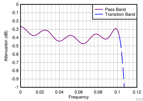
图 8-20. Divide-by-4 Filter Response (Zoomed)
