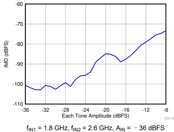
图 6-33. Intermodulation Distortion vs. Input Amplitude (1800 MHz and 2600 MHz)
