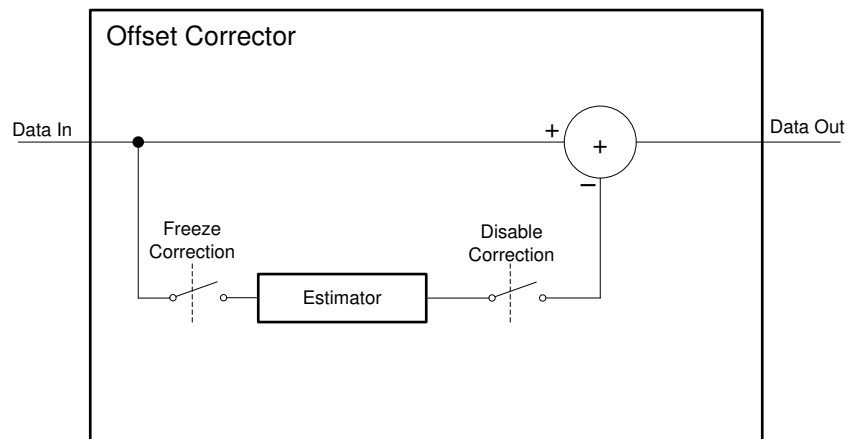
图 9-6. Offset Corrector in the ADC32RF8x
