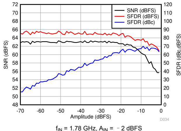
图 6-58. Performance vs. Amplitude
