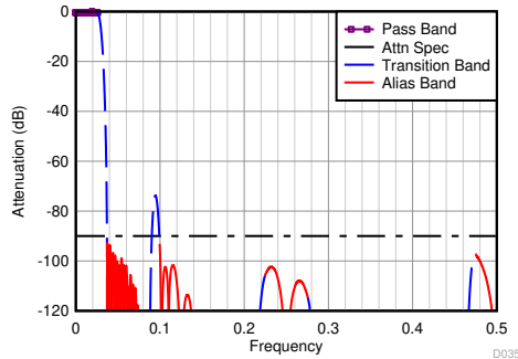
图 8-31. Divide-by-16 Filter Response
