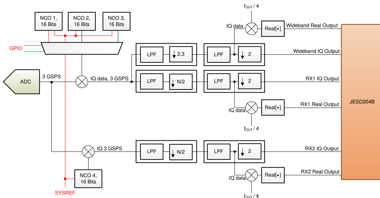
图 8-14. DDC Chains Overview (One ADC Channel Shown)
