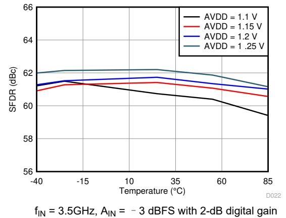
图 6-46. Spurious-Free Dynamic Range vs. AVDD Supply and Temperature
