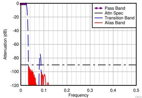
图 8-33. Divide-by-18 Filter Response
