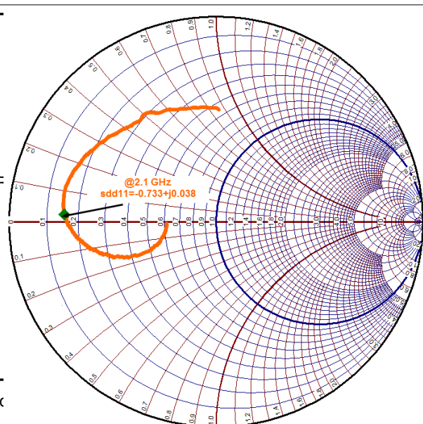
图 8-2. SDD11 Over the Input Frequency Range
