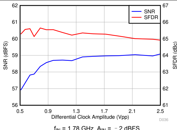
图 6-60. Performance vs. Clock Amplitude
