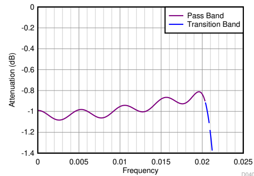
图 8-36. Divide-by-20 Filter Response (Zoomed)
