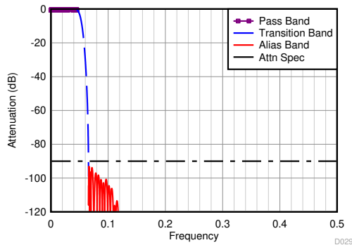
图 8-25. Divide-by-9 Filter Response
