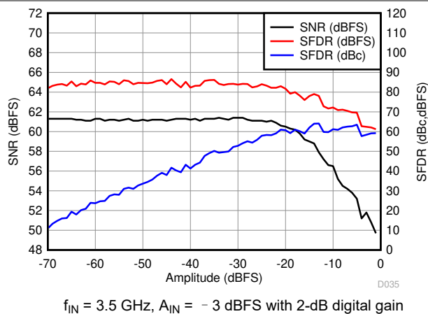
图 6-59. Performance vs. Amplitude
