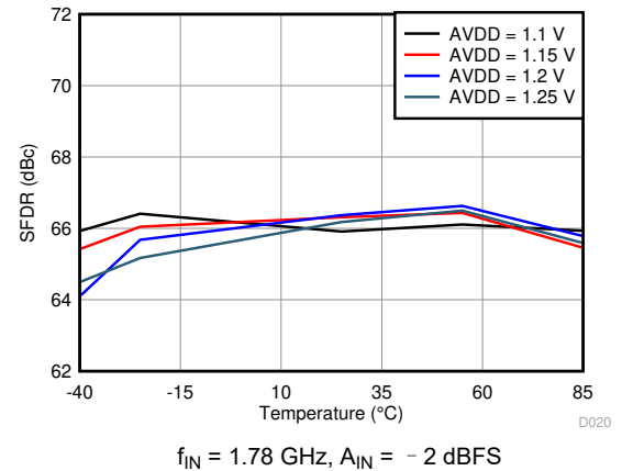
图 6-44. Spurious-Free Dynamic Range vs. AVDD Supply and Temperature
