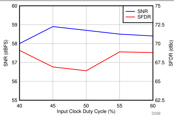
图 6-62. Performance vs. Clock Duty Cycle
