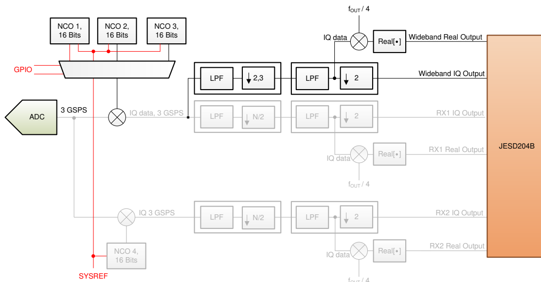
图 8-16. Decimation Filter Implementation for Single-Band and Wide-Bandwidth Mode
