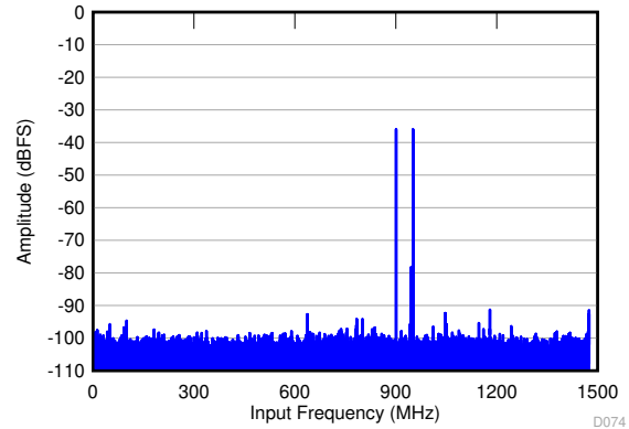
图 6-16. FFT for Two-Tone Input Signal (-36 dBFS)
