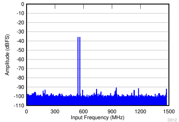
f_{IN1} = 3.49 \text{ GHz} , f_{IN2} = 3.51 \text{ GHz} , IMD = 92 dBFS, A_{IN} = -3 \text{ dBFS} with 2-dB gain
