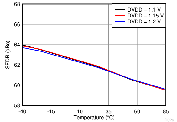
图 6-50. Spurious-Free Dynamic Range vs. DVDD Supply and Temperature
