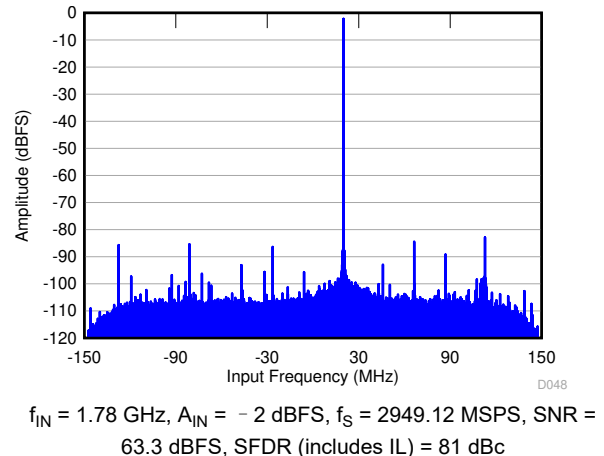
图 6-72. FFT in 10x Decimation (Complex Output)
