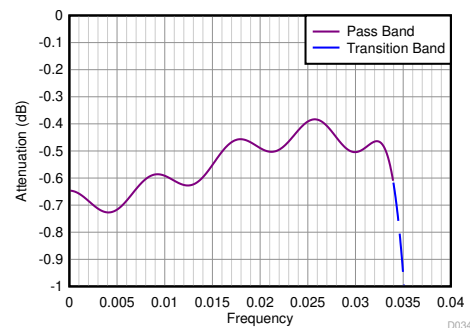
图 8-30. Divide-by-12 Filter Response (Zoomed)
