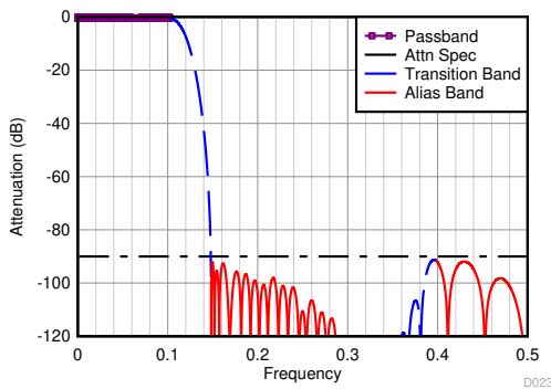
图 8-19. Divide-by-4 Filter Response
