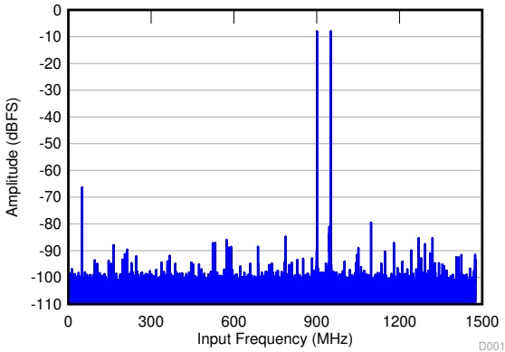
图 6-15. FFT for Two-Tone Input Signal (-8 dBFS)
