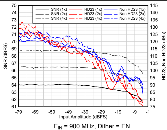
图 6-87. AC Performance vs A_{IN}
