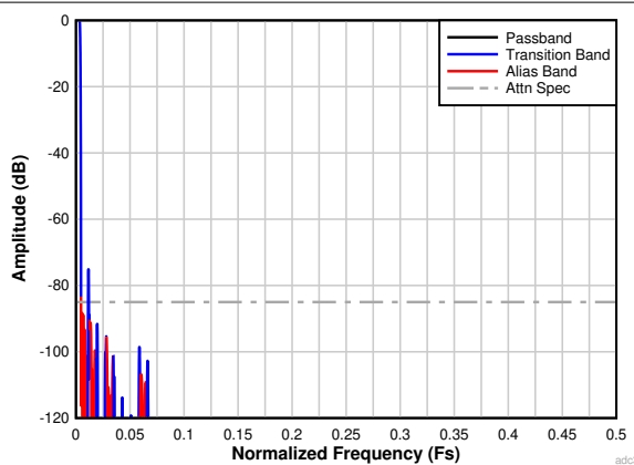
图 7-35. Complex Decimation by 128 Filter Response
