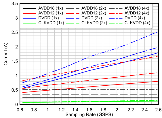
图 6-47. Current vs Sampling Rate vs Averaging
