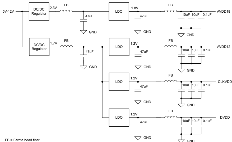
图 8-6. Power Supply Design Example
