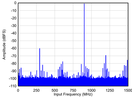
图 6-60. Single Tone FFT at F_{IN} = 900 MHz
