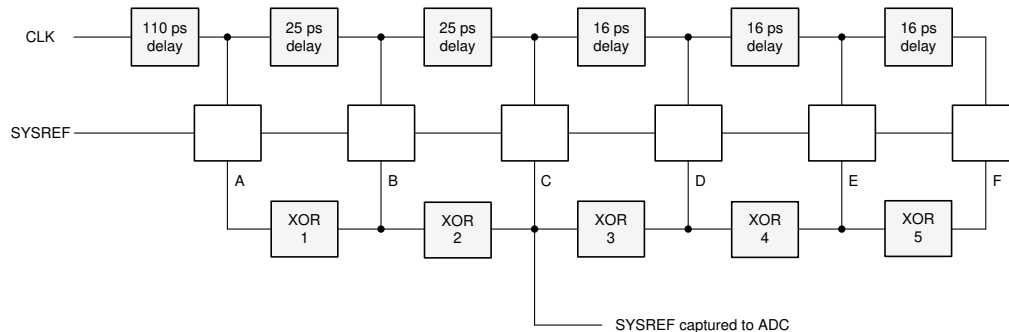
图 7-16. SYSREF Detection Circuitry
