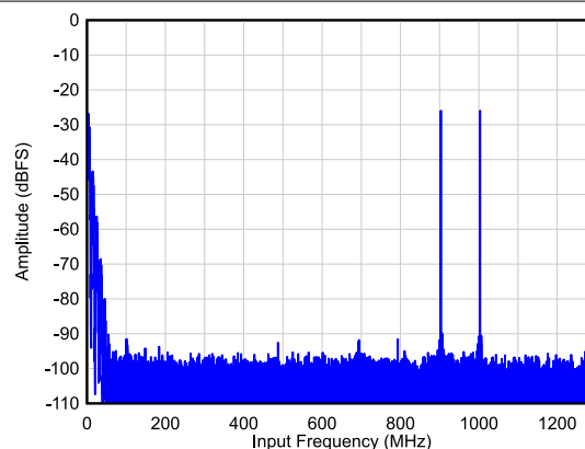
图 6-24. Two Tone FFT at F_{IN} = 900/1000 MHz
