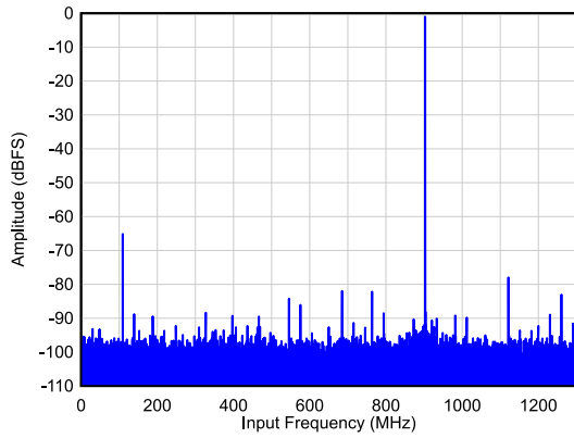
图 6-5. Single Tone FFT at F_{IN} = 900 MHz
