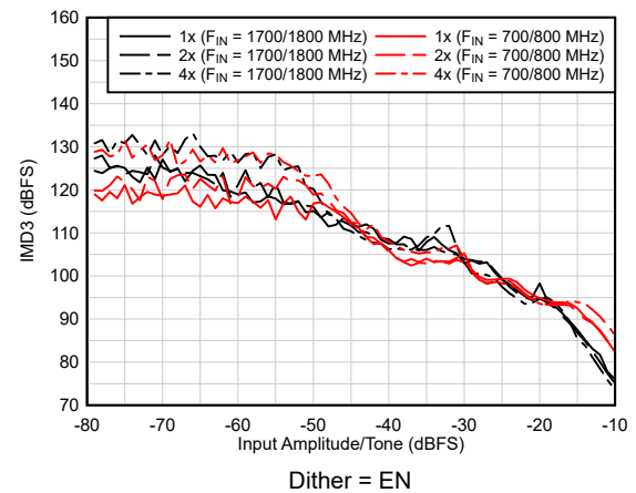
图 6-89. IMD3 Performance vs A_{IN}
