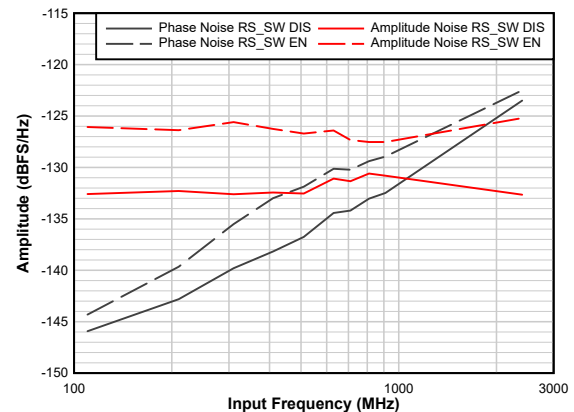
图 7-11. Amplitude and Phase noise at 10 kHz offset vs Input Frequency
