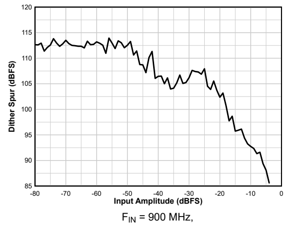
图 6-30. Dither Spur vs A_{IN}
