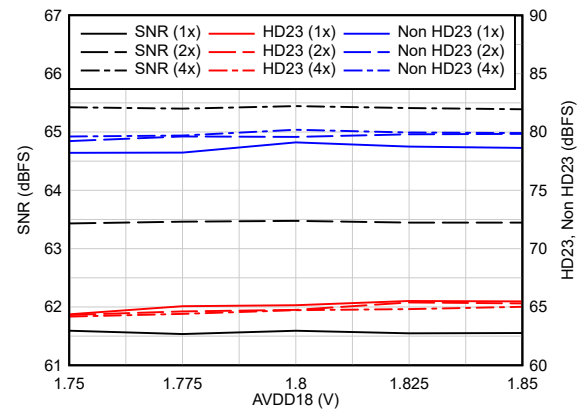
图 6-91. AC Performance vs AVDD18
