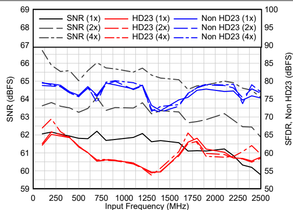
A_{IN} = -1 dBFS, Dither = DIS 图 6-82. AC Performance vs F_{IN}
