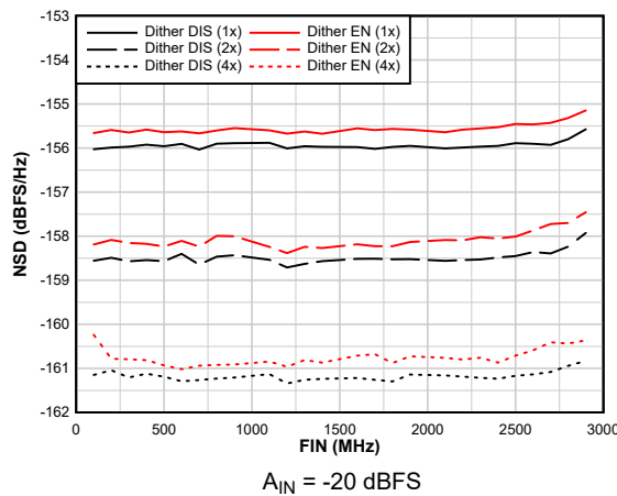
图 6-31. NSD Performance vs F_{IN}
