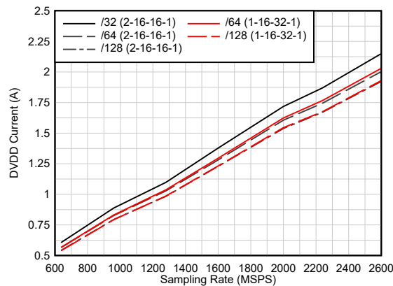
图 6-53. Current vs Sampling Rate vs Decimation
