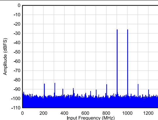
图 6-23. Two Tone FFT at F_{IN} = 900/1000 MHz
