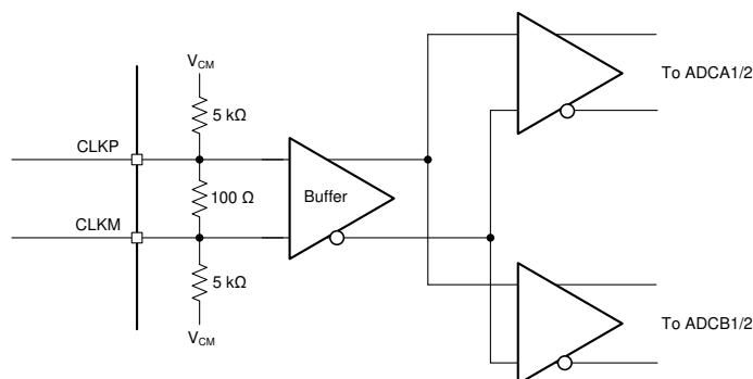
图 7-14. Internal Clock Input Routing
