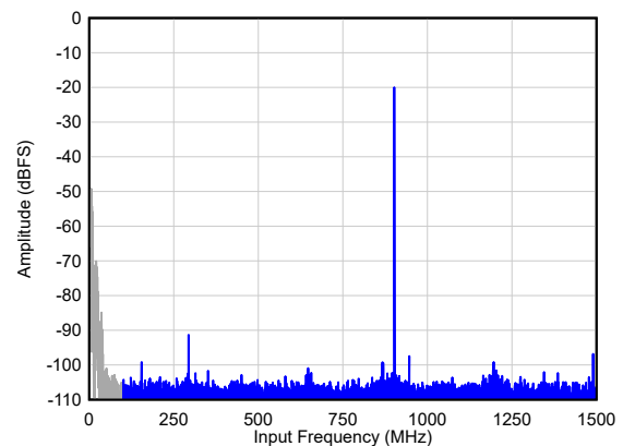
图 6-75. Single Tone FFT at F_{IN} = 900 MHz
