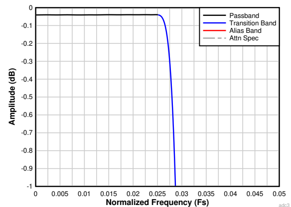
图 7-29. Decimation by 16 Passband Ripple Response
