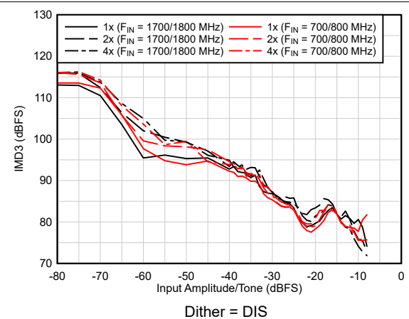
图 6-34. IMD3 Performance vs A_{IN}
