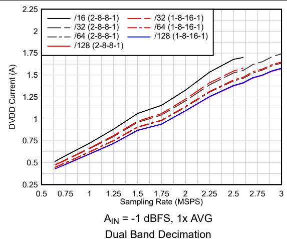
图 6-107. Current vs Sampling Rate vs Complex Decimation
