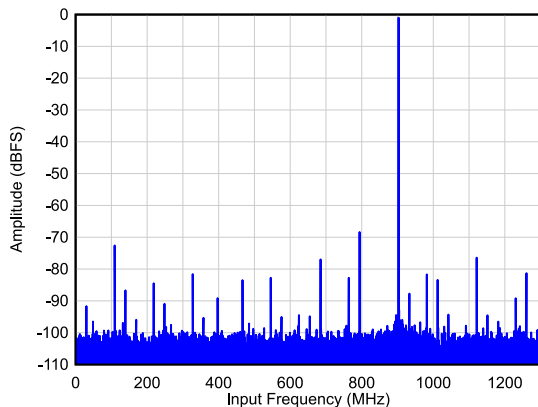
图 6-13. Single Tone FFT at F_{IN} = 900 MHz
