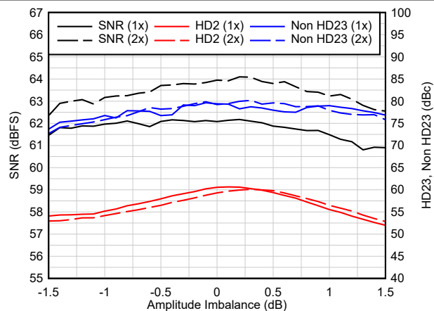
图 7-5. Amplitude Imbalance - 3.0 GSPS
