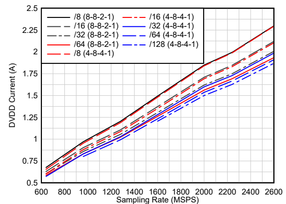
图 6-50. Current vs Sampling Rate vs Decimation
