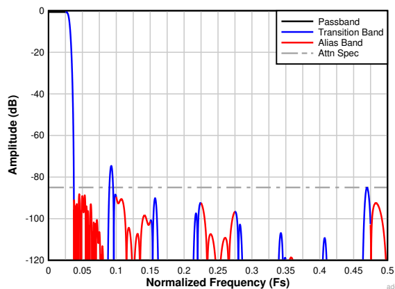
图 7-28. Complex Decimation by 16 Filter Response
