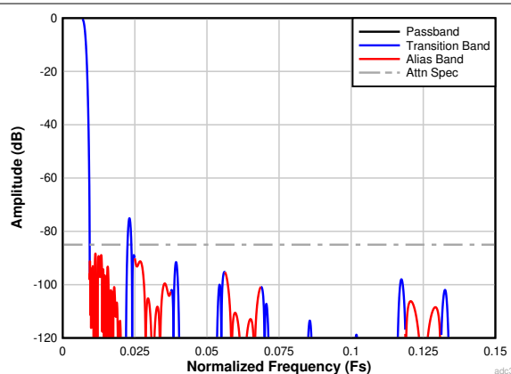
图 7-33. Complex Decimation by 64 Filter Response
