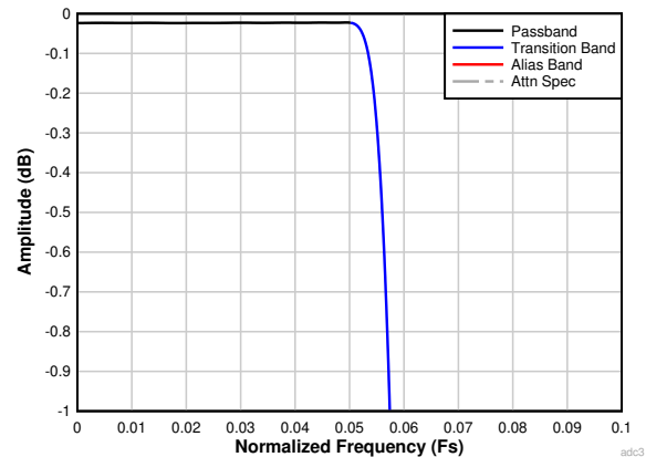
图 7-27. Decimation by 8 Passband Ripple Response
