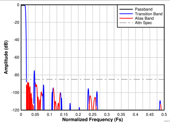
图 7-30. Complex Decimation by 32 Filter Response
