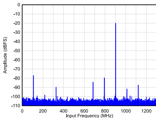
图 6-19. Single Tone FFT at F_{IN} = 900 MHz
