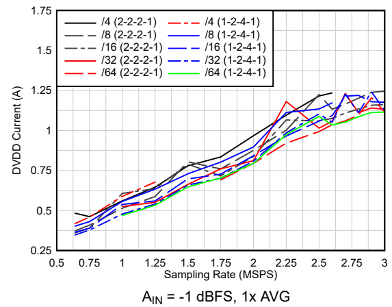
图 6-103. Current vs Sampling Rate vs Real Decimation
