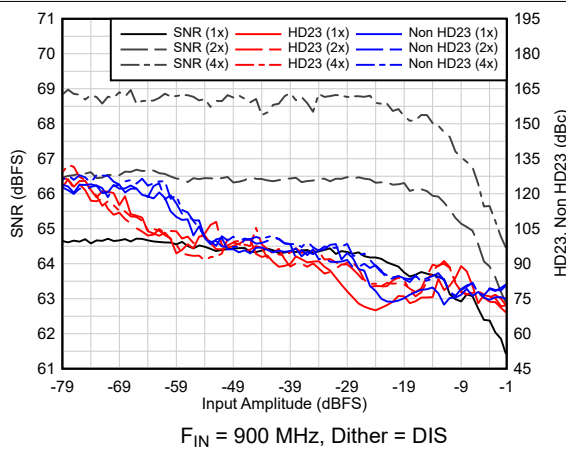
图 6-86. AC Performance vs A_{IN}
