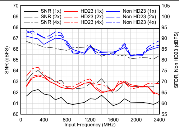
A_{IN} = -4 dBFS, Dither = EN 图 6-83. AC Performance vs F_{IN}
