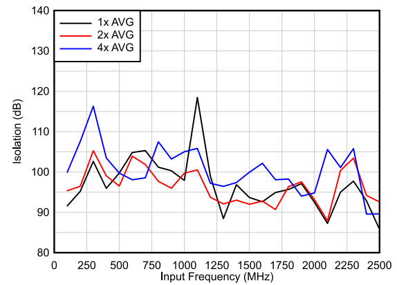
图 6-42. Isolation vs Input Frequency
