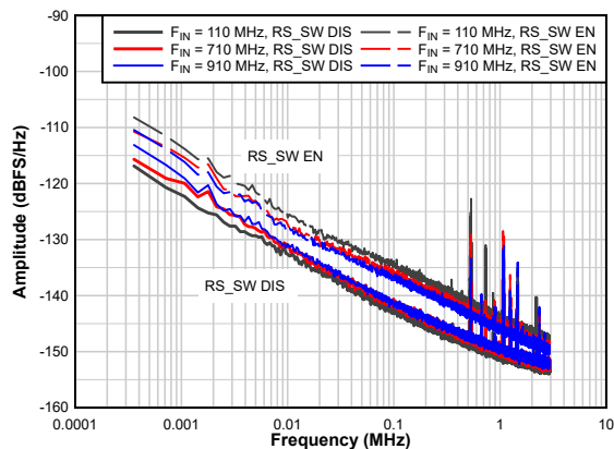
图 7-10. Amplitude Noise vs Input Frequency
