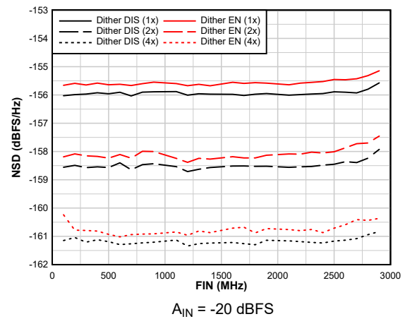
图 6-85. NSD Performance vs F_{IN}
