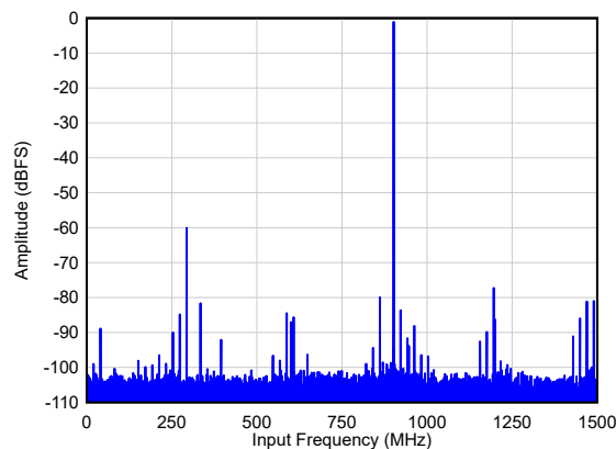
图 6-68. Single Tone FFT at F_{IN} = 900 MHz
