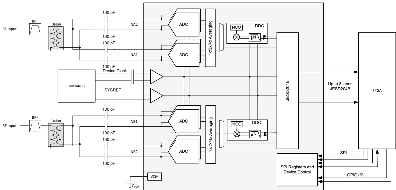
图 8-1. Typical Configuration for Wideband RF Sampling
