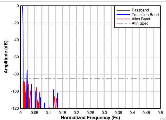
图 7-32. Complex Decimation by 64 Filter Response
