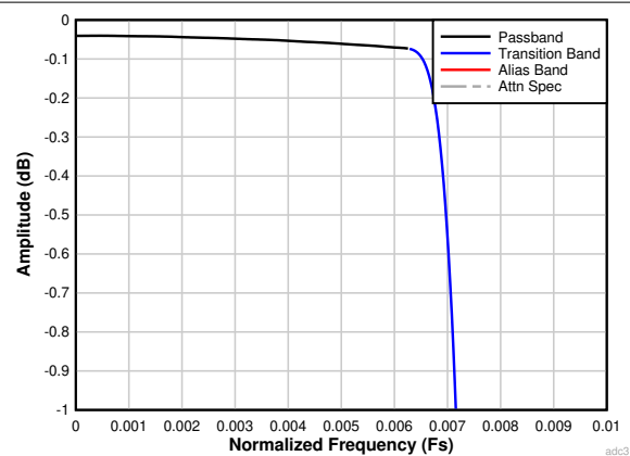
图 7-34. Decimation by 64 Passband Ripple Response
