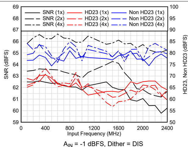
图 6-27. AC Performance vs F_{IN}
