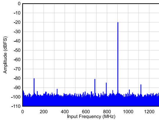
图 6-17. Single Tone FFT at F_{IN} = 900 MHz
