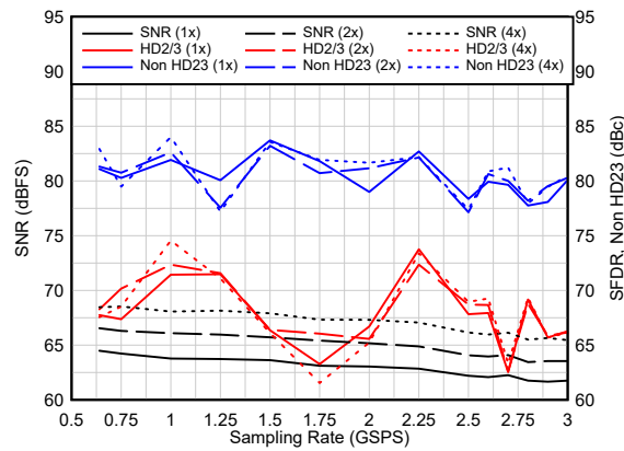
图 6-90. AC Performance vs F_S
