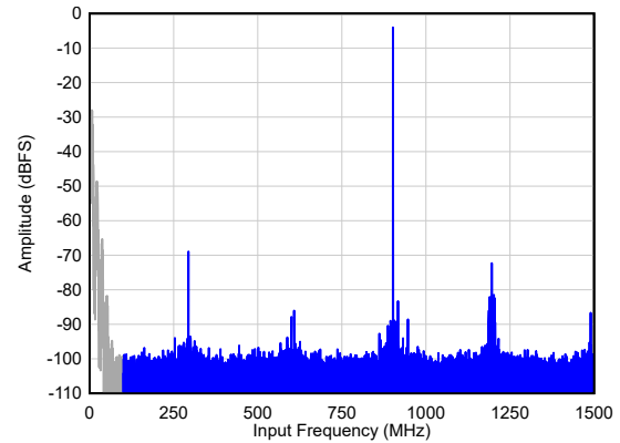
图 6-61. Single Tone FFT at F_{IN} = 900 MHz
