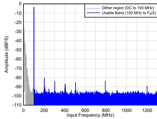
图 6-2. Single Tone FFT at F_{IN} = 100 MHz
