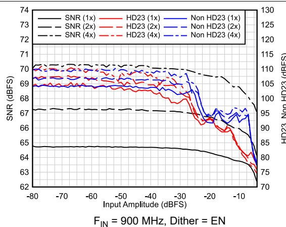
图 6-33. AC Performance vs A_{IN}
