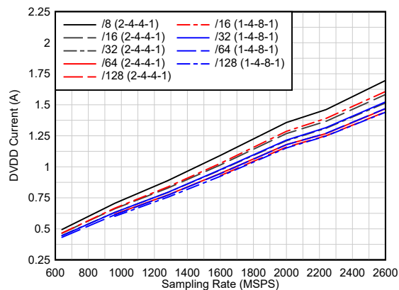
图 6-49. Current vs Sampling Rate vs Decimation
