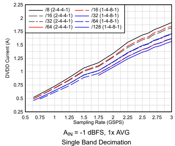
图 6-105. Current vs Sampling Rate vs Complex Decimation
