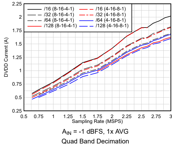
图 6-108. Current vs Sampling Rate vs Complex Decimation
