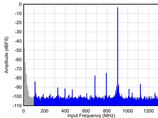
图 6-14. Single Tone FFT at F_{IN} = 900 MHz
