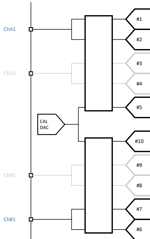
图 7-18. Internal ADC setup for 2x averaging mode
