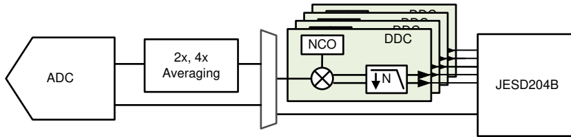
图 7-23. Digital Decimation Filter Options
