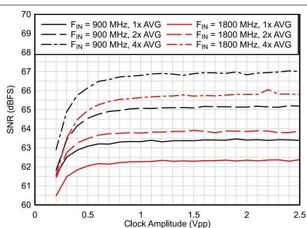
图 8-3. SNR vs Clock Amplitude (dither off)
