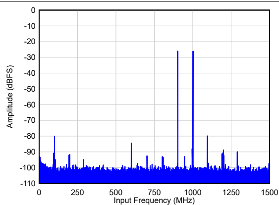
IMD3 = 54 dBc A_{IN} = -26 dBFS/tone, 1x AVG, Dither = DIS 图 6-80. Two Tone FFT at F_{IN} = 900/1000 MHz
