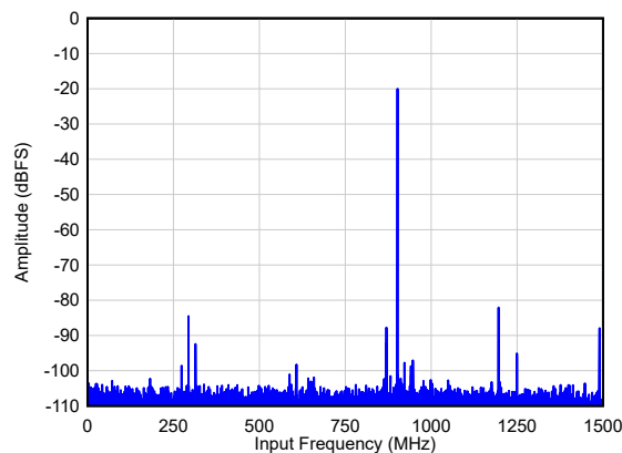
图 6-74. Single Tone FFT at F_{IN} = 900 MHz
