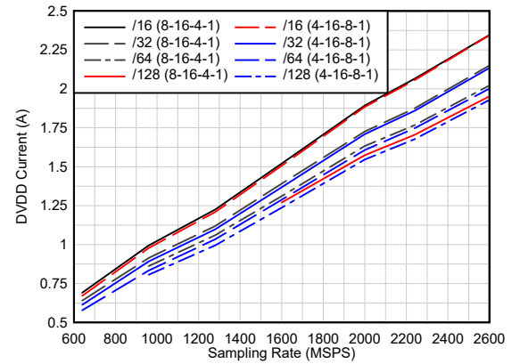
图 6-54. Current vs Sampling Rate vs Decimation
