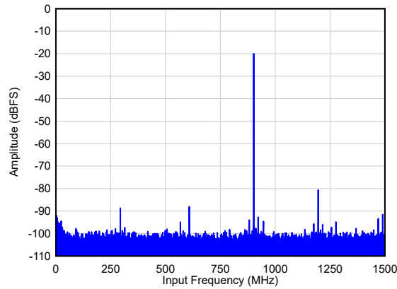
图 6-72. Single Tone FFT at F_{IN} = 900 MHz
