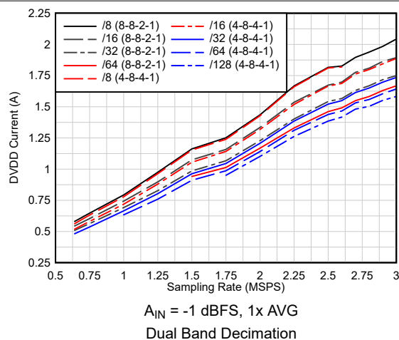
图 6-106. Current vs Sampling Rate vs Complex Decimation
