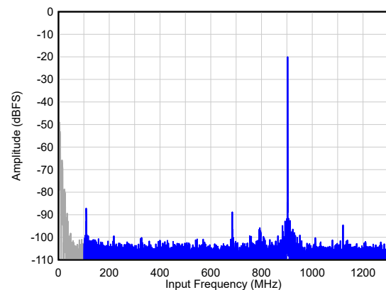
图 6-20. Single Tone FFT at F_{IN} = 900 MHz
