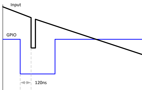
图 7-20. Timing Diagram Shows the ADC Switch
