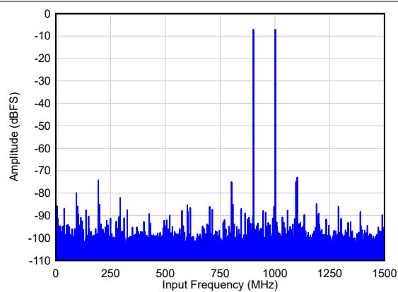
IMD3 = 68 dBc A_{IN} = -7 dBFS/tone, 1x AVG, Dither = DIS 图 6-78. Two Tone FFT at F_{IN} = 900/1000 MHz
