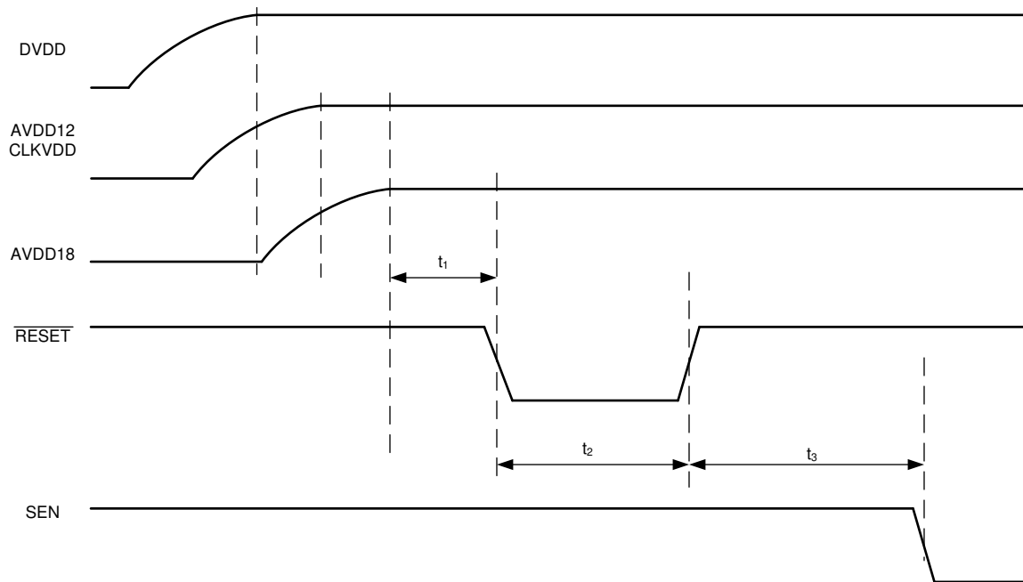
图 8-4. Initialization of Serial Registers After Power-Up
