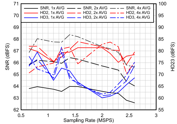
图 6-36. AC Performance vs F_s
