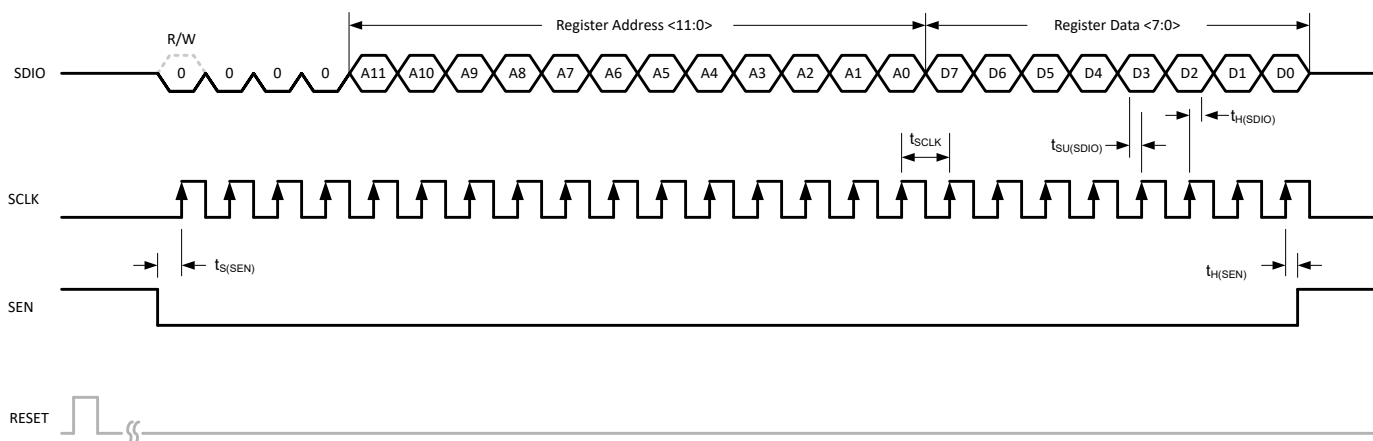
图 7-46. Serial Register Write Timing Diagram
