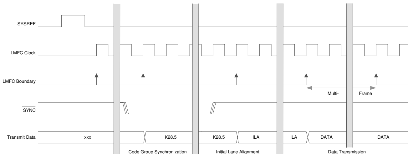
图 7-42. JESD204B Internal Timing Diagram
