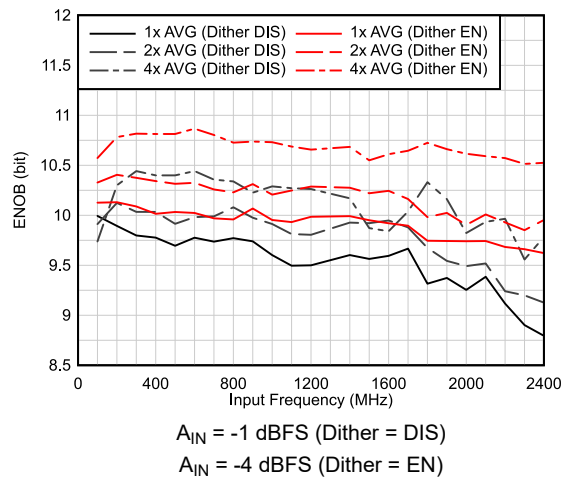
图 6-29. ENOB Performance vs F_{IN}
