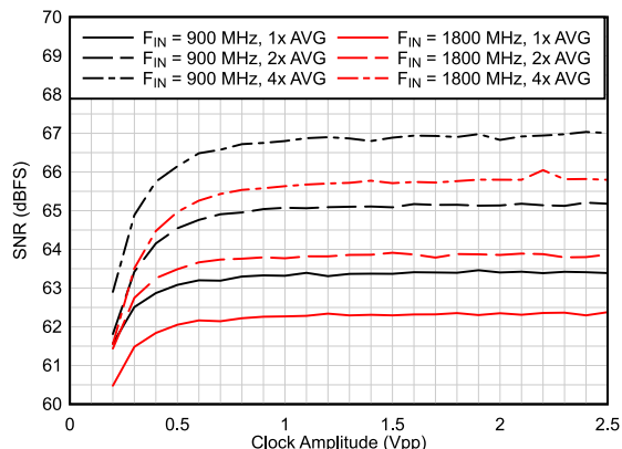
图 7-12. SNR vs Clock Amplitude (Dither OFF)
