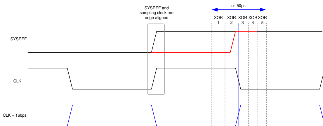
图 7-17. Detection of SYSREF Transition Within Capture Window
