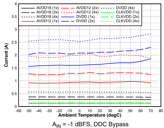
图 6-113. Current vs Temperature
