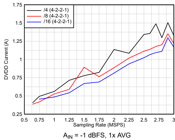
图 6-102. Current vs Sampling Rate vs Real Decimation
