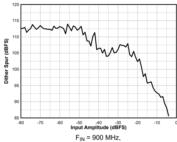
图 6-84. Dither Spur vs A_{IN}
