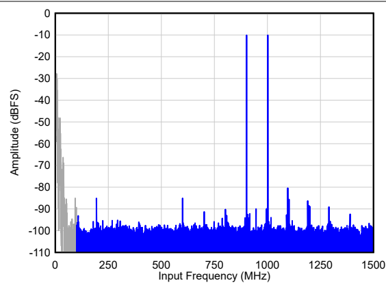
IMD3 = 70 dBc A_{IN} = -10 dBFS/tone, 1x AVG, Dither = EN 图 6-79. Two Tone FFT at F_{IN} = 900/1000 MHz
