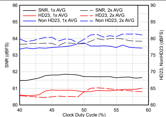
图 6-95. AC Performance vs Clock Duty Cycle
