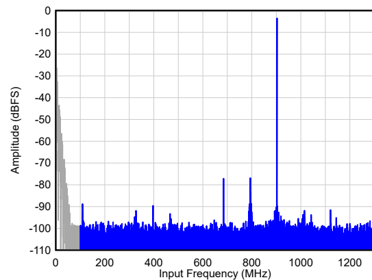
图 6-12. Single Tone FFT at F_{IN} = 2200 MHz
