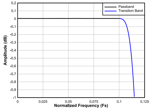
图 7-25. Decimation by 4 Passband Ripple Response
