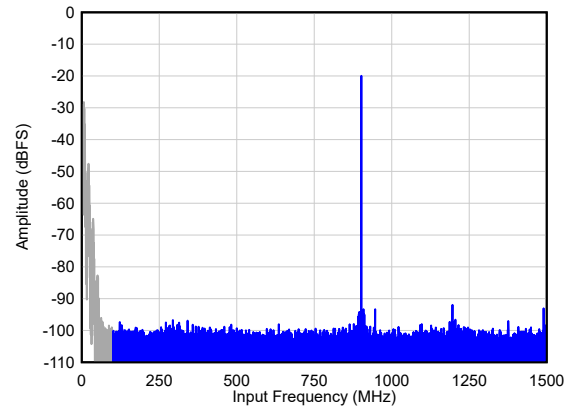
图 6-73. Single Tone FFT at F_{IN} = 900 MHz
