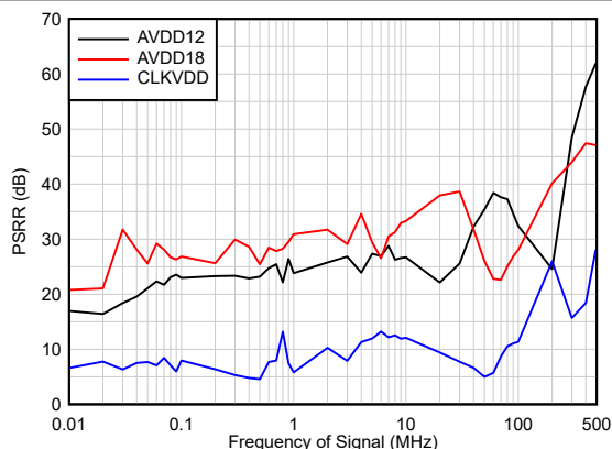
图 8-5. Power Supply Rejection Ratio (PSRR) vs Frequency
