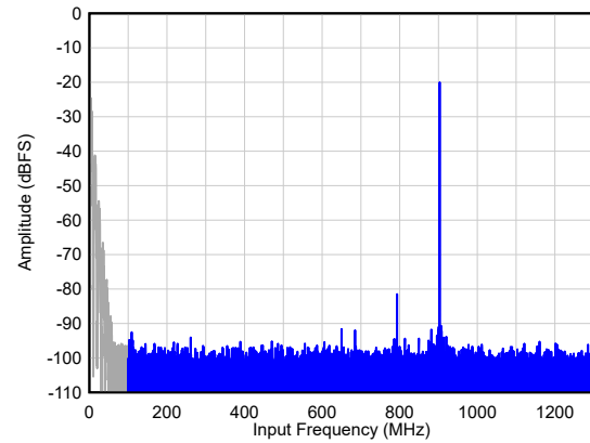
图 6-18. Single Tone FFT at F_{IN} = 900 MHz
