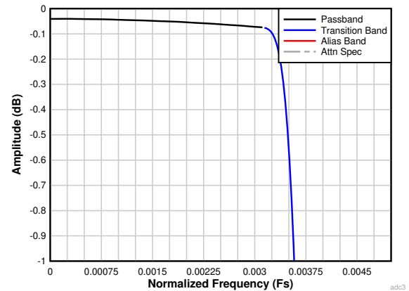
图 7-37. Decimation by 128 Passband Ripple Response
