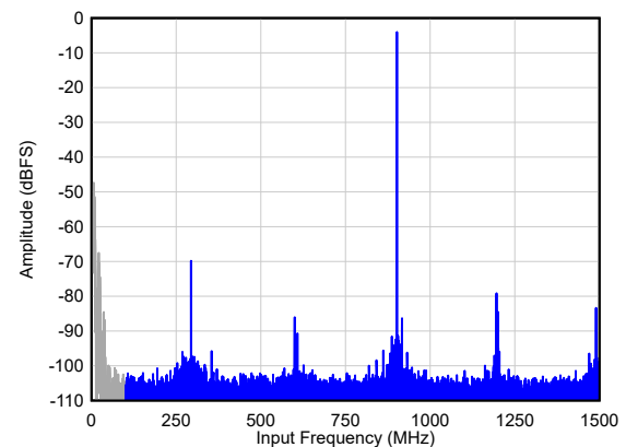
图 6-69. Single Tone FFT at F_{IN} = 900 MHz
