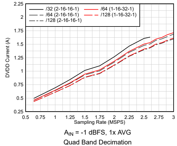
图 6-109. Current vs Sampling Rate vs Complex Decimation
