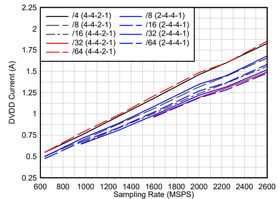
图 6-48. Current vs Sampling Rate vs Decimation
