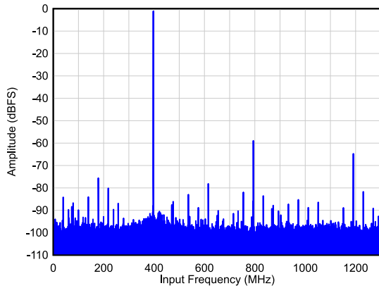
图 6-11. Single Tone FFT at F_{IN} = 2200 MHz
