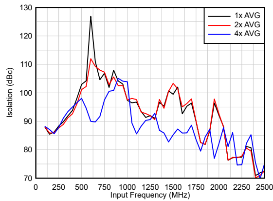
图 6-96. Isolation vs Input Frequency
