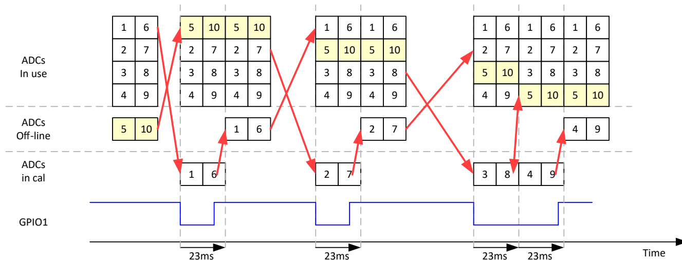
图 7-19. Timing Diagram - Calibration (4x AVG Example)
