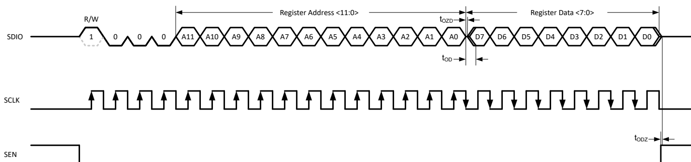
图 7-47. Serial Register Read Timing Diagram
