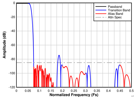
图 7-26. Complex Decimation by 8 Filter Response
