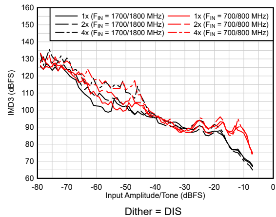
图 6-88. IMD3 Performance vs A_{IN}
