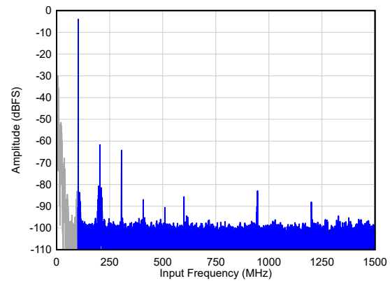
图 6-57. Single Tone FFT at F_{IN} = 100 MHz
