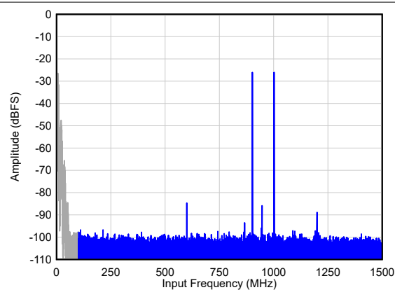
IMD3 = 71 dBc A_{IN} = -26 dBFS/tone, 1x AVG, Dither = EN 图 6-81. Two Tone FFT at F_{IN} = 900/1000 MHz
