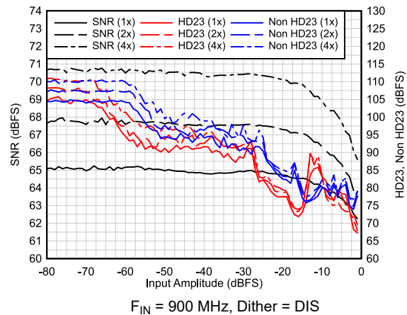
图 6-32. AC Performance vs A_{IN}
