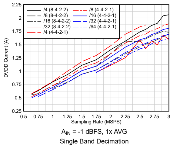
图 6-104. Current vs Sampling Rate vs Complex Decimation
