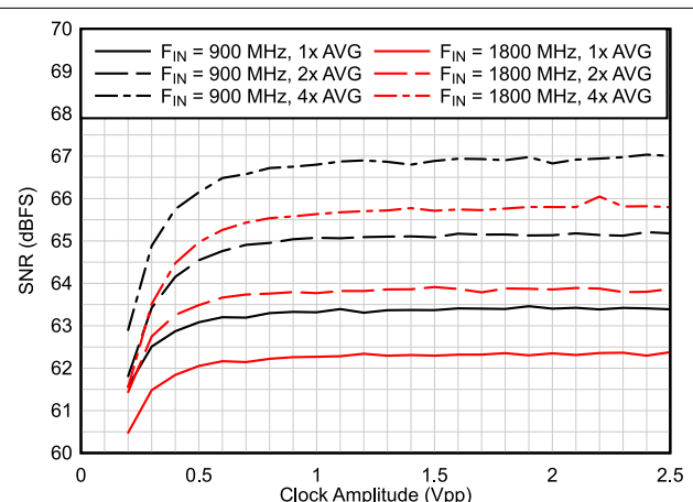
图 8-3. SNR vs Clock Amplitude (dither off)
