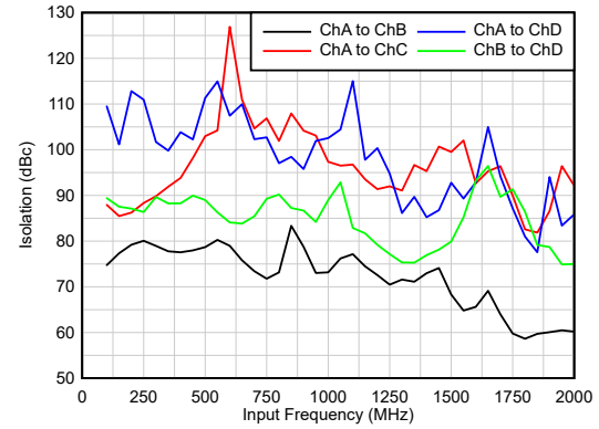
图 6-38. Isolation vs Input Frequency
