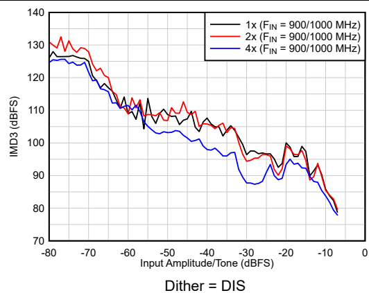
图 6-36. IMD3 Performance vs A_{IN}
