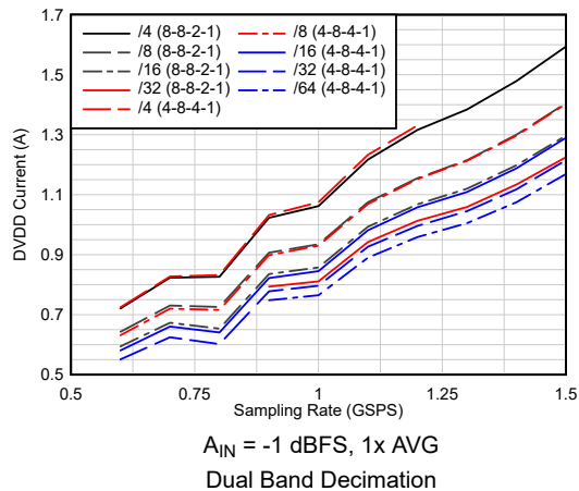
图 6-53. Current vs Sampling Rate vs Complex Decimation
