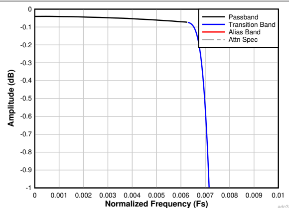
图 7-31. Decimation by 64 Passband Ripple Response
