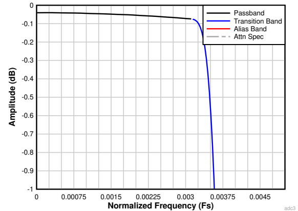
图 7-34. Decimation by 128 Passband Ripple Response
