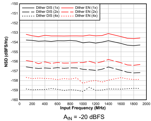
图 6-32. NSD Performance vs F_{IN}
