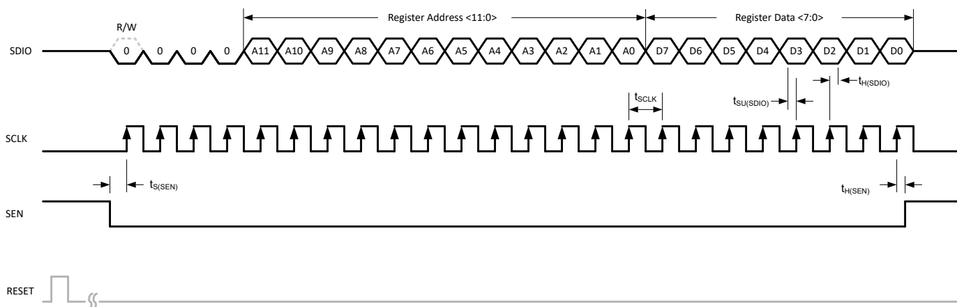
图 7-43. Serial Register Write Timing Diagram
