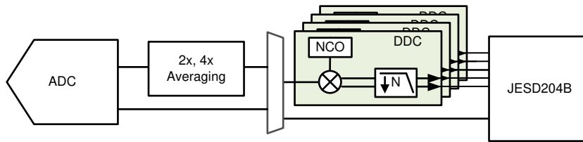
图 7-20. Digital Decimation Filter Options
