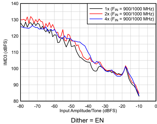
图 6-37. IMD3 Performance vs A_{IN}
