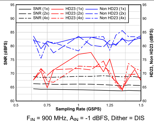
图 6-35. AC Performance vs F_S
