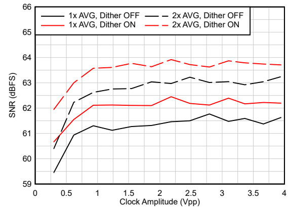
图 7-10. SNR vs Clock Amplitude ( F_{IN} = 1800 \text{ MHz} )
