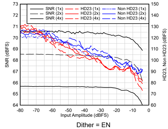
图 6-34. AC Performance vs A_{IN}
