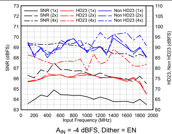
图 6-30. AC Performance vs F_{IN}
