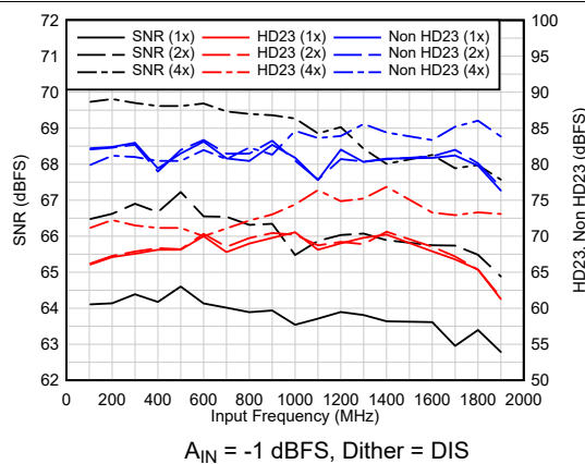
图 6-29. AC Performance vs F_{IN}
