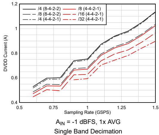
图 6-51. Current vs Sampling Rate vs Complex Decimation
