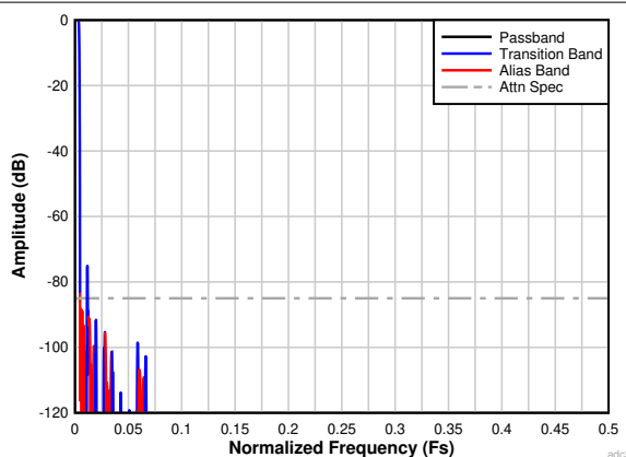
图 7-32. Complex Decimation by 128 Filter Response
