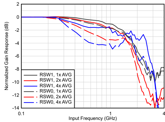
图 7-2. Full power input bandwidth
