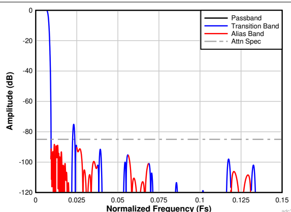
图 7-30. Complex Decimation by 64 Filter Response
