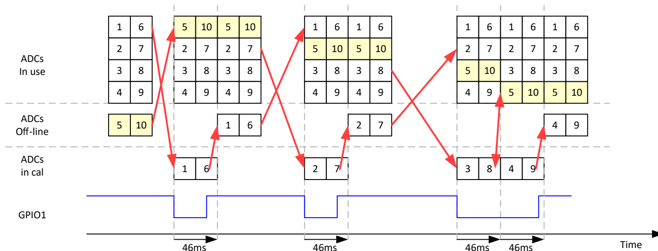
图 7-16. Timing diagram - calibration (4x AVG example)
