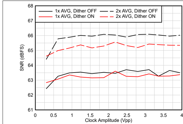
图 7-9. SNR vs Clock Amplitude ( F_{IN} = 900 \text{ MHz} )
