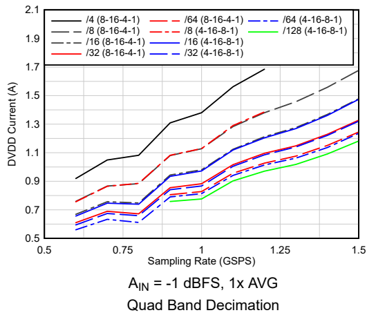
图 6-55. Current vs Sampling Rate vs Complex Decimation
