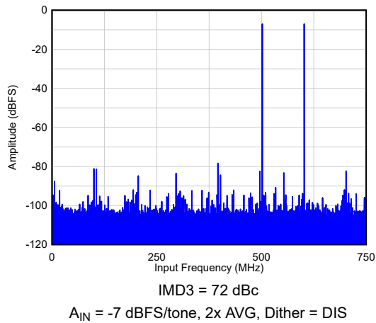
图 6-25. Two Tone FFT at F_{IN} = 900, 1000\text{ MHz}
