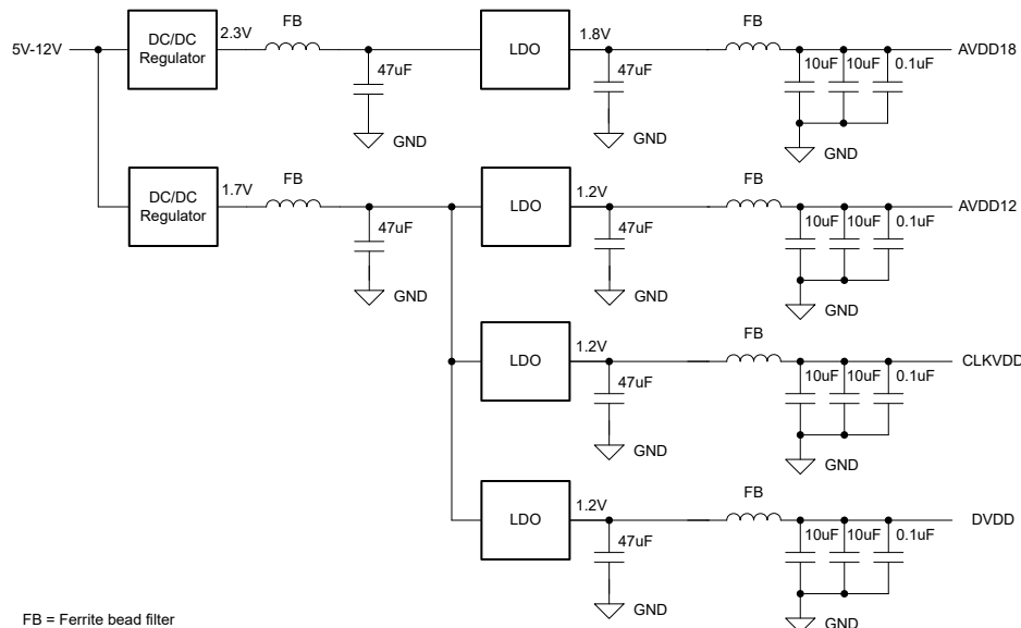
图 8-6. Power supply design example
