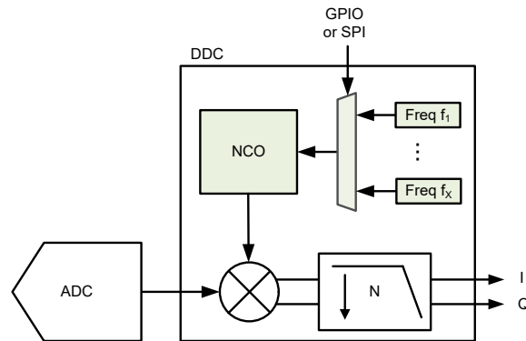
图 7-35. NCO Block Diagram
