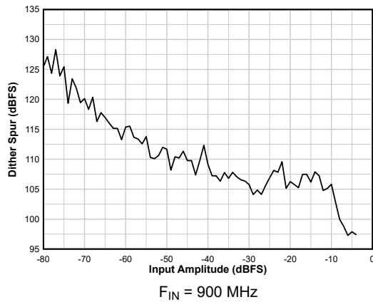
图 6-31. Dither Spur vs A_{IN}
