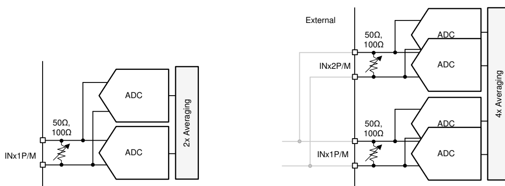
图 7-42. Internal digital averaging (left: 2x, right: 4x)
