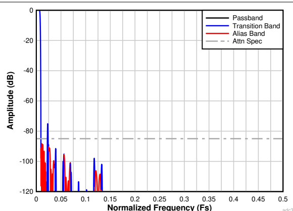
图 7-29. Complex Decimation by 64 Filter Response
