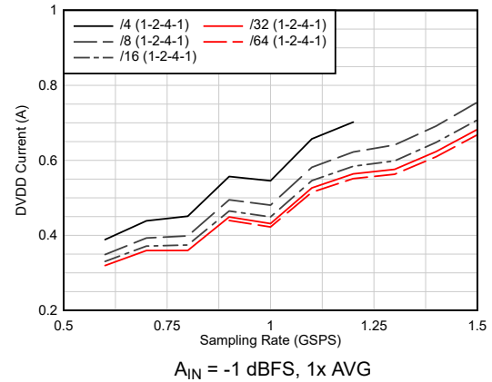
图 6-50. Current vs Sampling Rate vs Real Decimation
