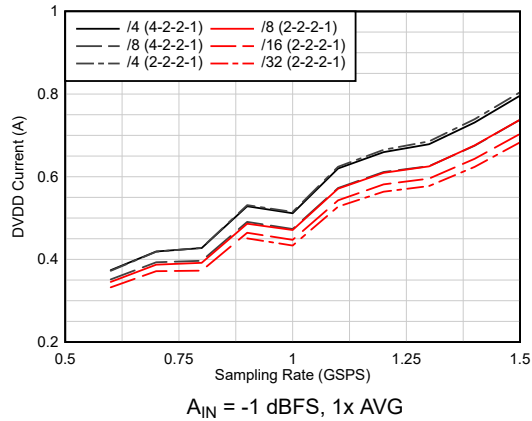
图 6-49. Current vs Sampling Rate vs Real Decimation
