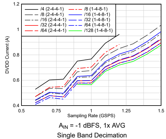
图 6-52. Current vs Sampling Rate vs Complex Decimation
