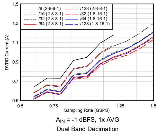
图 6-54. Current vs Sampling Rate vs Complex Decimation
