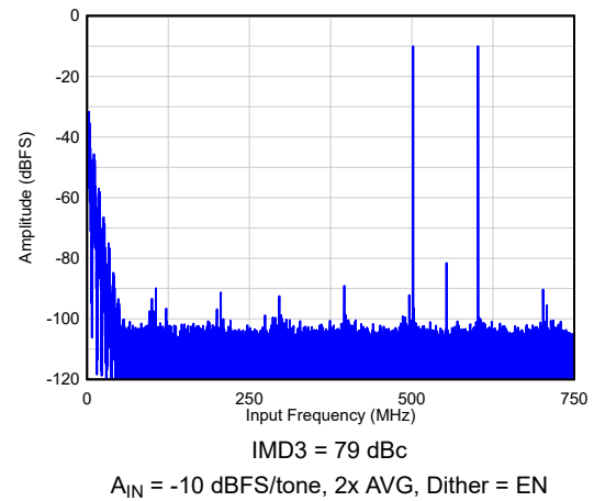
图 6-26. Two Tone FFT at F_{IN} = 900, 1000\text{ MHz}
