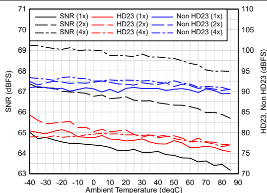
图 6-43. AC Performance vs Temperature
