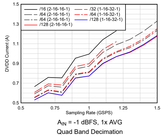
图 6-56. Current vs Sampling Rate vs Complex Decimation
