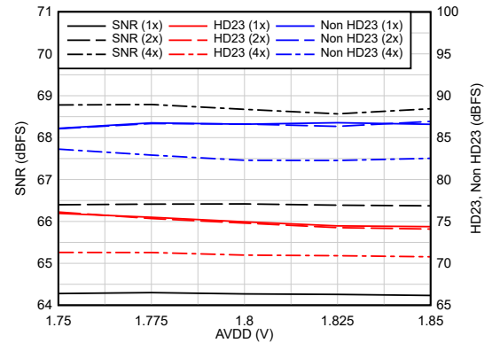
图 6-40. AC Performance vs \text{AVDD18}
