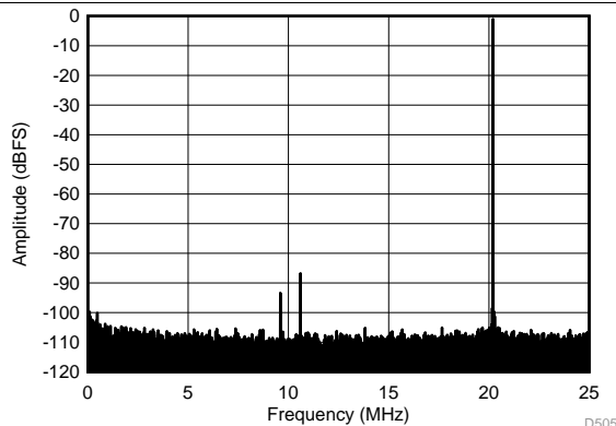
SFDR = 85.8 dBc, SFDR = 99.1 dBc (non 23), SNR = 72.4 dBFS, SINAD = 72.2 dBFS, THD = 84.8 dBc, HD2 = -92.3 dBc, HD3 = -85.8 dBc
