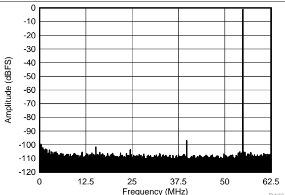
Figure 96. FFT for 70-MHz Input Signal (Dither On) SFDR = 95.9 dBc, SNR = 72.7 dBFS, SINAD = 72.7 dBFS, THD = 93.6 dBc, HD2 = -100.6 dBc, HD3 = -95.9 dBc
