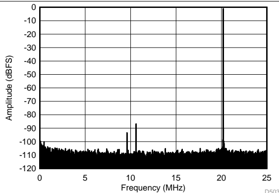
SFDR = 85.8 dBc, SFDR = 100.3 dBc (non 23), SNR = 72.4 dBFS, SINAD = 72.2 dBFS, THD = 84.8 dBc, HD2 = -92.3 dBc, HD3 = -85.8 dBc
