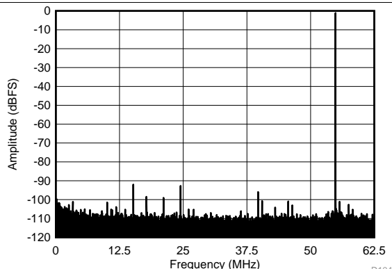
Figure 97. FFT for 70-MHz Input Signal (Dither Off) SFDR = 90.9 dBc, SNR = 73.3 dBFS, SINAD = 73.1 dBFS, THD = 87 dBc, HD2 = -90.9 dBc, HD3 = -94.9 dBc
