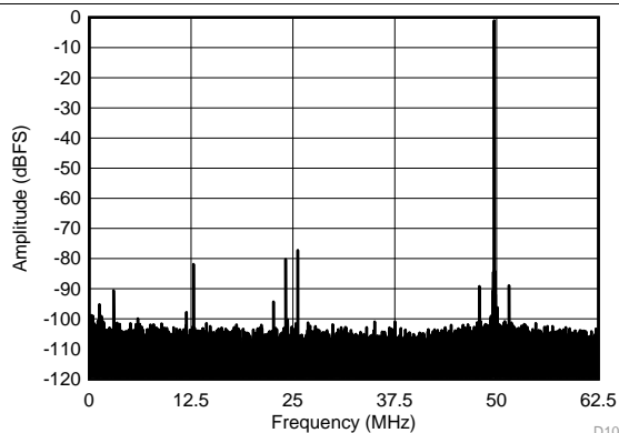
SFDR = 76.2 dBc, SNR = 68.8 dBFS, SINAD = 67.5 dBFS, THD = 74.3 dBc, HD2 = -76.2\text{ dBc} , HD3 = -79.2\text{ dBc}
