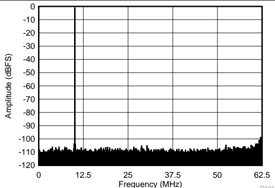
Figure 94. FFT for 10-MHz Input Signal (Chopper On, Dither On) SFDR = 102.6 dBc, SNR = 72.9 dBFS, SINAD = 72.8 dBFS, THD = 99.8 dBc, HD2 = -108.6 dBc, HD3 = -104.0 dBc
