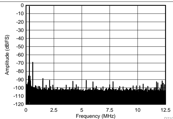
SFDR = 67.9 dBc, SNR = 67.2 dBFS, SINAD = 67.2 dBFS, THD = 87.6 dBc, HD2 = -67.9 dBc, HD3 = -96.9 dBc
