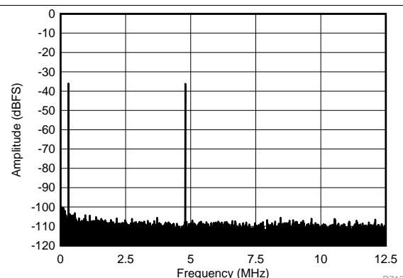
f_{IN1} = 46 \text{ MHz} , f_{IN2} = 50 \text{ MHz} , IMD3 = 90 dBFS, each tone at -36 dBFS
