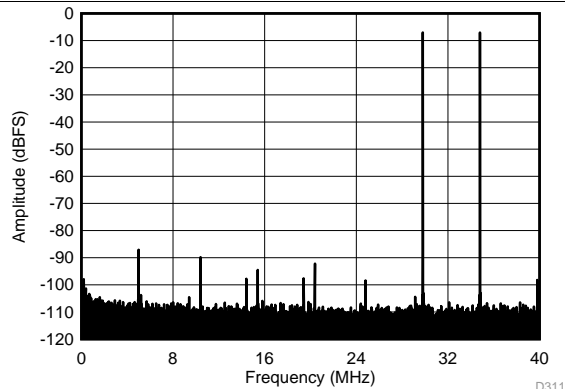
Figure 73. FFT for Two-Tone Input Signal (-7 dBFS at 46 MHz and 50 MHz)
