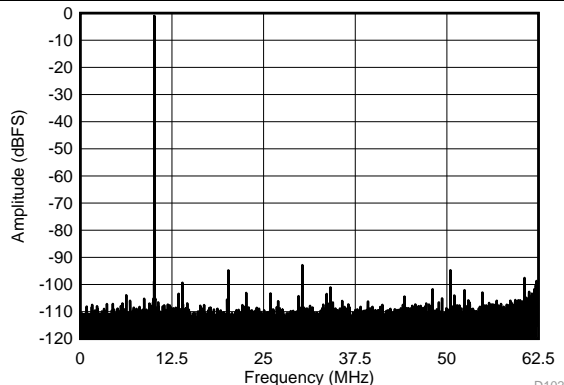
Figure 95. FFT for 10-MHz Input Signal (Chopper On, Dither Off) SFDR = 91.8 dBc, SNR = 73.5 dBFS, SINAD = 73.4 dBFS, THD = 87.3 dBc, HD2 = -93.8 dBc, HD3 = -91.8 dBc
