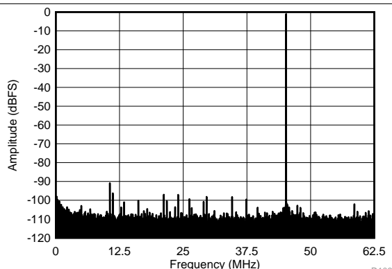
Figure 99. FFT for 170-MHz Input Signal (Dither Off) SFDR = 89.9 dBc, SNR = 72.8 dBFS, SINAD = 72.6 dBFS, THD = 87.1 dBc, HD2 = -97.2 dBc, HD3 = -89.9 dBc
