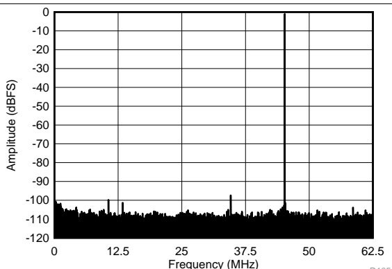
Figure 98. FFT for 170-MHz Input Signal (Dither On) SFDR = 96.4 dBc, SNR = 72.1 dBFS, SINAD = 72.0 dBFS, THD = 92.6 dBc, HD2 = -96.4 dBc, HD3 = -98.8 dBc
