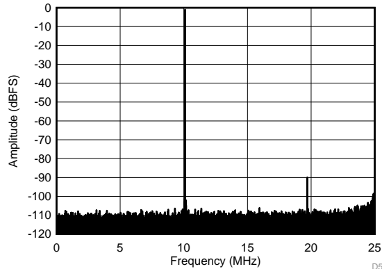
SFDR = 88.9 dBc, SFDR = 99.8 dBc (non 23), SNR = 73.6 dBFS, SINAD = 73.5 dBFS, THD = 88.8 dBc, HD2 = -111.4 dBc, HD3 = -88.9 dBc
