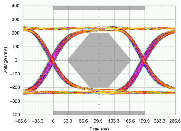
5-mil. FR4 Microstrip Trace at 5 Gb/s with No De-Emphasis
