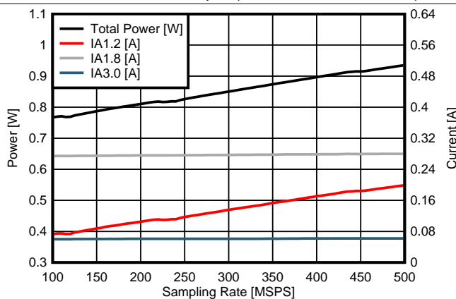
图 23. Supply Power and Current vs Sampling Rate
