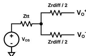
图 29. Electrical Circuit Diagram for Differential Output Signals
