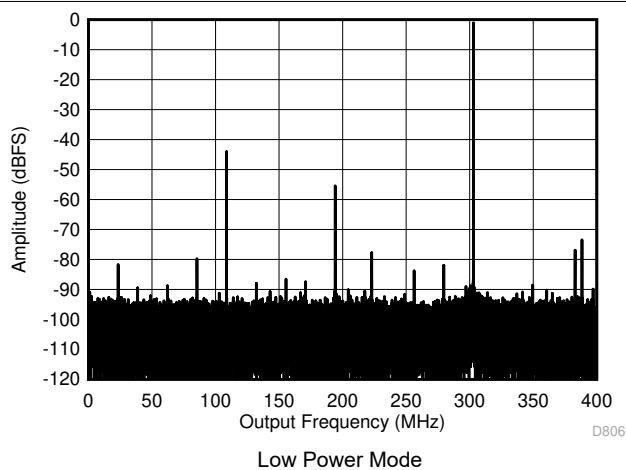
图 5-12. Single Tone FFT at 2097 MHz and -1dBFS
