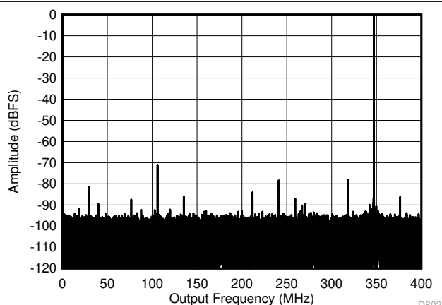
图 5-8. Single Tone FFT at 2097 MHz and -1dBFS
